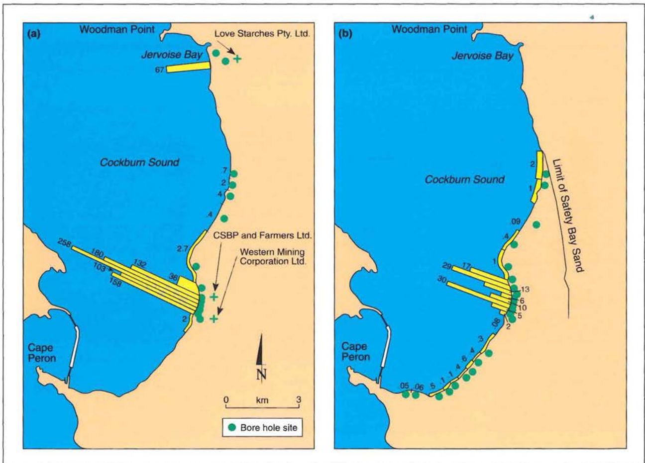
Figure 4. Groundwater nitrogen loads into Cockburn Sound from (a) the Tamala Limestone and (b) the Safety Bay Sand. Loads are in tonnes of nitrogen per kilometre of coastline per year.
