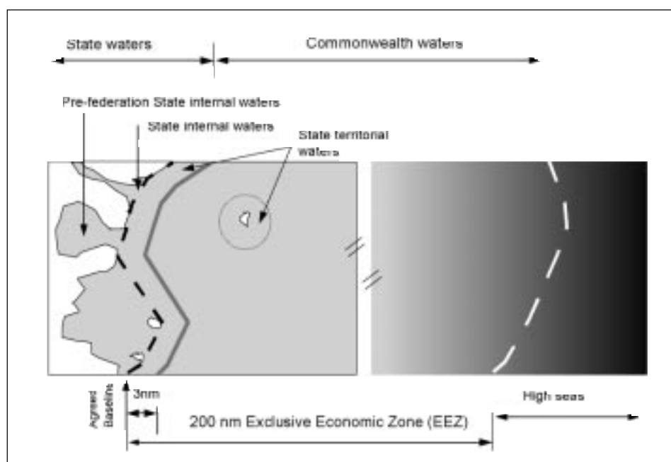
Figure 2: Schematic map of Australia's coastal and marine realm including State and Commonwealth waters (nm = nautical mile).
