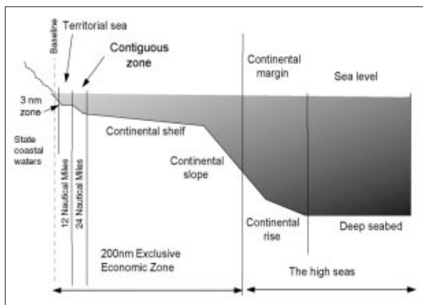
Figure 1: Schematic profile of the various zones including the 200 n mile Exclusive Economic Zone and the high seas (nm = nautical mile).
