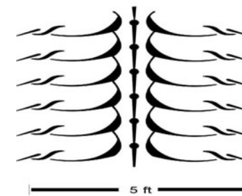
Figure 2-7. Leatherback track
