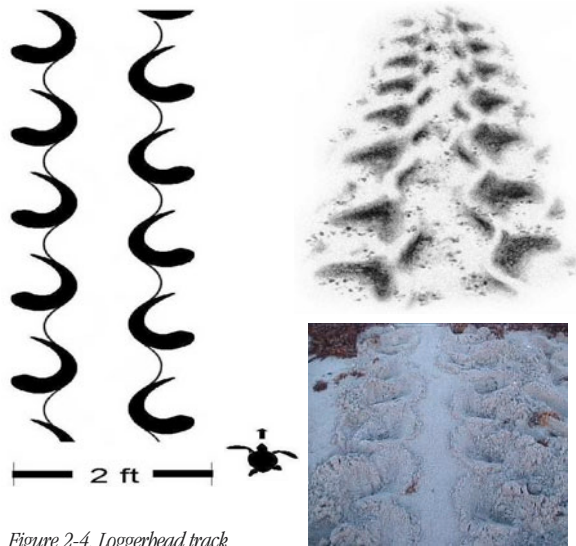
Figure 2-4. Loggerhead track
