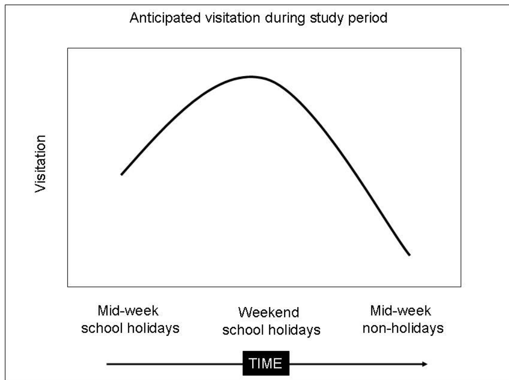
Figure 7: Anticipated changes in relative visitation levels over the course of the study period, with moderate visitation during the mid-week school holiday period, high visitation during with weekend school holiday period and low visitation during the mid-week non-holiday period
