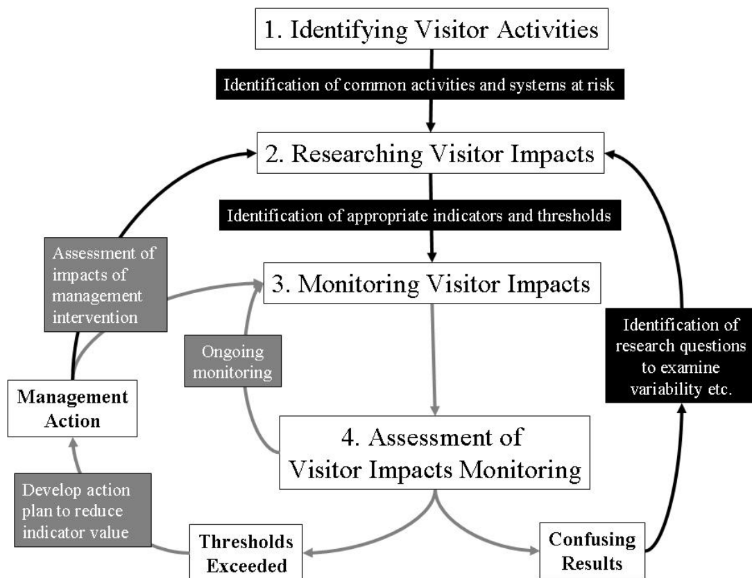
Figure 9: Visitor impact assessment flow chart. Conceptual flow diagram showing the links and differences between visitor impacts research and visitor impacts monitoring in protected areas. (Black arrows represent components of the process likely to be undertaken by research scientists, grey arrows represent the components of the process likely to be undertaken by protected area agency staff.). Figure modified from Hadwen et al. (2008b)
