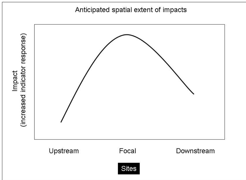
Figure 8: Anticipated spatial extent of impacts (indicator response), with highest response at focal sites, some downstream effects (moderate response at downstream control sites) and no response at upstream control sites
