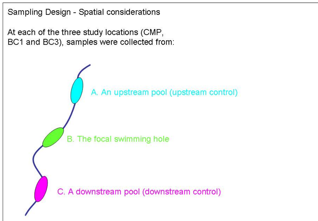
Figure 5: Graphical representation of the spatial design of the monitoring program, with upstream, focal and downstream sites
