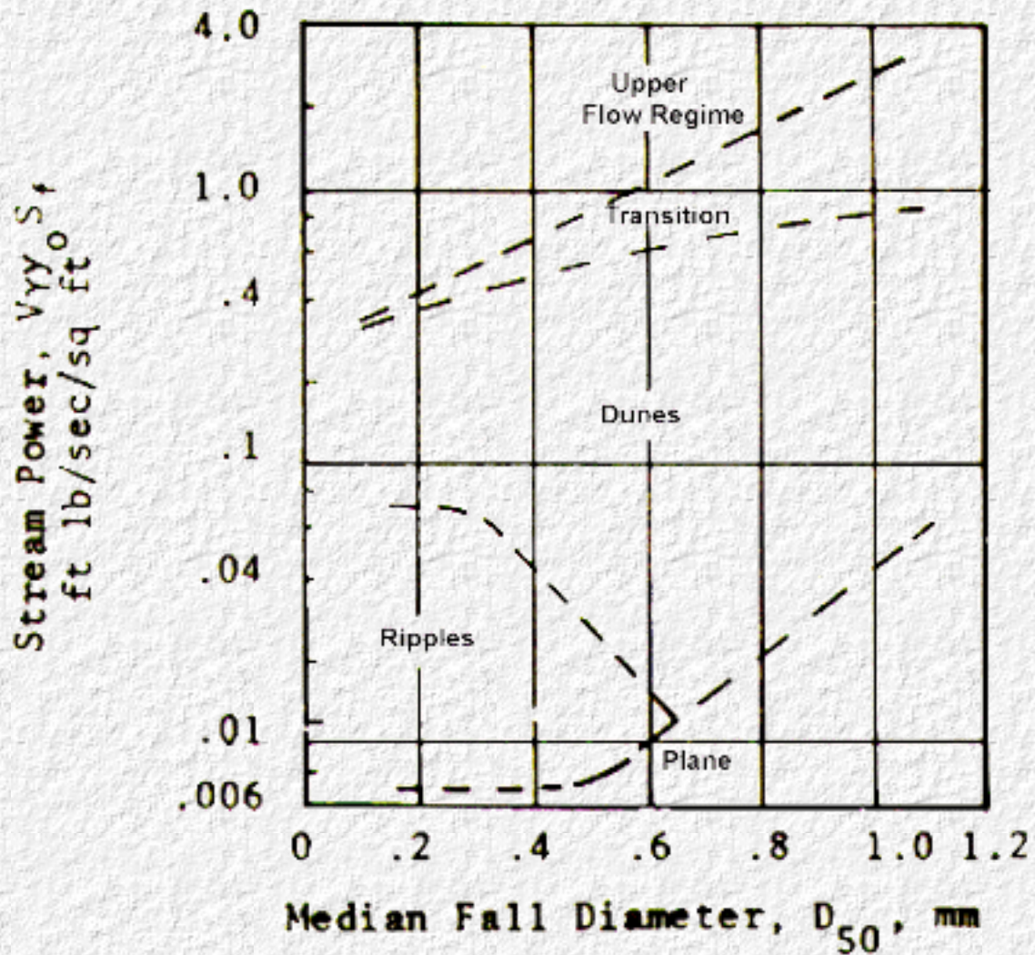
Figure 2. Relation of Stream Power and Median Grain Size to Flow Regime (from HIRE, Fig 3.4.4)
