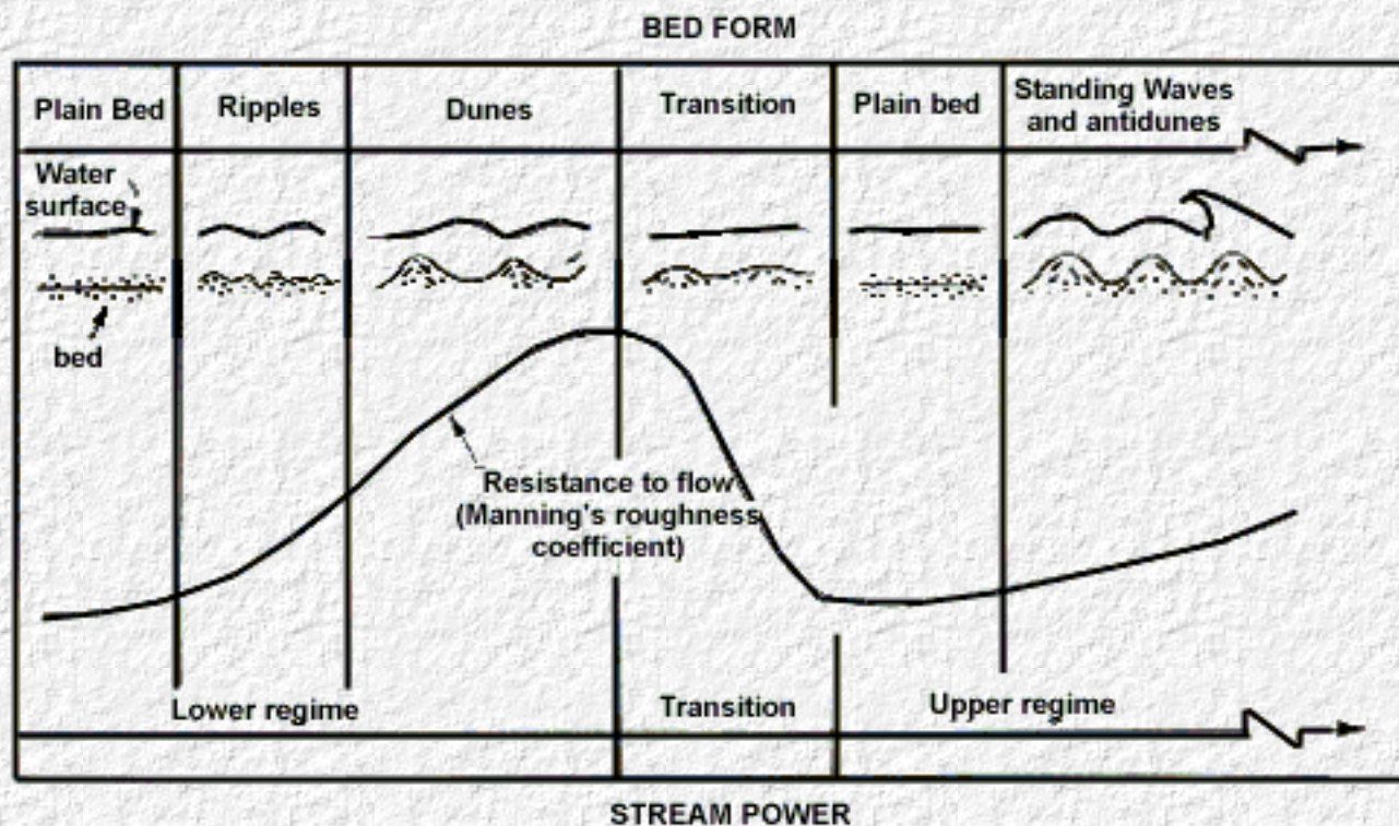
Figure 3. Forms and Bed Roughness in Sand-Bed Channels
