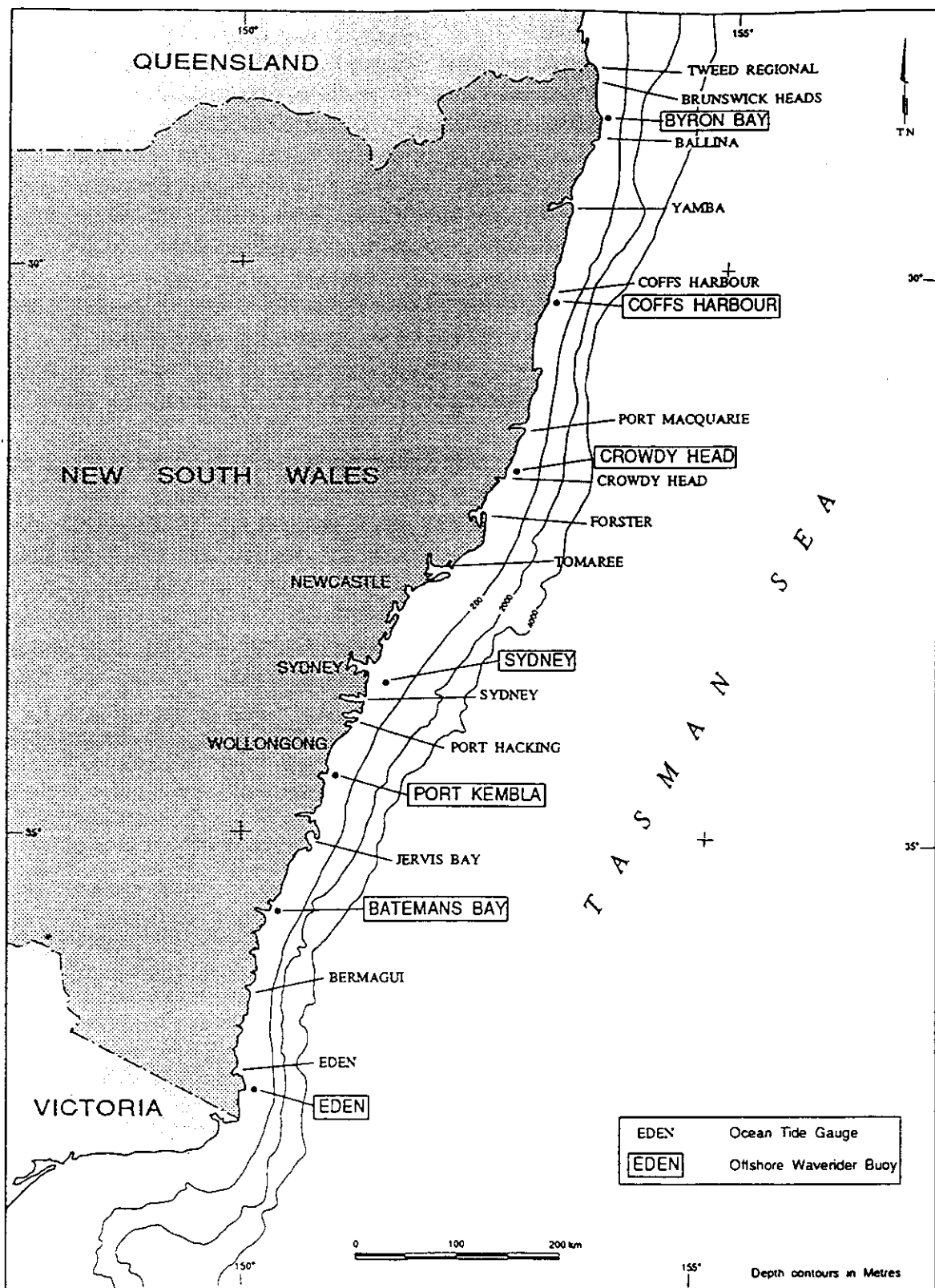
Fig. 3.2.1 New South Wales Public Works Department real-time wave-rider buoy locations 1995 (see Manly Hydraulics Laboratory report 733).
