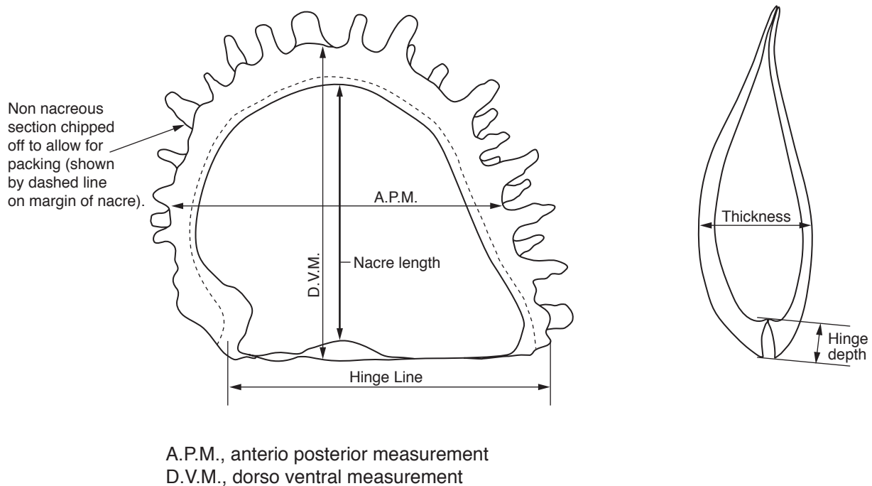
Figure 6. Morphometric measurements commonly used to measure the morphology of Pinctada maxima . DVM is the principal measure of growth.
