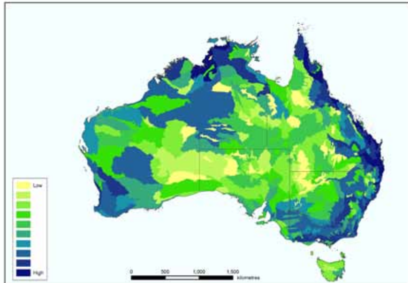
Figure 6 Species richness in Australia's bioregions
