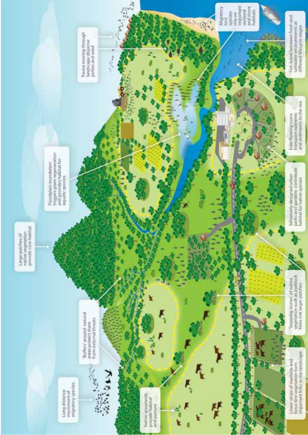
Figure 2 Elements of connectivity within the landscape
