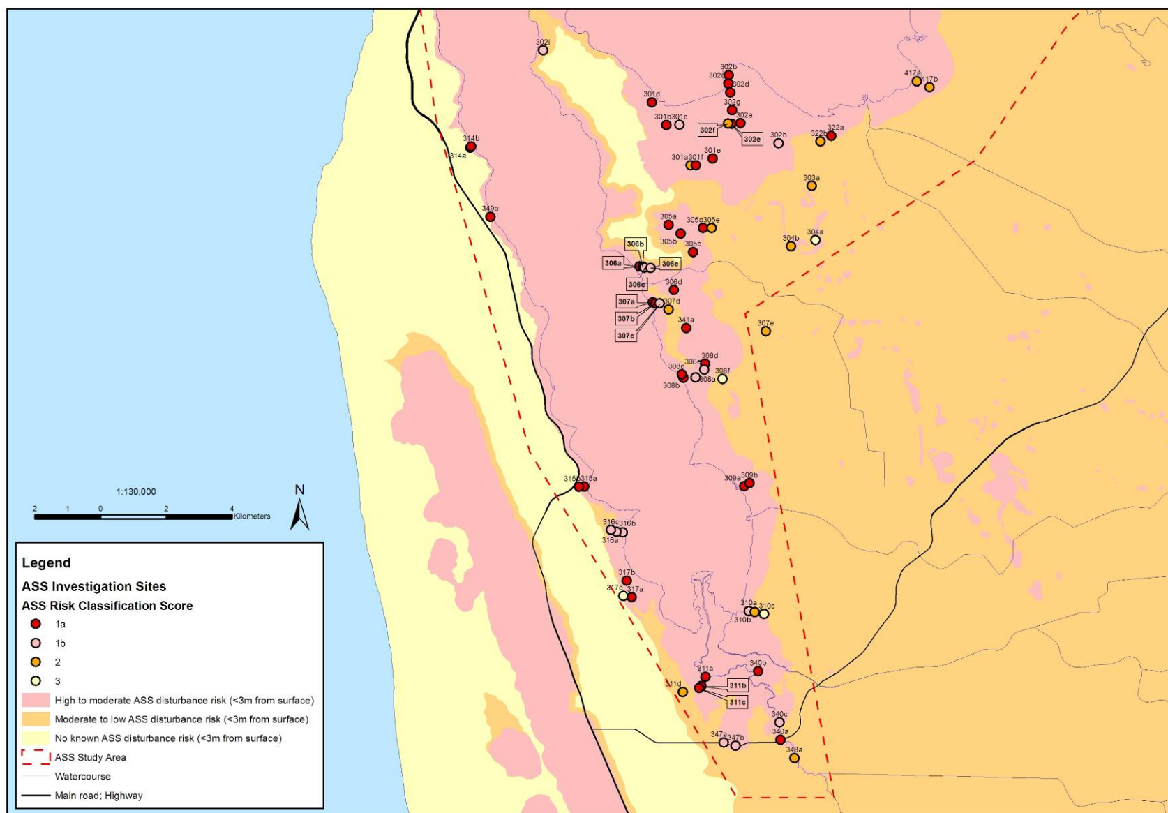
Figure 16: Mapping of high risk of potential Acid Sulfate Soil materials occurring within the superficial sediments (<3mbgl) surrounding the SE Peel Inlet, Harvey Inlet and Harvey Rive and classification of ASS disturbance risk for the superficial formations at various sites (see Appendix 2 for details on risk classification).
