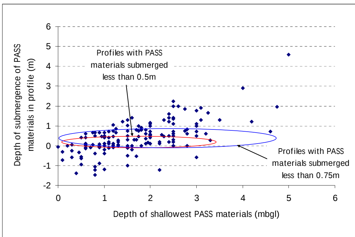
Figure 10: Plot of the depth at which shallowest PASS materials occurred in superficial sediment profiles (mbgl) in relation to the depth that the materials were submerged below the water-table (measured at the time of coring), for profiles where both PASS materials occurred and a water-table measurement was available (145 sites).
