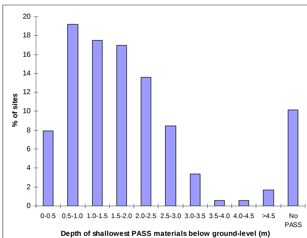
Figure 6: Distribution of sites classified by depth of shallowest PASS materials below ground-level.
