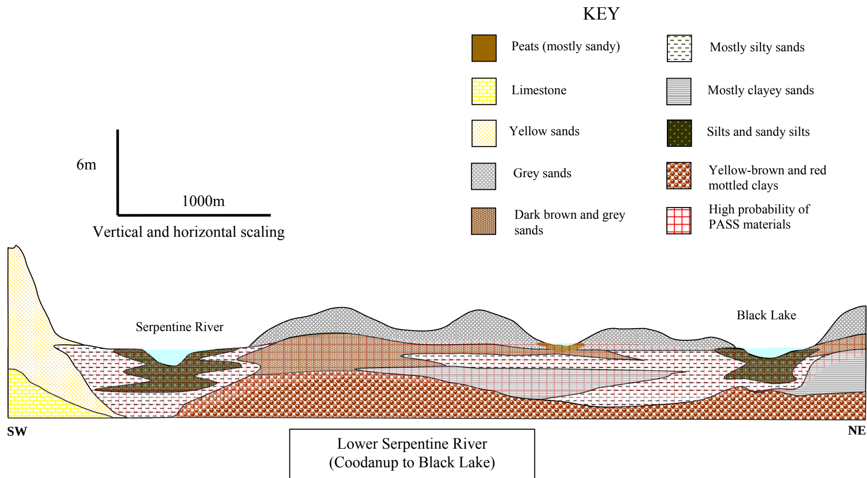
Figure 17: Schematic landscape cross-section illustrating occurrence of PASS materials in relation to landscape position and dominant lithology in the lower Serpentine River area (representing the landscape from Coodanup to Black Lake).
