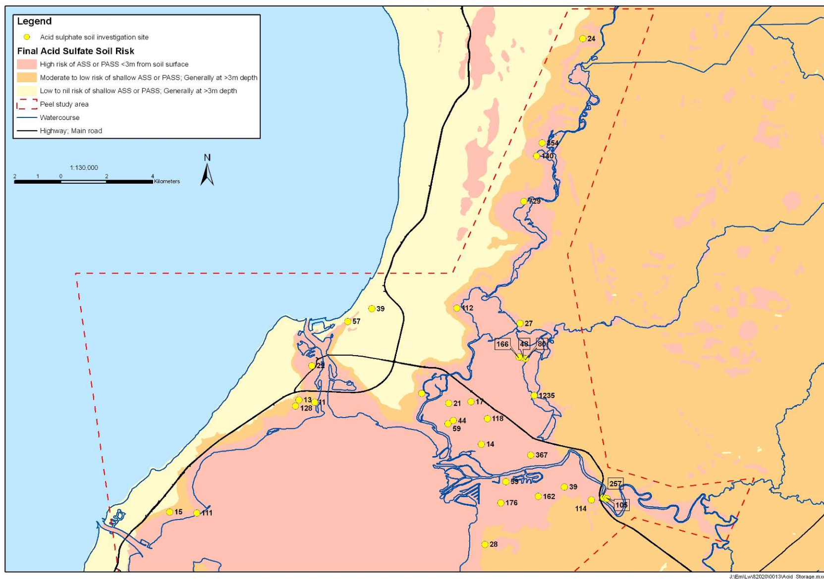
Figure 12: Estimated storage of potential acidity (tonnes H_2SO_4/ha ) within the surface 1m of shallow PASS materials encountered at Acid Sulfate Soil investigation sites in
