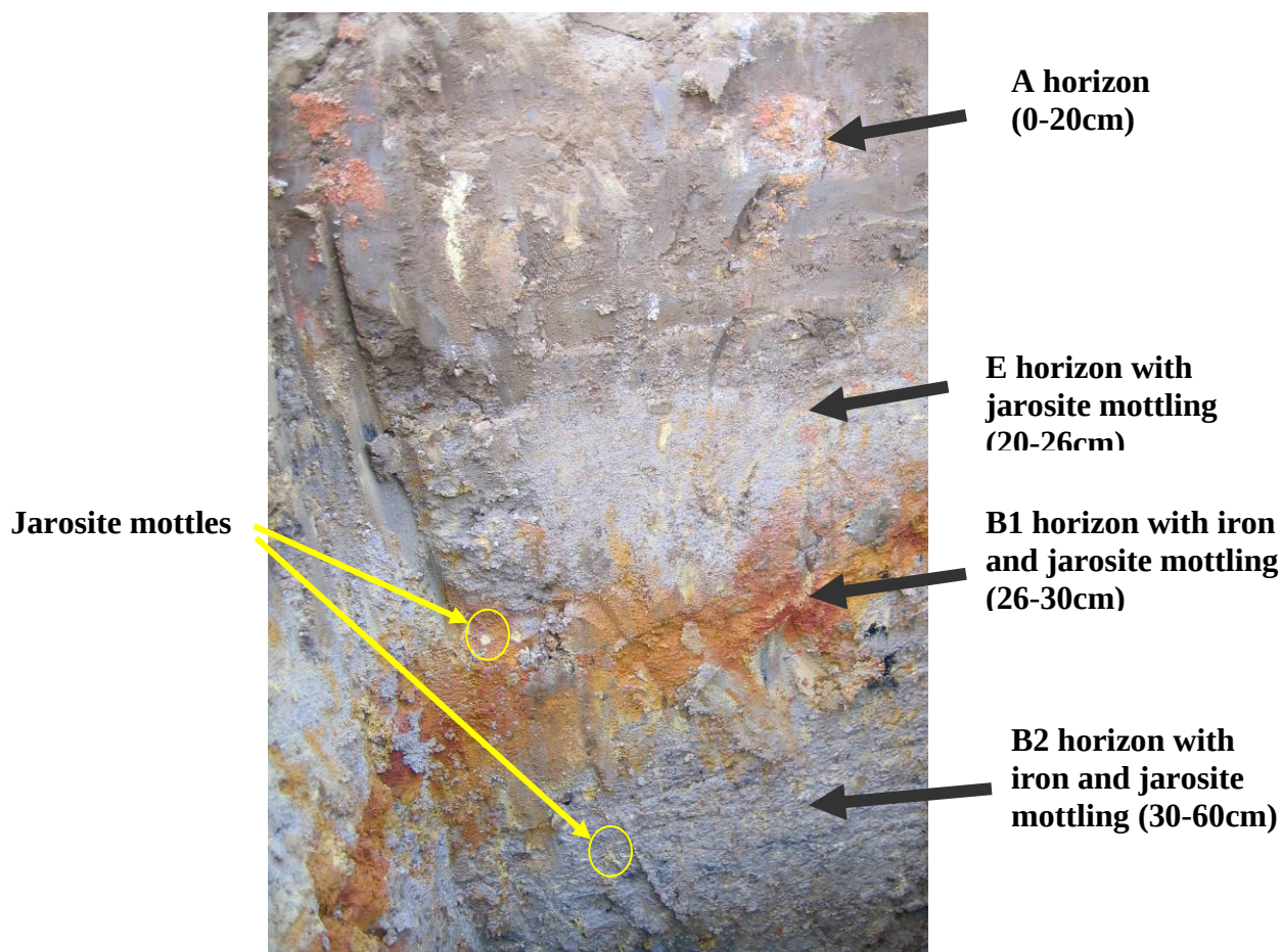
Figure 14: Jarosite evident as pale yellow mottling (Munsell Colour 2.5Y 8/3) within an actual ASS profile in South Yunderup site 411f
