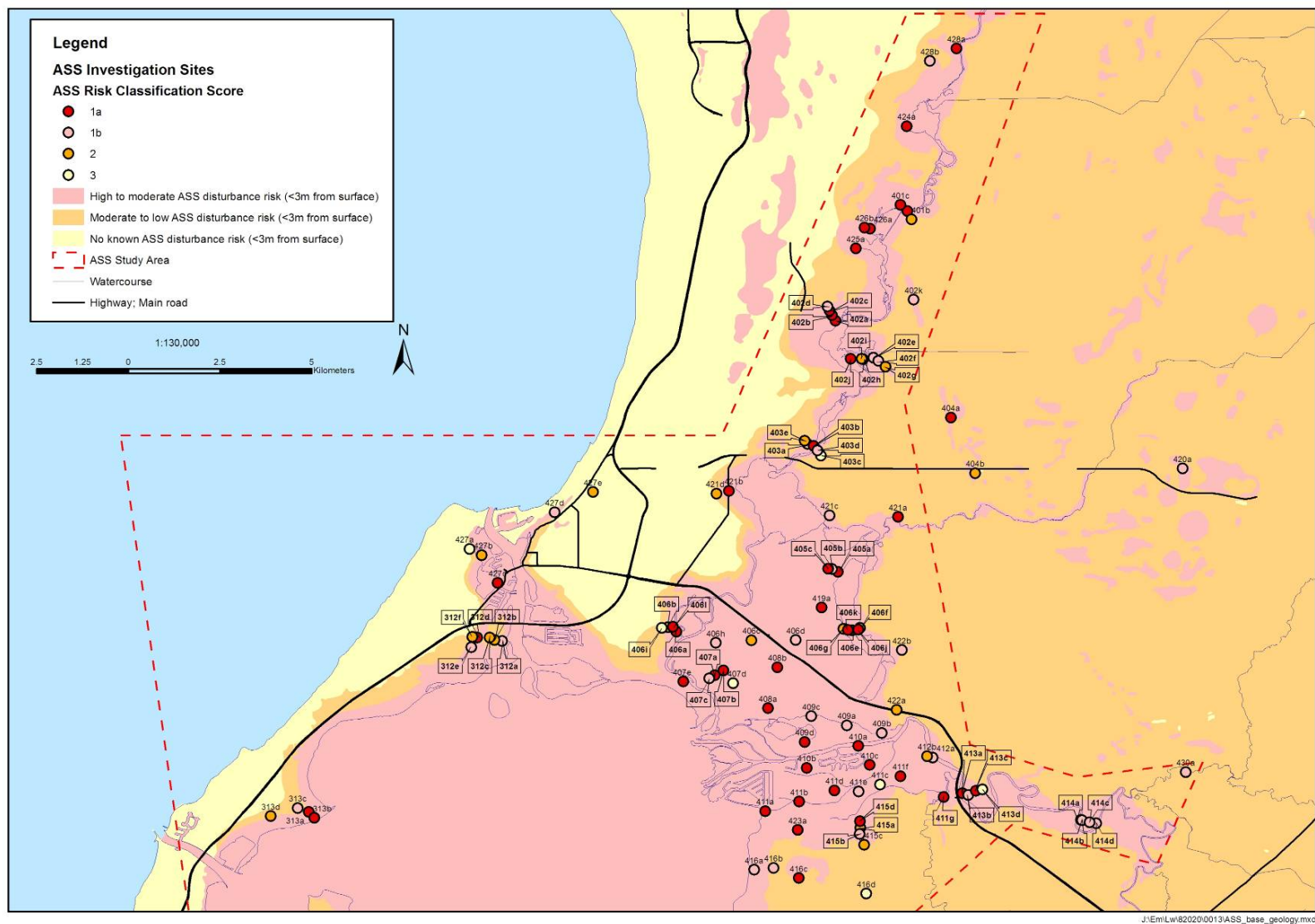
Figure 15: Mapping of high risk of potential Acid Sulfate Soil materials occurring within the superficial sediments (<3 mbgl) surrounding the Peel Inlet, Serpentine River and Murray River and classification of ASS disturbance risk for the superficial formations at various sites (see Appendix 2 for details on risk classification).
