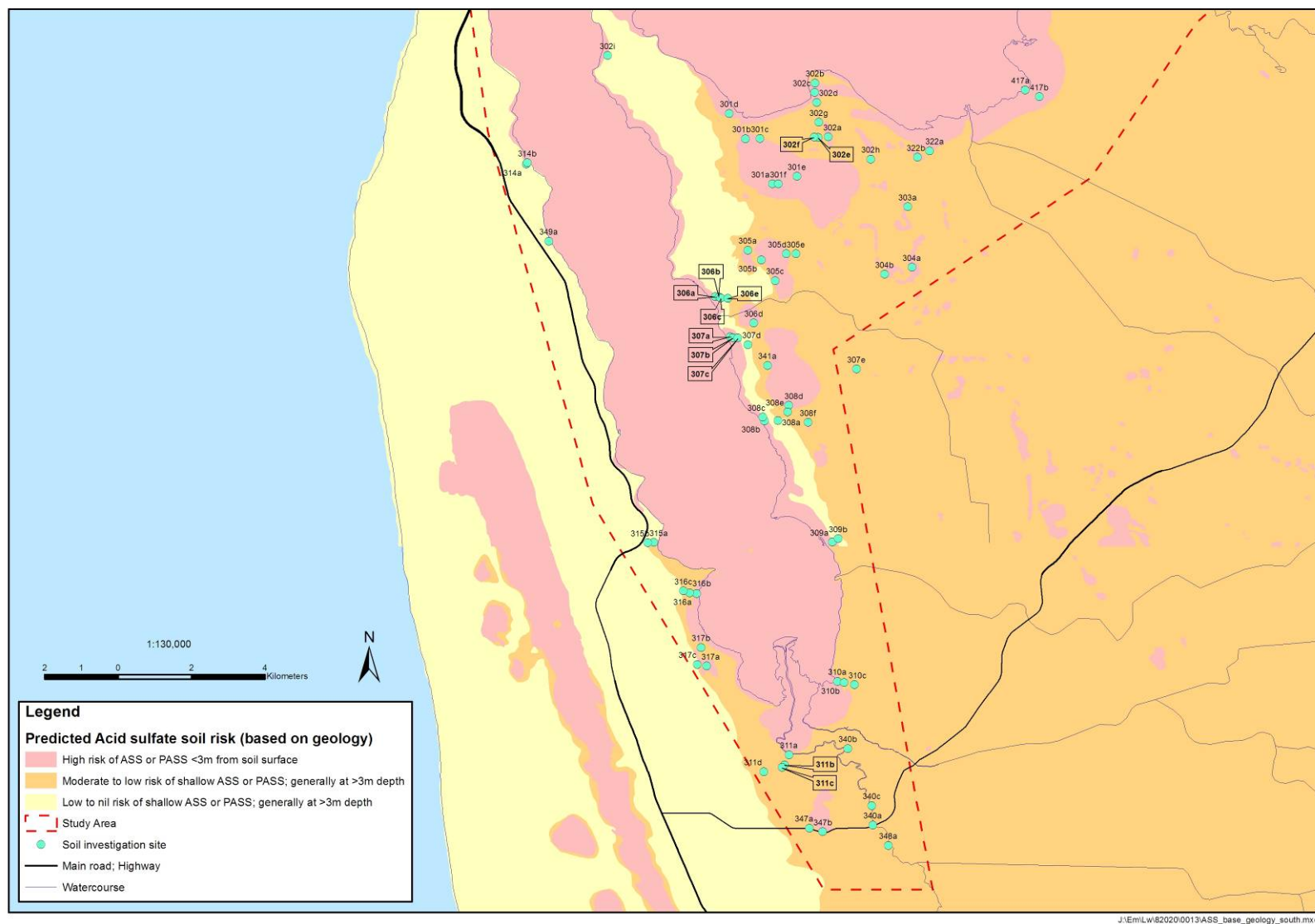
Figure 4: Initial ASS risk map (based on 1:50 000 scale environmental and urban geology mapping) and superficial formation investigation sites (SE Peel inlet, Harvey Inlet and Harvey River). Note: map not printed to scale.
