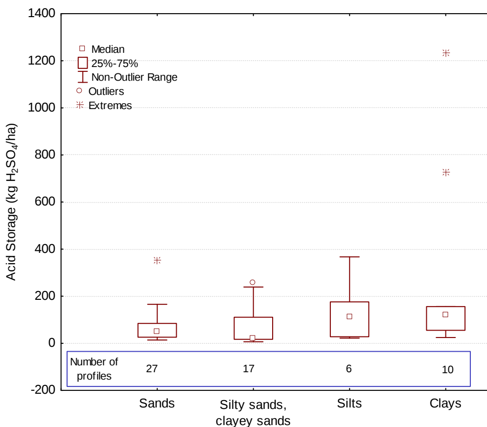
Figure 11: Estimation of acid storage within the shallowest PASS materials (up to 1 m thickness) categorised by the dominant textures in which the PASS materials occurred.
