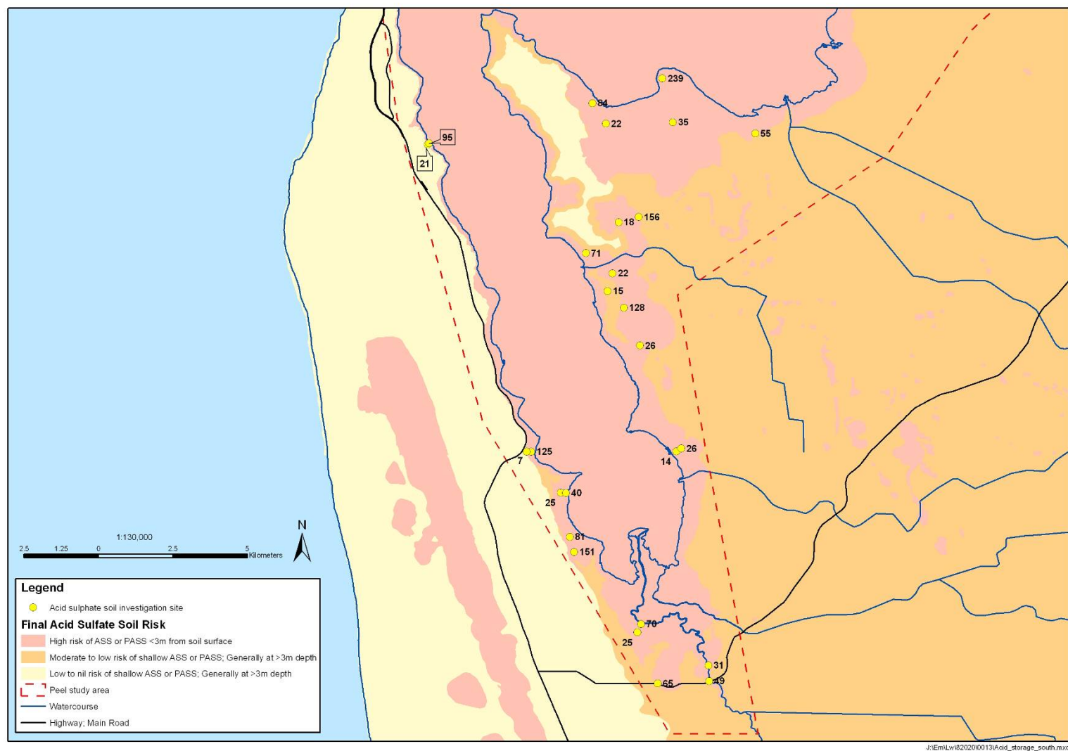
Figure 13: Estimated storage of potential acidity (tonnes H_2SO_4 /ha) within the surface 1 m of shallow PASS materials encountered at Acid Sulfate Soil investigation sites in superficial sediments around the SE Peel Inlet, Harvey Inlet and Harvey River. Note: map not displayed to scale.
