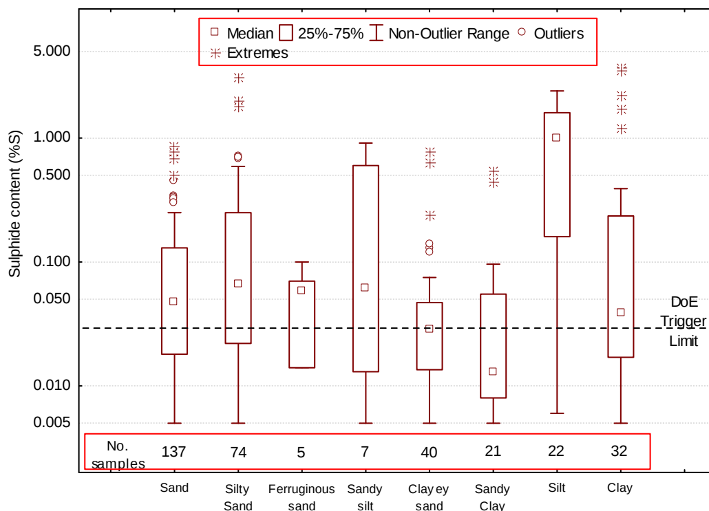
Figure 5: Concentrations of PASS materials (as indicated by % sulfide-S on a logarithmic scale) for representative samples of horizons (grouped by dominant soil texture).
