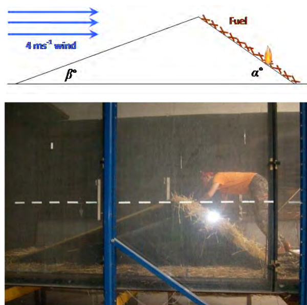
Figure 6. Schematic cross-section of the experimental ridge configuration and the approximate ignition point (top), and the actual combustion tunnel set-up (bottom).
