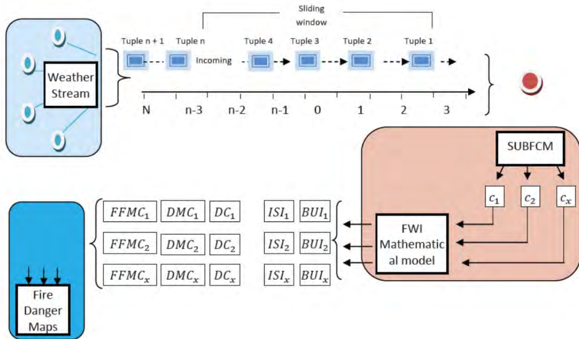
Figure 2: Distributed weather data stream mining flow diagram
