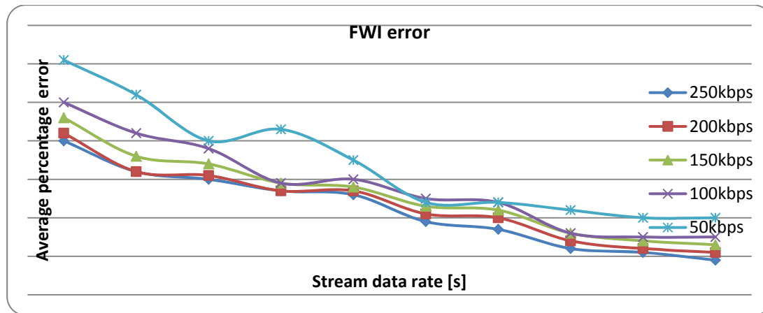
Figure 7: Average FWI error for different network data rates
