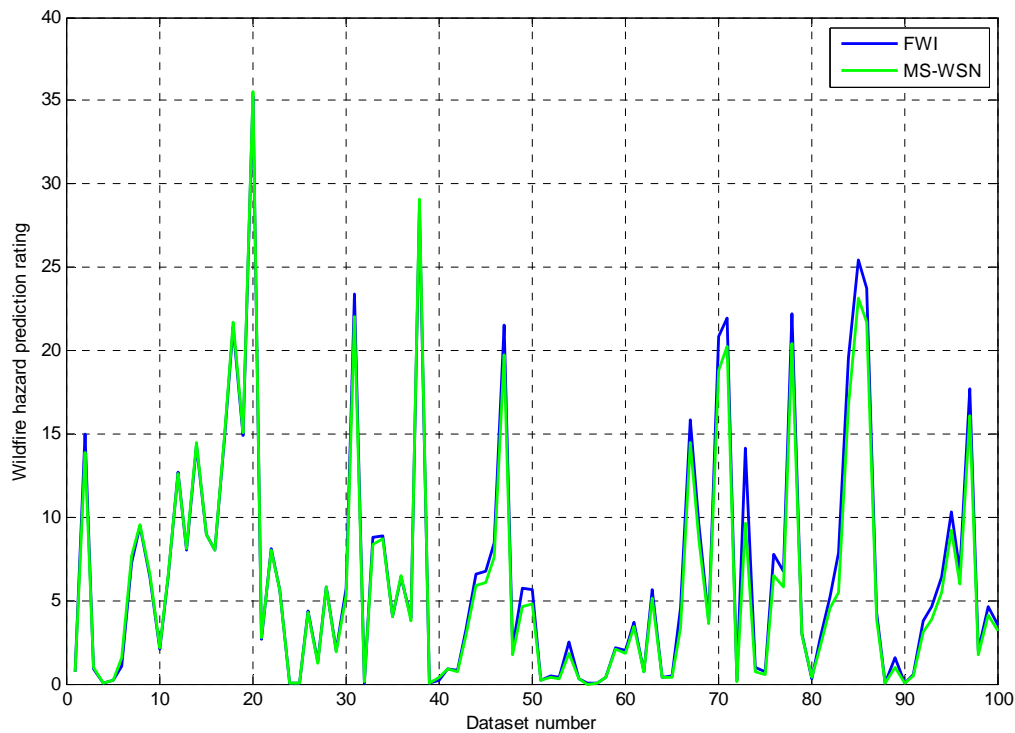
Figure 5: Comparison of Micro-scale FWI and FWI systems FWI index
