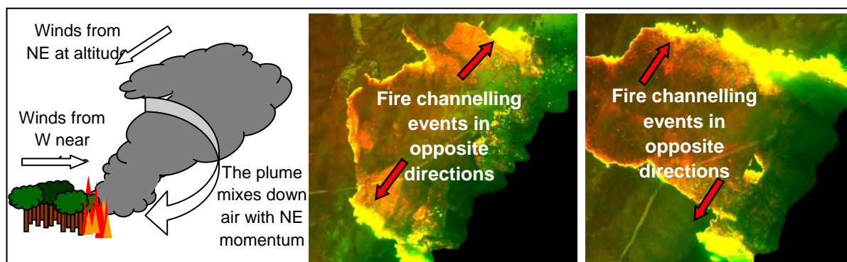
Figure 3. Schematic illustrating how a fire plume mixes down air with momentum travelling in a different direction to surface winds (left) and two line-scan images showing fire channelling events propagating in opposite directions (centre and right).
