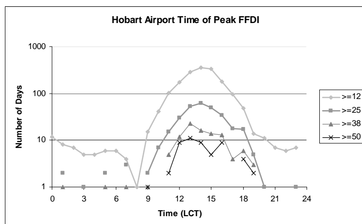
Figure 5. Frequency analysis of times of Peak FFDI for various FFDI ranges at Hobart Airport, plotted with a logarithmic y-scale to better resolve the plots displaying differing ranges of FFDI.
