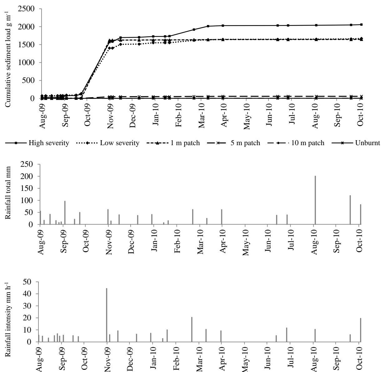
Figure 6: Time series charts showing (a) the cumulative sediment load; (b) the rainfall total contributing to each measurement date; and (c) the 30-minute maximum ( I_{30} ) rainfall intensity contributing to each measurement date.
