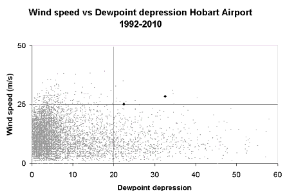
Figure 8. Scatterplot of Hobart Airport 850 hPa wind speed ( \text{m s}^{-1} ) and dewpoint depression ( ^\circ\text{C} ) from routine 2200 or 2300 UTC (0900 local time) radiosonde soundings between 1992 and 2010. The two case study values are indicated by black diamonds. Threshold values of 25 \text{ m s}^{-1} and 20^\circ\text{C} are represented by gridlines
