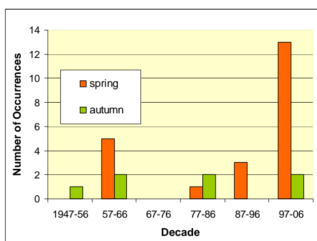
Figure 2. Comparison of spring and autumn counts of FFDI 40 or more at Hobart City, binned by decade.
