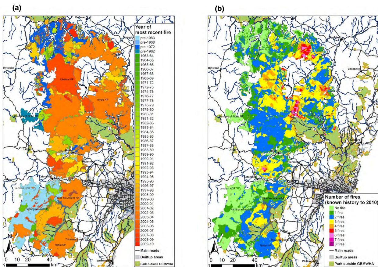
Fig 1: (a) Time of last fire, and (b) number of fires, for the Greater Blue Mountains World Heritage Area for the period of available fire history to 2010. Note that only fires within the GBMWhA reserves are shown and the length of fire history varies for the different
