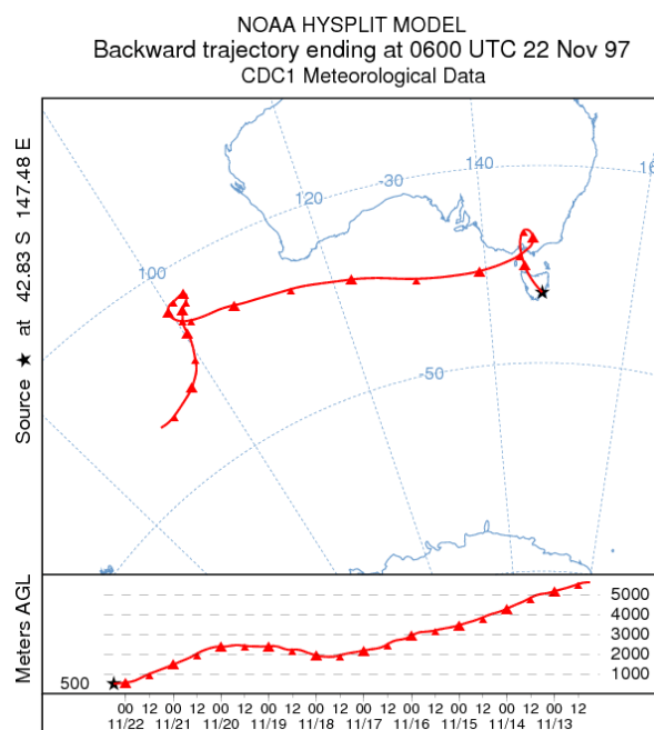
Figure 10. Airmass trajectory for the 10 days leading to 0600 UTC (1700 LCT) 22 November 1997. Figure courtesy of NOAA Air Resources Laboratory, using NCEP/NCAR reanalysis data.
