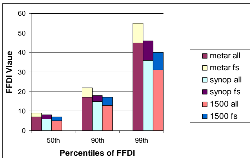
Figure 4. Stacked clustered column plots of 50 th , 90 th and 99 th percentile FFDI at Hobart Airport. “All” observations include those through the year, while “fs” include October-March fire season observations. The columns represent “metar” (half-hourly), “synop” (three hourly and 1500-only observations).
