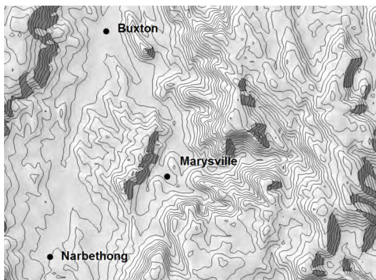
Figure 10. Output of the wind-terrain model overlayed on 10m DEM contours. The model indicates a significant fire channelling-prone landform immediately to the west of Marysville.
