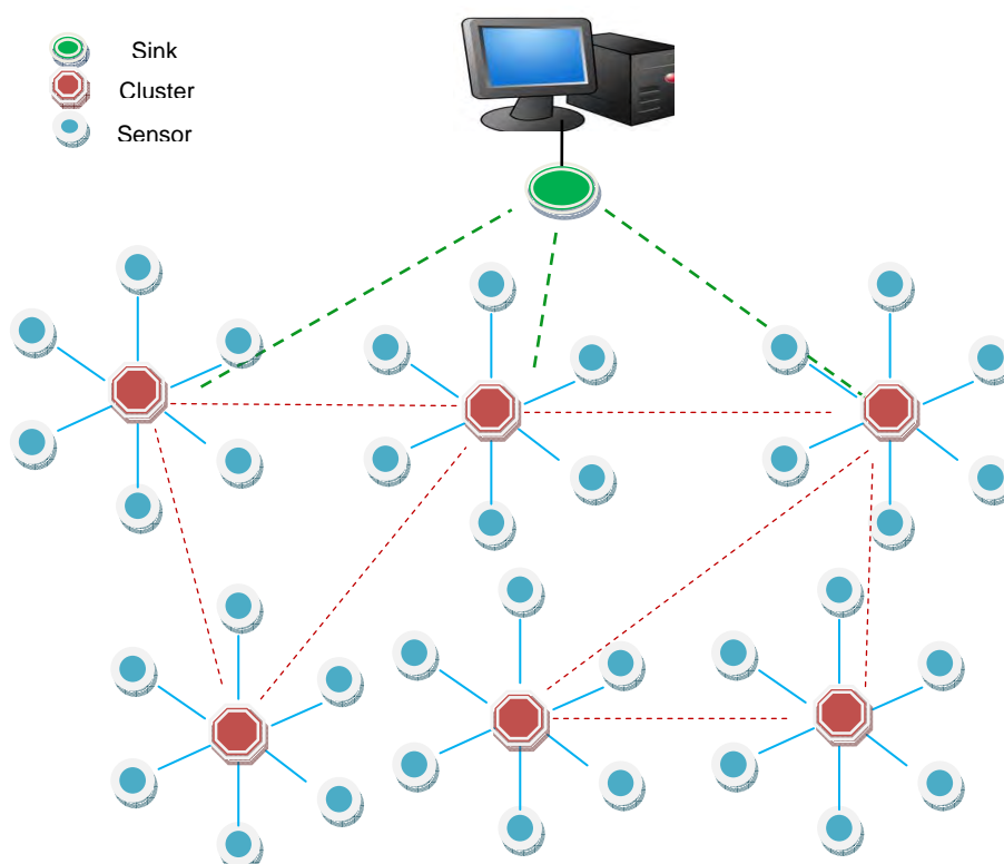
Figure 3. The WSN cluster architecture
