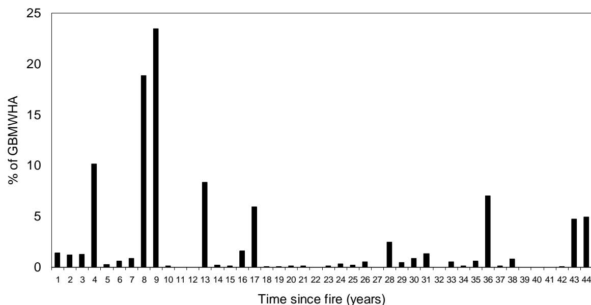
Fig 2: Proportions of the Greater Blue Mountains World Heritage Area in each time-since-fire category, as at 2010.
