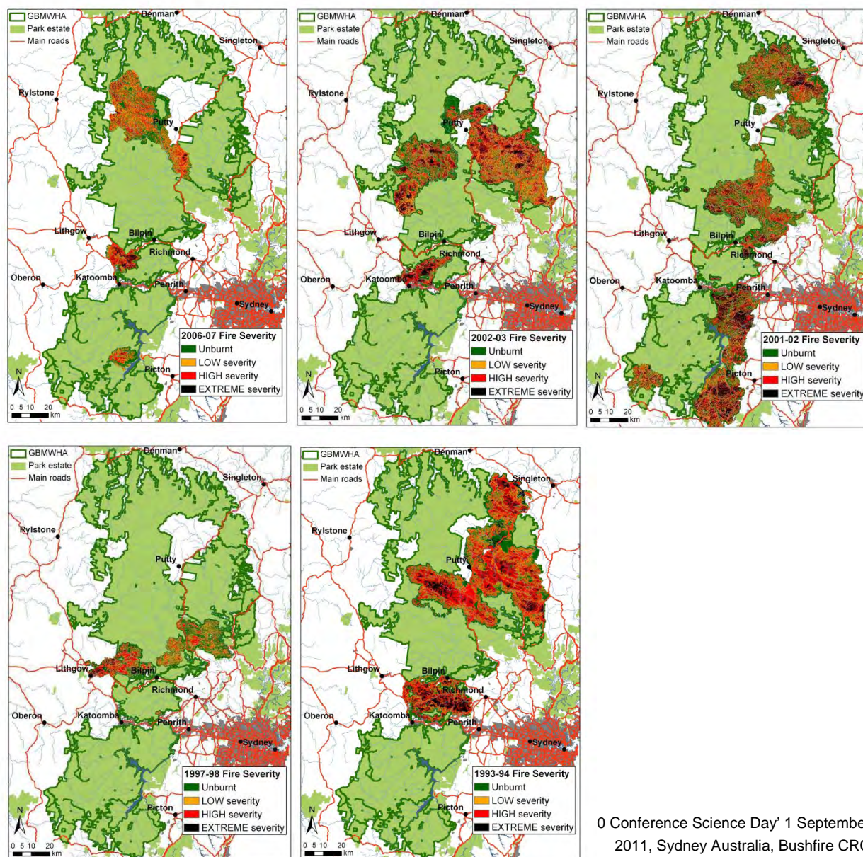
Fig 5: Fire severity maps produced in this study for the five major bush fire seasons since 1990.
