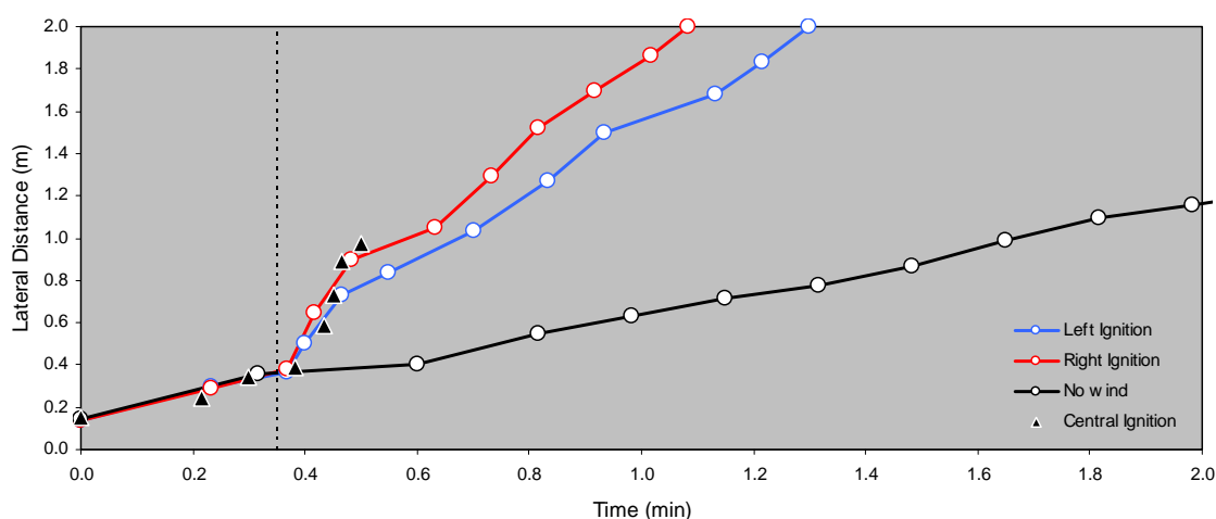
Figure 8. Comparison of maximum lateral distance travelled versus time since ignition for the different ignition locations and the wind and no wind cases. The dashed vertical line marks the time when the fire reached the top of the slope.
