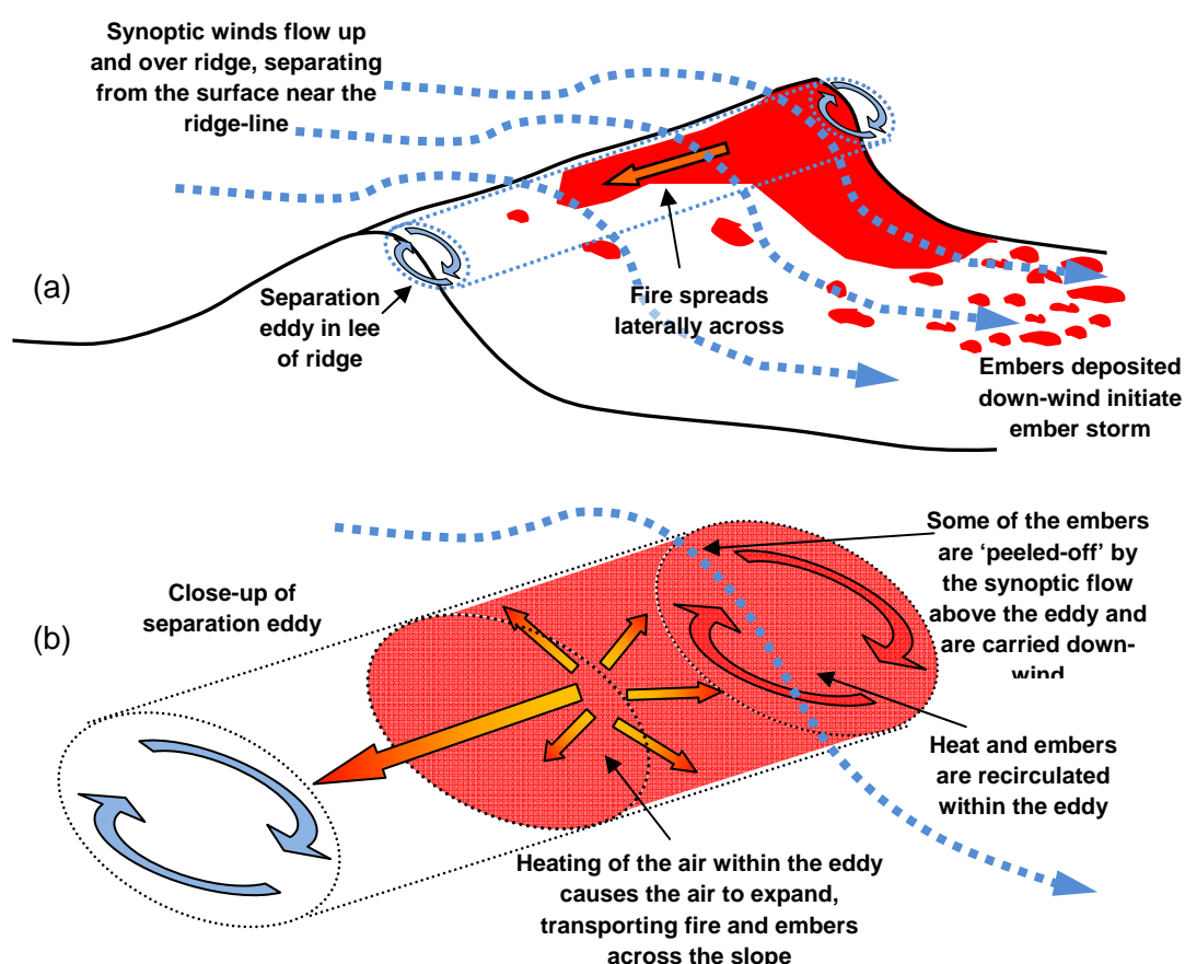
Figure 5. Schematic diagram illustrating the fire channelling hypothesis. (a) Diagram showing the rotor (separation eddy) in the lee of the ridge, the fire spreading across the slope and the mass spotting downwind. (b) Close up of the separation eddy illustrating how the recirculated heat and embers cause expansion of the air, which transports heat and embers across the slope.
