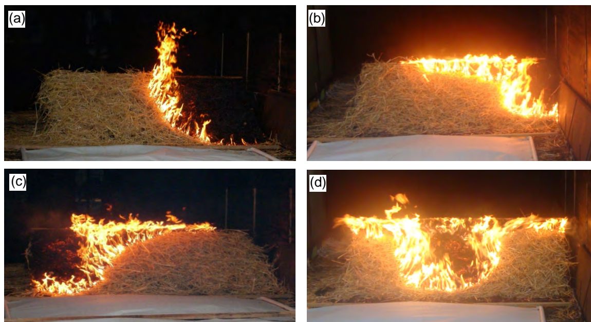
Figure 7. Experimental fires burning across the lee slope. (a) right side ignition, no wind; (b) right side ignition with 4 \text{ ms}^{-1} wind; (c) left side ignition with 4 \text{ ms}^{-1} wind; (d) central ignition with 4 \text{ ms}^{-1} wind.
