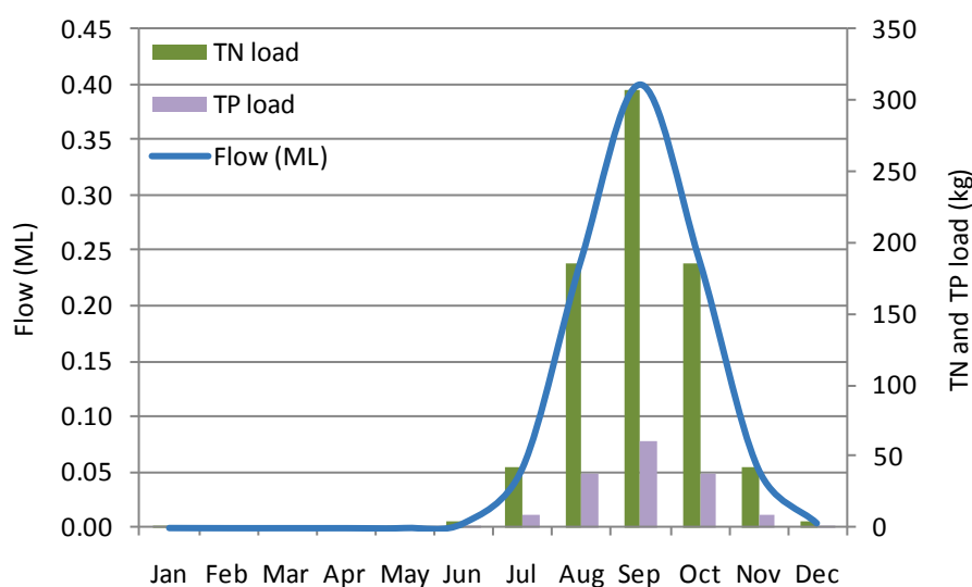
Figure G-1 Timeseries of nutrient load and flow for a single dairy
