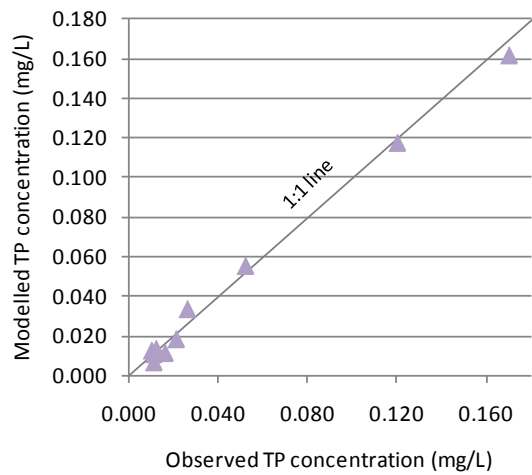
Figure G-4 Observed and modelled median winter concentrations for calibration sites
