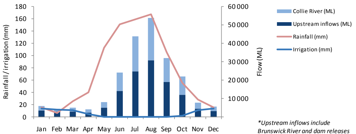
Collie River modelled monthly flows (1997 – 2008)
