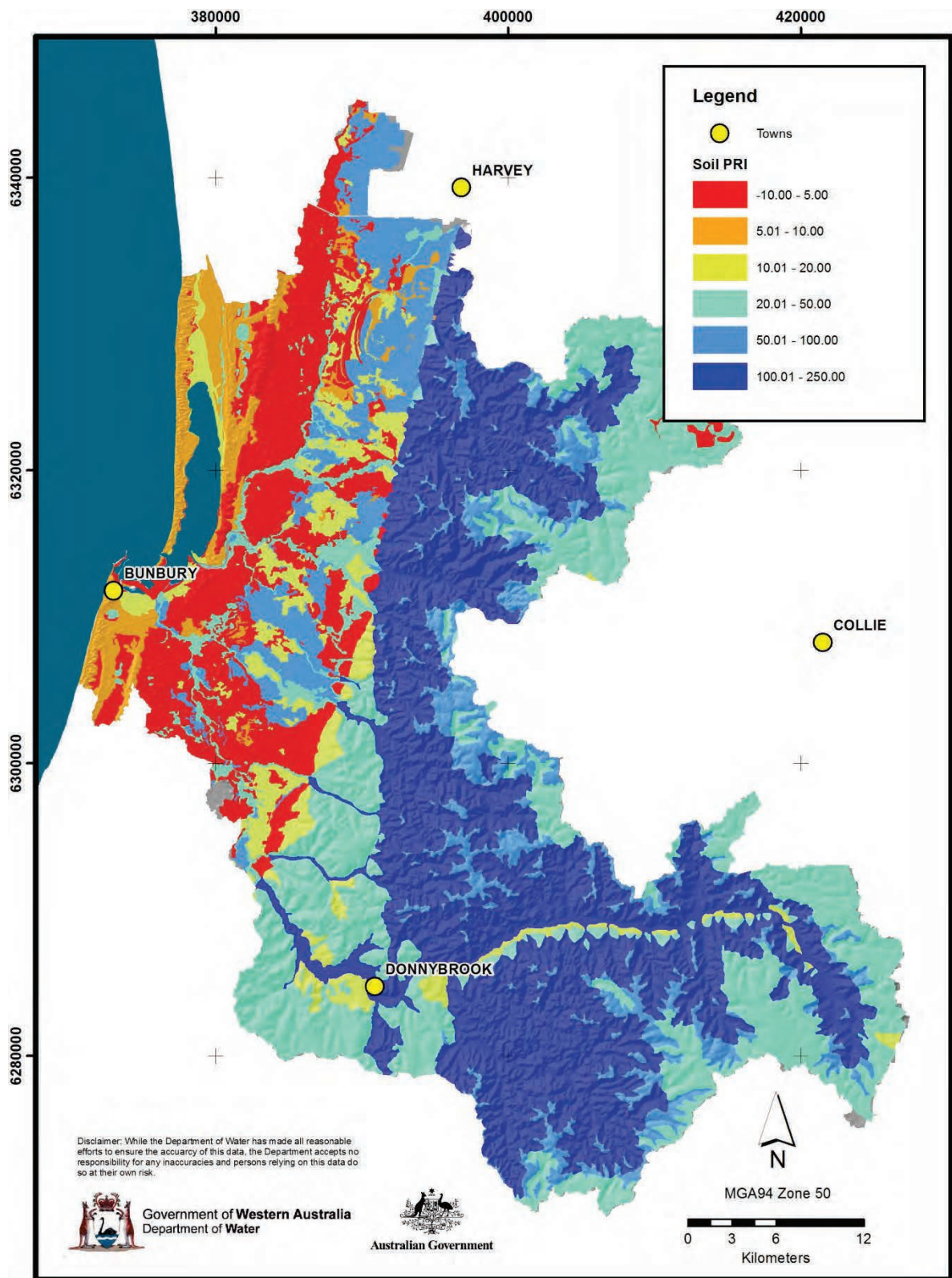
Figure A.3 Soil Phosphorus Retention Index (PRI) map of the catchment
