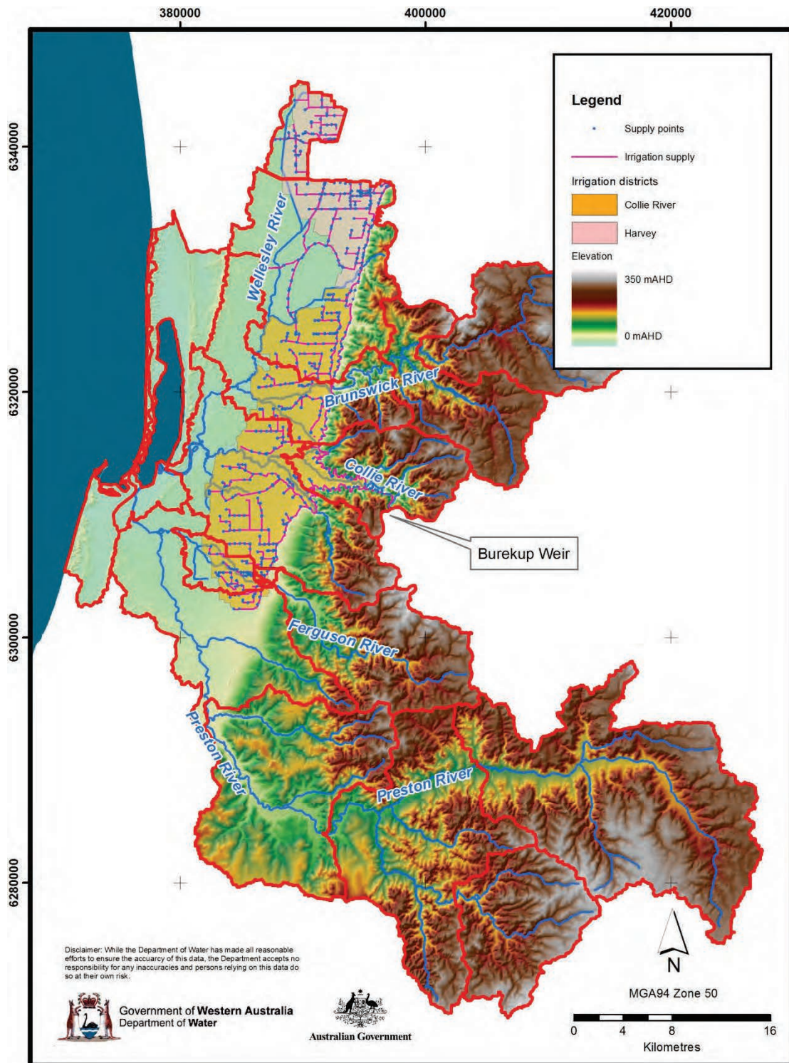
Figure A.6 Surface water hydrology of the Leschenault catchment
