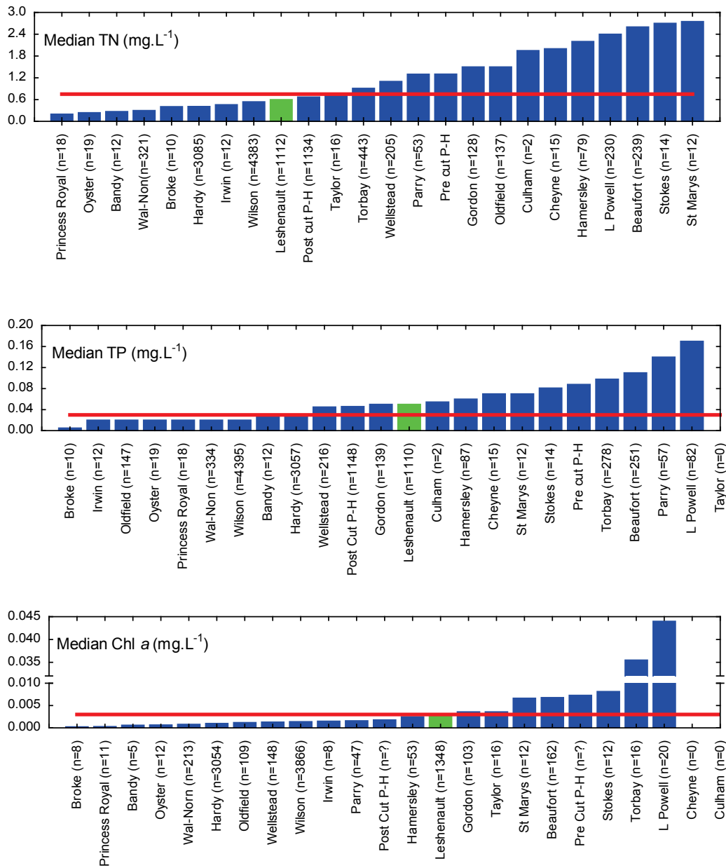
Figure E.6 Total phosphorus, total nitrogen and Chl a concentrations in south west estuaries
