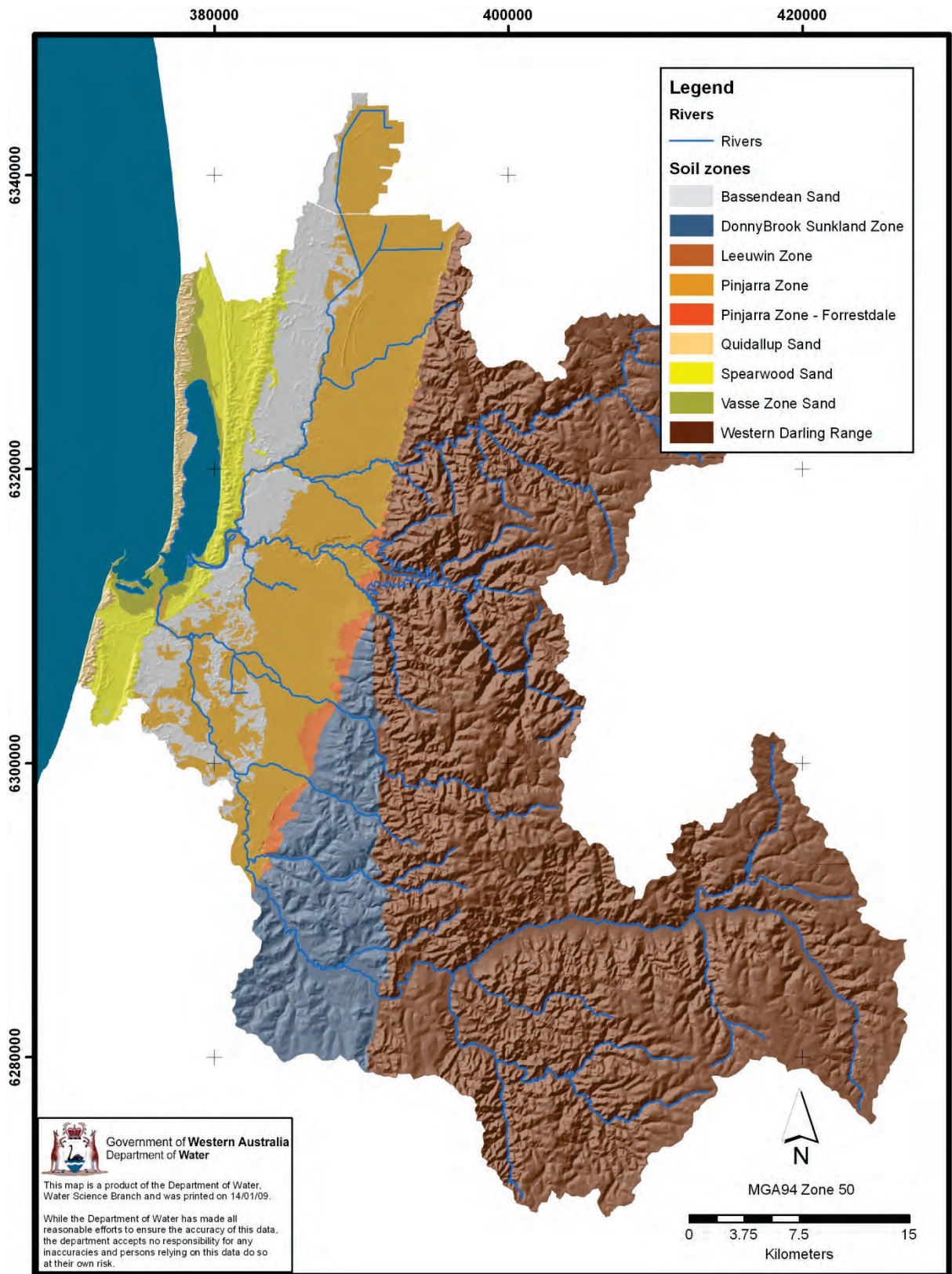
Figure A.2 Soils in the Leschenault Catchment
