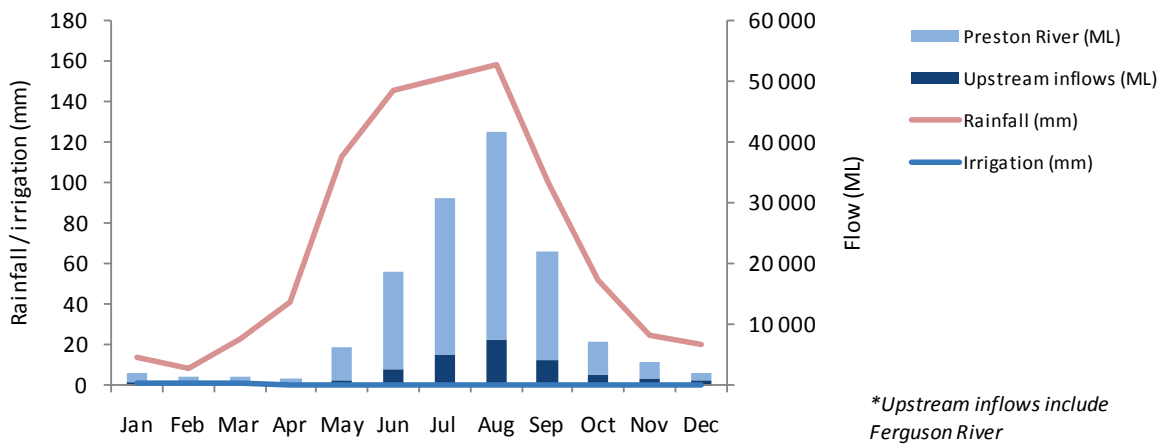
Preston River modelled monthly flows (1997 – 2008)
