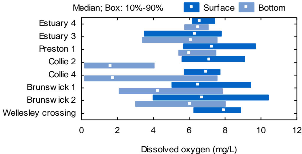
Figure 3-3: Median (point) and 80% of data for surface and bottom dissolved oxygen concentrations. Data collected from October to May (dry season) during 2006 to 2009.
