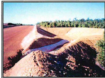
Figure 7. Drainage is captured and prevented from entering uninfested areas
