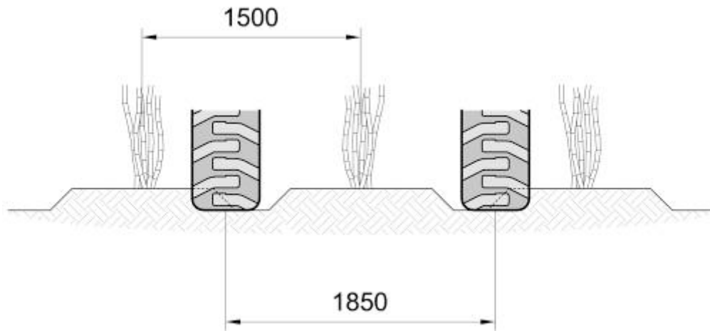
Figure 2.4 Wheel spacing 1.5 m row spacing – 1.85 m wheel spacing
