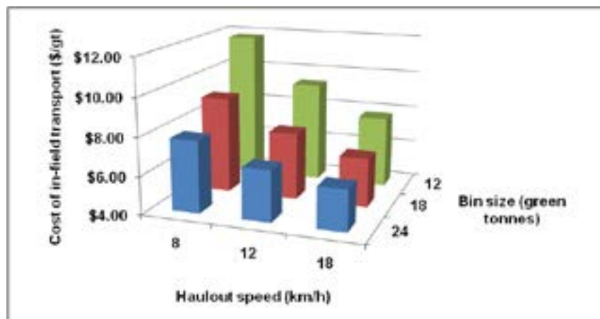
Figure 3.11 The effect of haulout travel speed and bin size on infield transport costs (McCormack et al. 2009)
