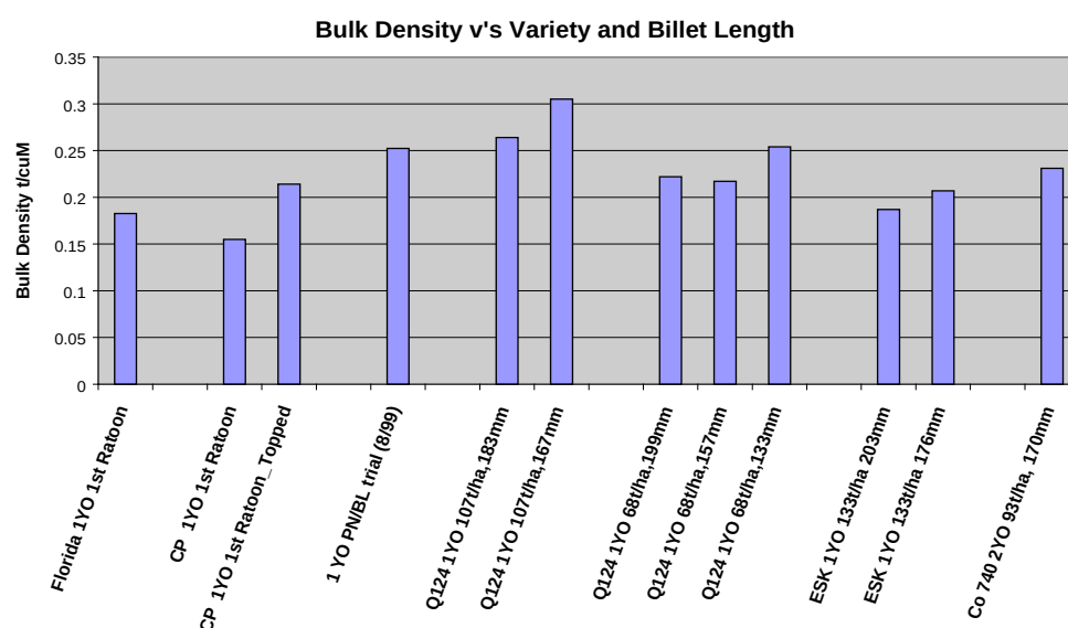
Figure 2.8 Bulk densities of whole-cane
