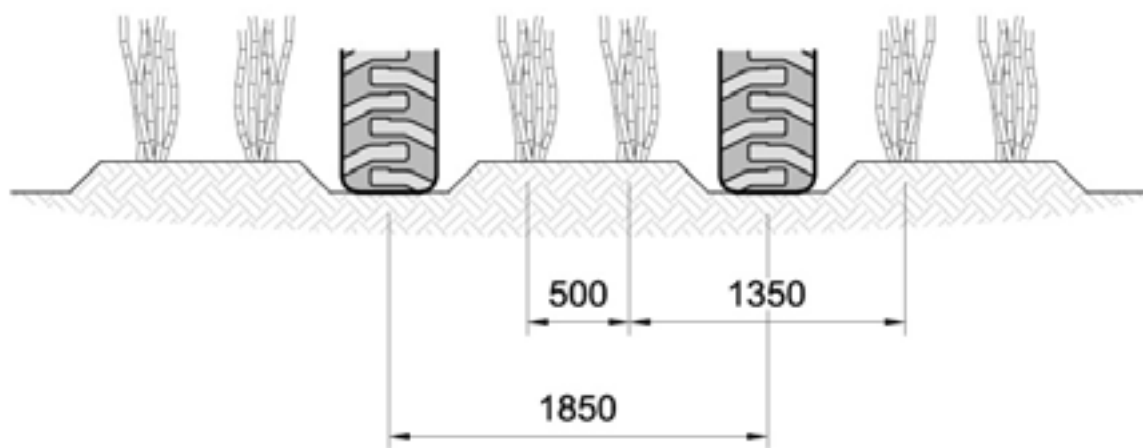
Figure 2.5 Wheel spacing: 1.85 m wheel spacing - dual row
