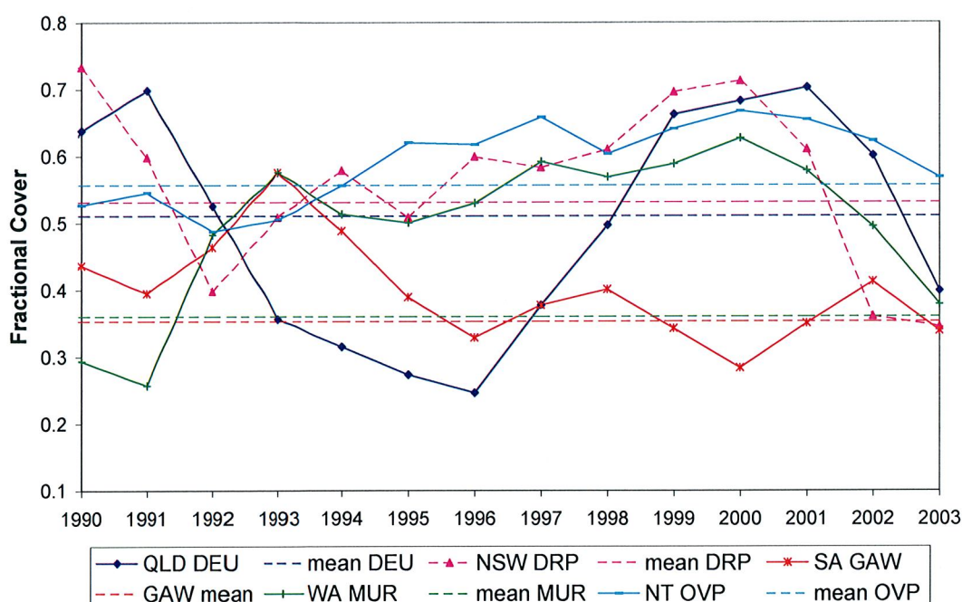
Figure 4 Simulated yearly fractional cover and the long-term (1890–2003) mean for bioregions produced by Aussie-GRASS
