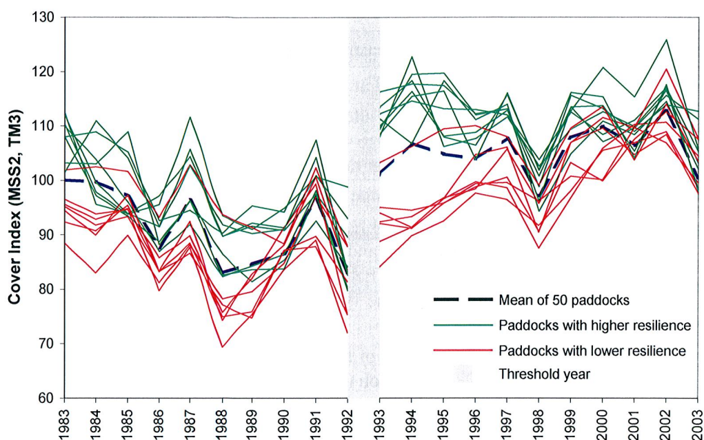
Figure 6 Yearly time traces of average cover on Basalt Plains combined land type in selected paddocks of greater than 80 km 2 .
