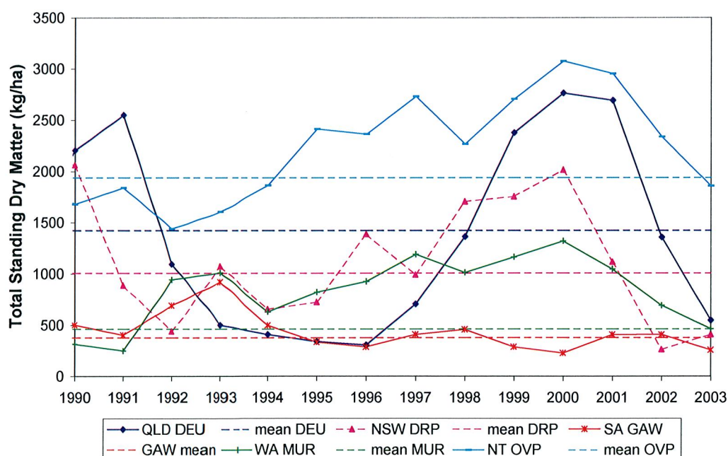
Figure 3 Aussie-GRASS simulated yearly total standing dry matter and the long-term (1890–2003) mean for selected bioregions
