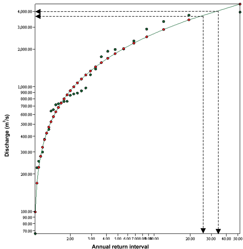
Figure 45: Annual series flood frequency curve for lower Ord River
