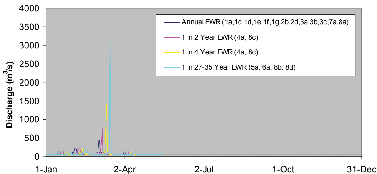
Figure 50: Lower Ord River comprehensive EWR hydrographs
