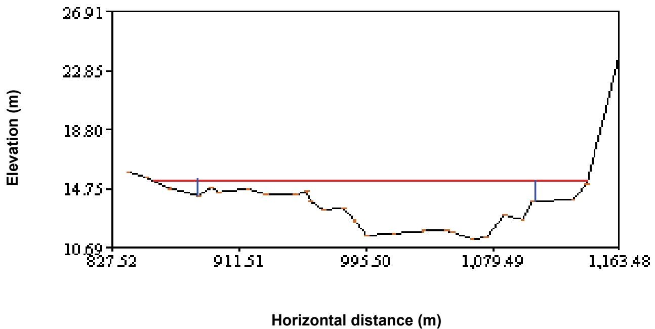
Figure 4: Example cross section showing inundation of benches at discharge of 125 m³/s
