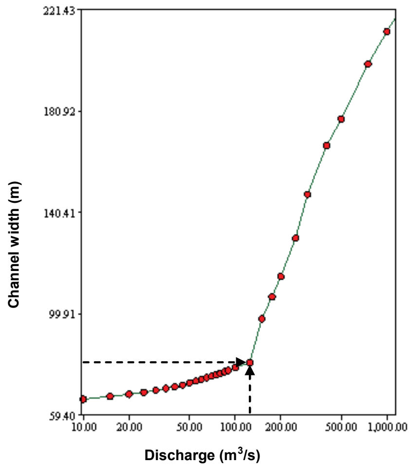
Figure 3: Flow rating curve of area of channel with depth >1m with discharge. Arrows indicate flow and channel width at 125 m³/s
