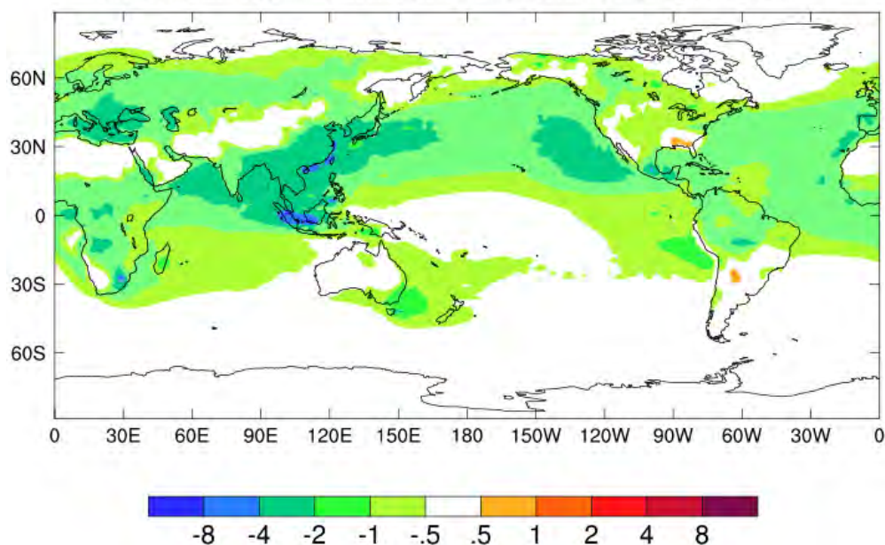
Figure S7 The cooling influence of aerosols. Note that this cooling influence (shown as green through blue areas) on solar radiation intensities (in Watts per square metre) at the top of the atmosphere is most pronounced in the South-East Asian Region, just across the equator from Australia. These estimates were calculated using the CSIRO Mk3.6 global climate model.
