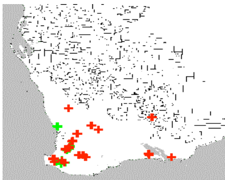
MODIS hotspot detection Terra-1 APR 28 22:20 2004 WST
