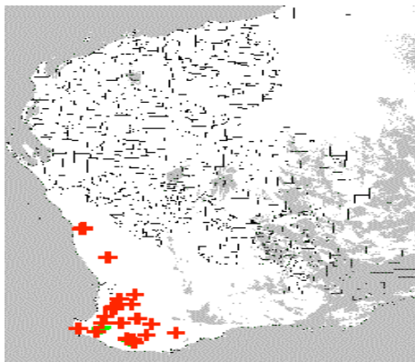
MODIS hotspot detection Aqua-1 MAY 05 00:56 2004 WST
