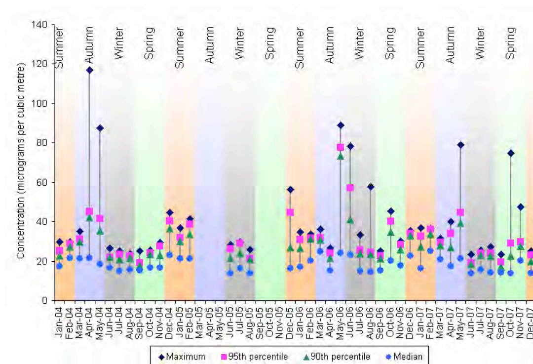
Figure 4 Daily averaged percentiles for PM 10 , during 2004 - 2007
