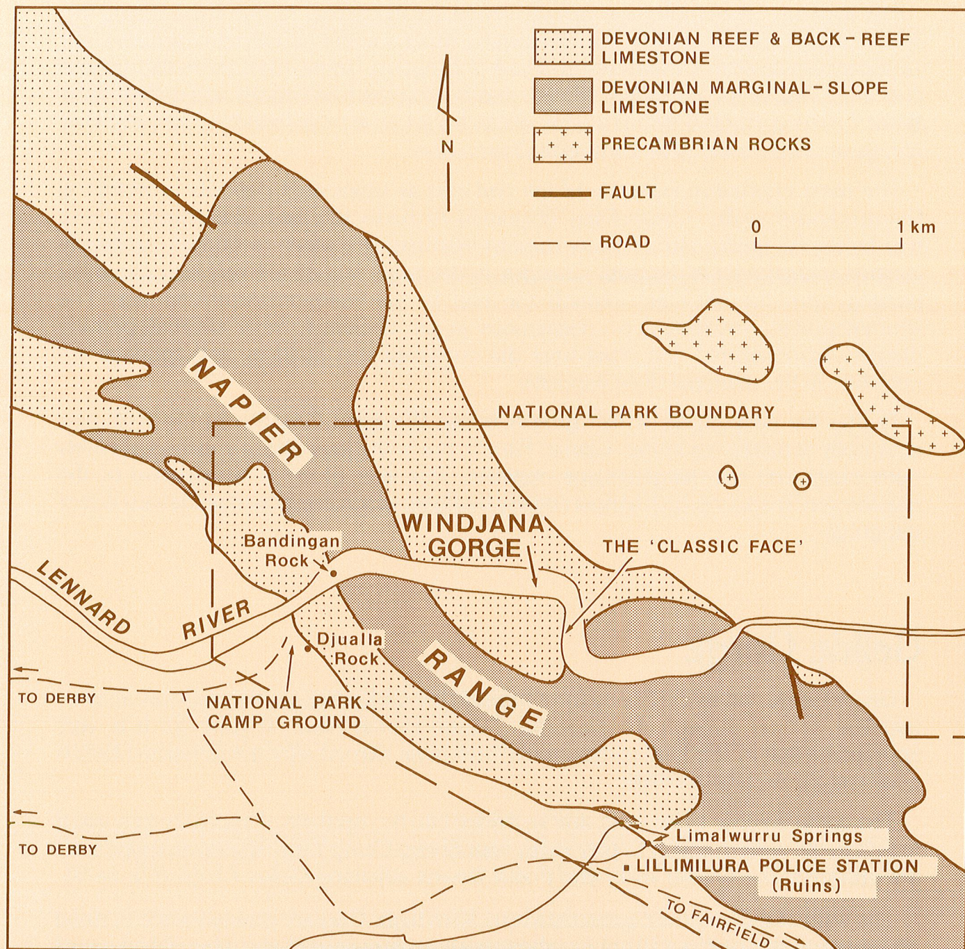
Figure 7: Geological map of the Windjana Gorge area.
