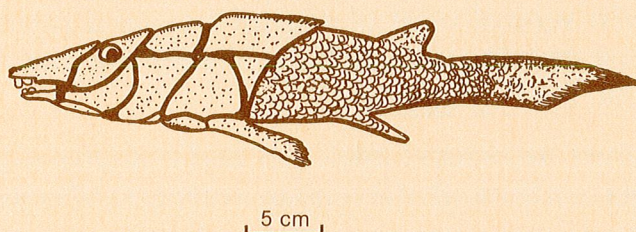
4. FISH
