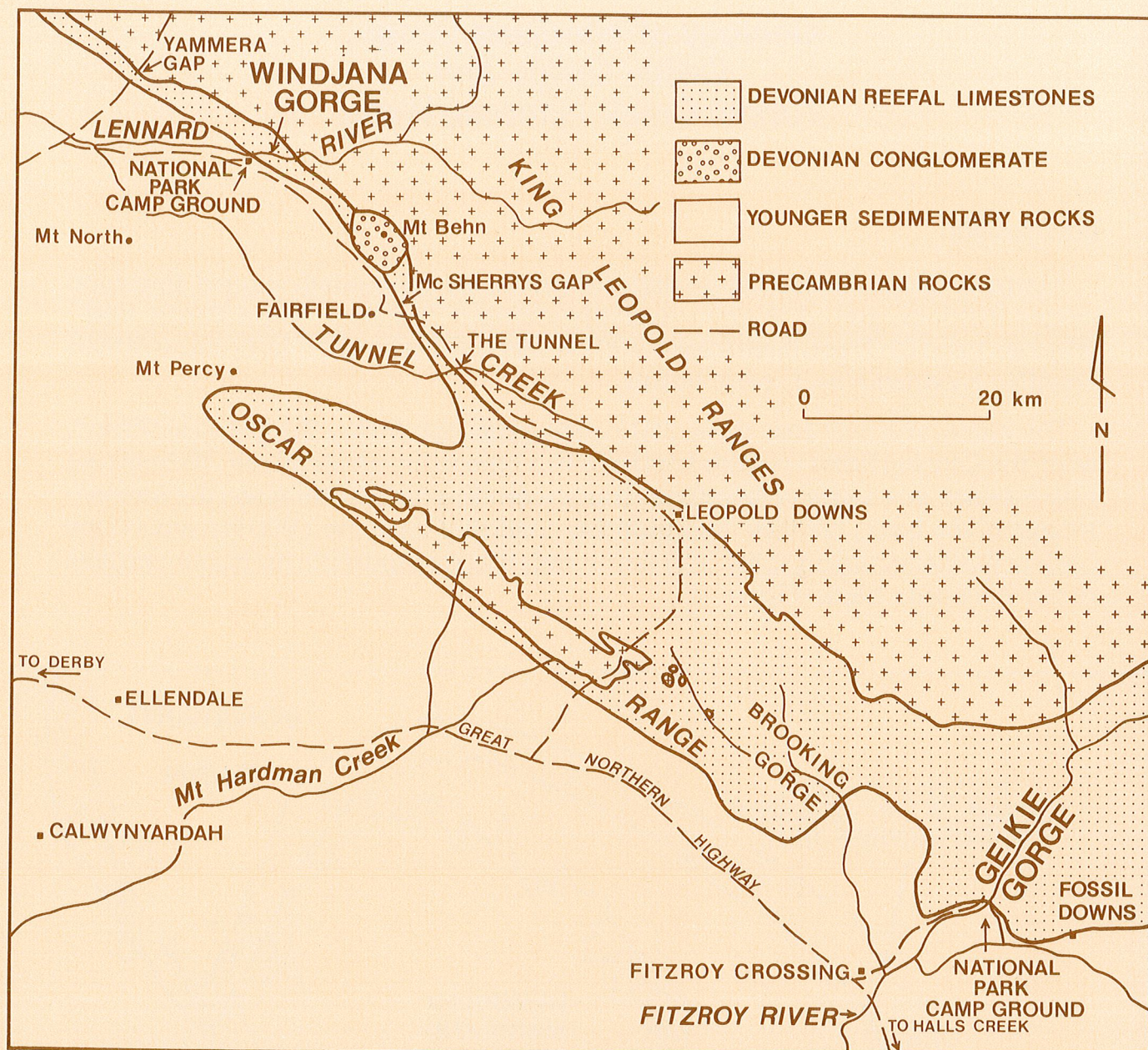
Figure 2: Geological map of the Windjana Gorge-Geikie Gorge area.
