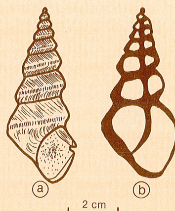
2. GASTROPOD
