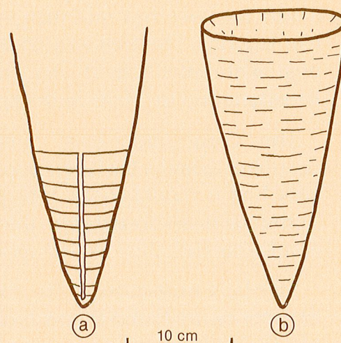
5. NAUTILOID
