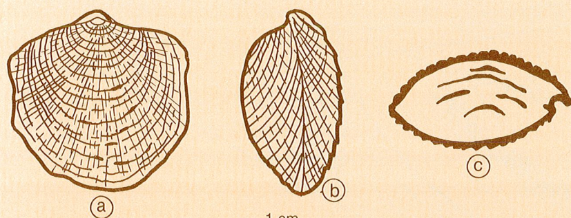
1. BRACHIOPOD
