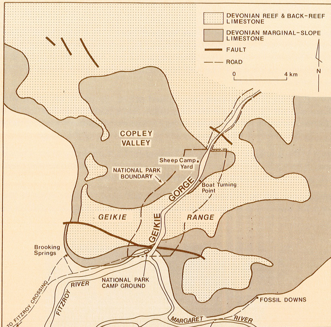
Figure 9: Geological map of the Geikie Gorge area.
