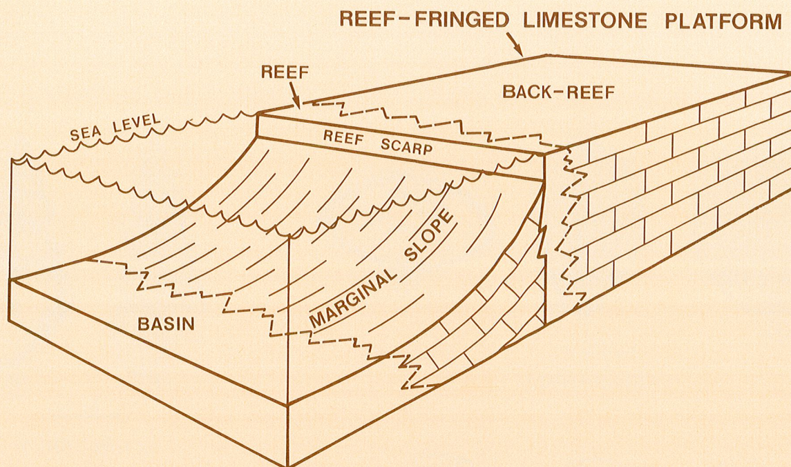
Figure 6: Diagrammatic section illustrating the structure of the Devonian reef complexes. The reef-fringed limestone platforms stood up to several hundred metres above the adjoining basins and were fronted by steeply inclined marginal-slope deposits.
