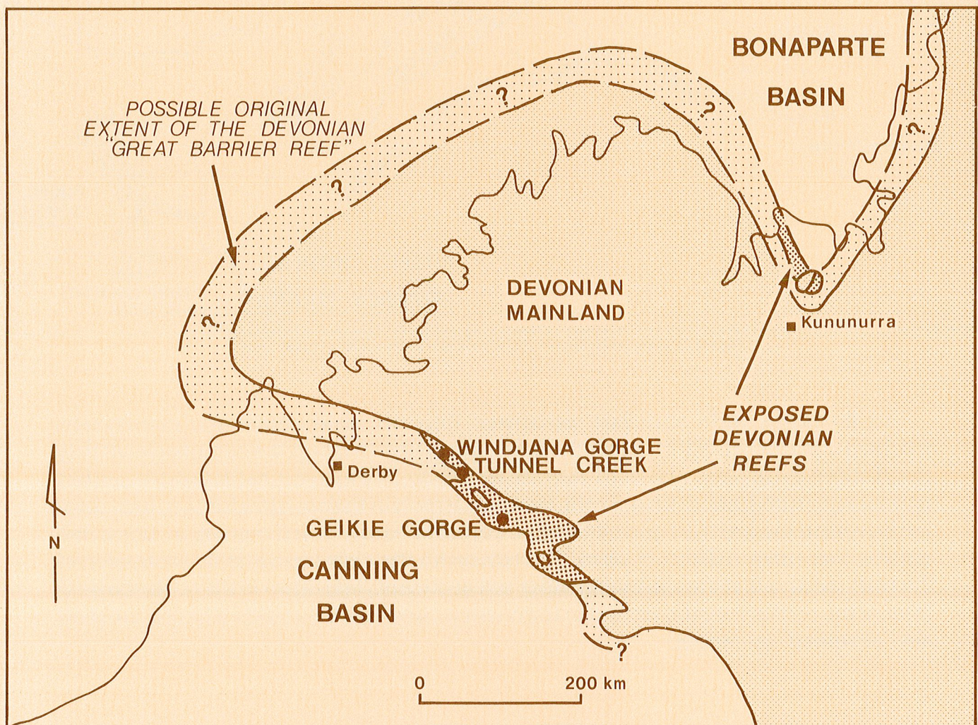
Figure 1: Map of the Kimberley district showing the outcrop area of Devonian reefs in the Canning and Bonaparte Basins, and the possible original extent of the Devonian "Great Barrier Reef".
