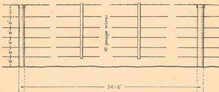
FIG. 3. STOCK PROOF FENCE (For Small Stock)
