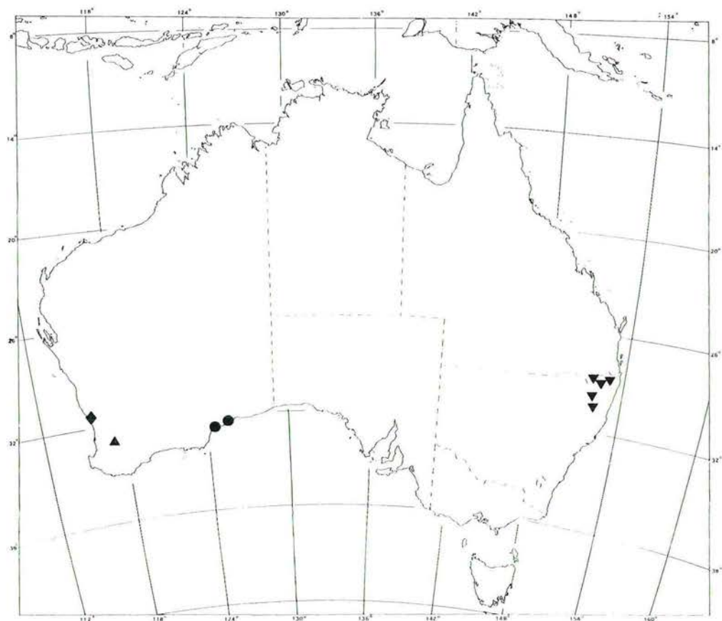
Map 1. Distribution of Banksia oligantha (▲), B. epica (●), B. leptophylla var. mellitica (◆) and B. spinulosa var. neoanglica (▼).
