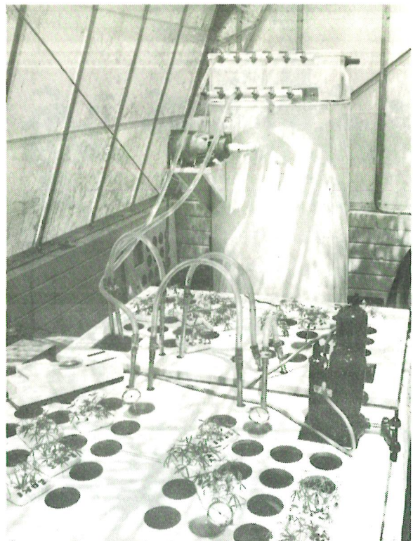
Plate 1 Insulated water baths showing cooling unit, coils and Haake temperature control units.
