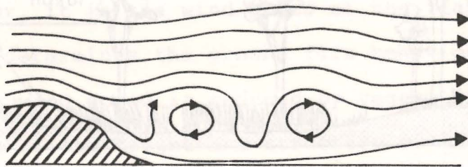
FIGURE 7: Probable airflow pattern over the Darling Scarp during the night.
