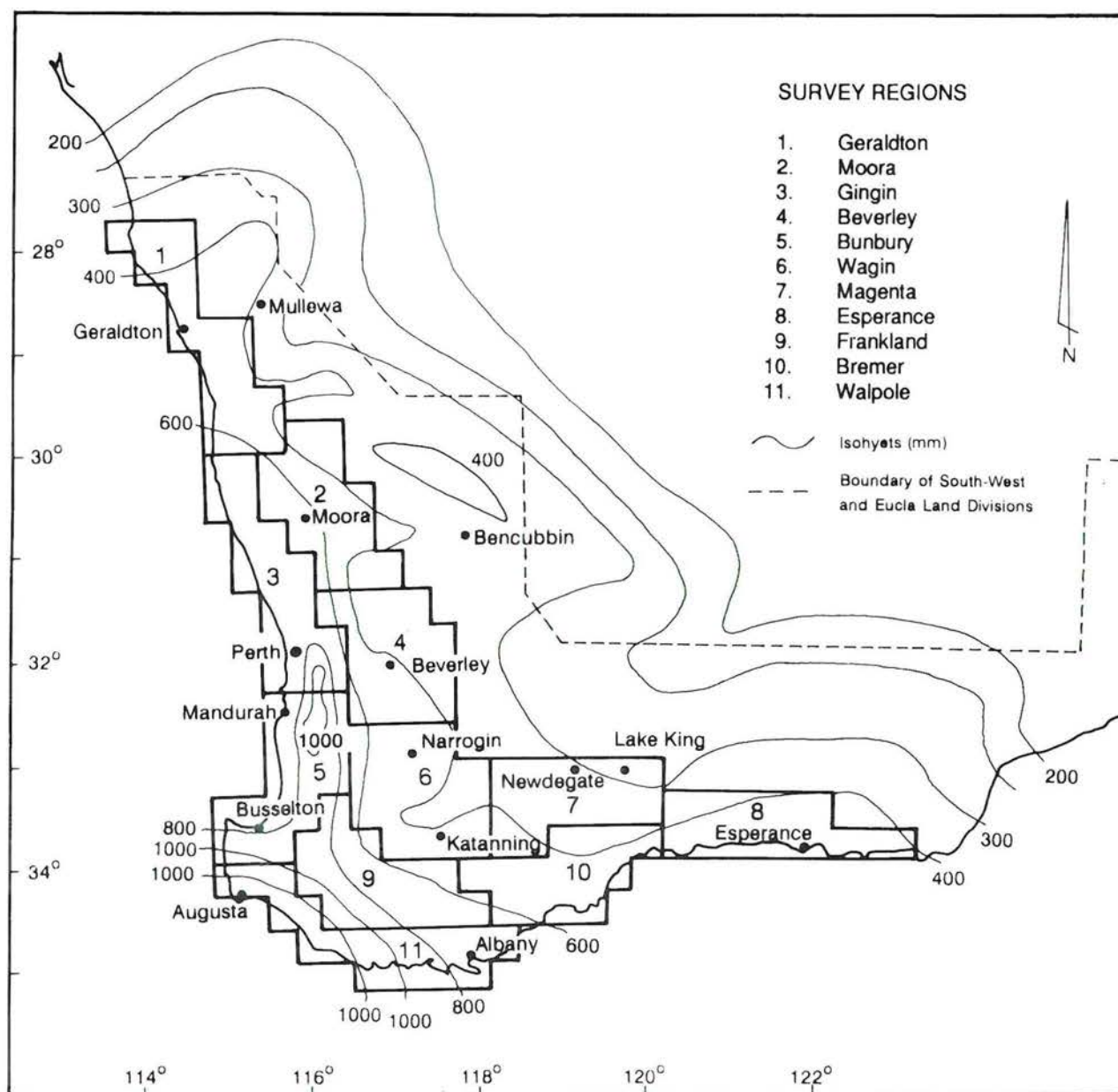
Figure 3 Rainfall (mm) in south-western Australia between January and November 1988.
