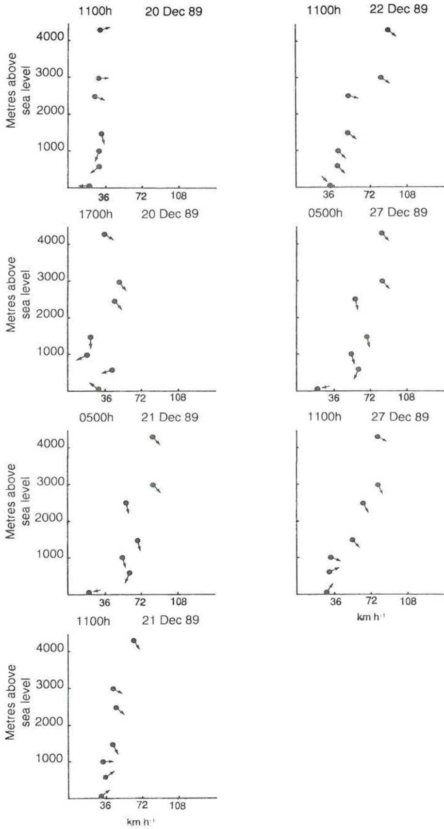
Figure 3 Upper level wind speed (●) and direction (↑ = north) at Albany for various times on 20, 21, 22 and 27 December 1989.
