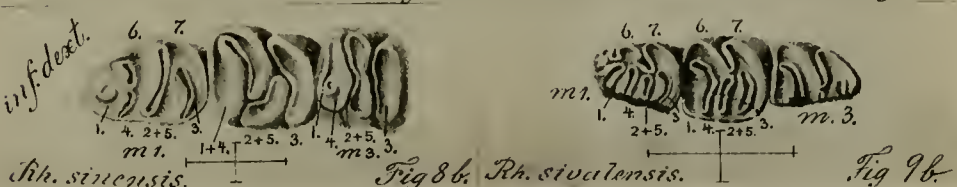
Enlarged upper and lower molar teeth of recent and fossil SPECIES OF RHIZOMYS.
