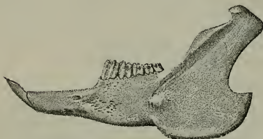
Skull of Lepus atlanticus (side view). Nat. size.
