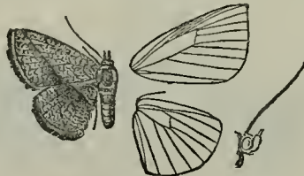
Striglina scitaria , ♂ \frac{1}{2} . (From Moths Ind. vol. i.)
