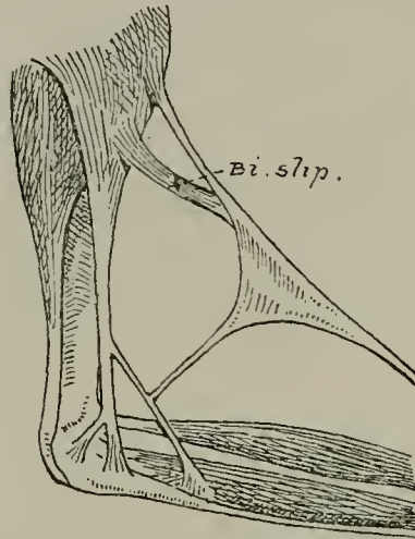
Muscles and tendons of Patagian of Phaethon .
