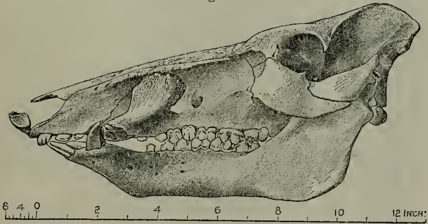
Skull of Potamochoerus larvatus , ♂, from Madagascar (side view).
