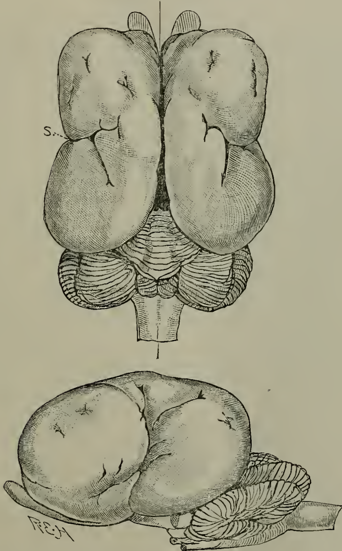
Brain of Manatus inunguis . The upper figure represents the dorsal aspect, the lower a lateral view.
