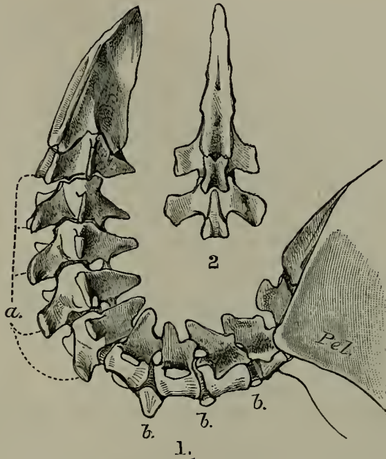
Caudal vertebræ of Biziura lobata . 1, lateral view; 2, from below. Pel., pelvis; a, hypocentra; b, free intercentra.
