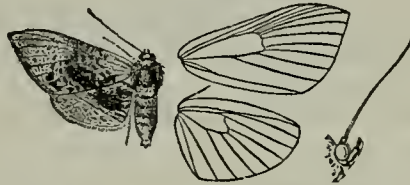
Rhodoneura acaciusalis , ♂. ¼. (From Moths Ind. vol. i.)
