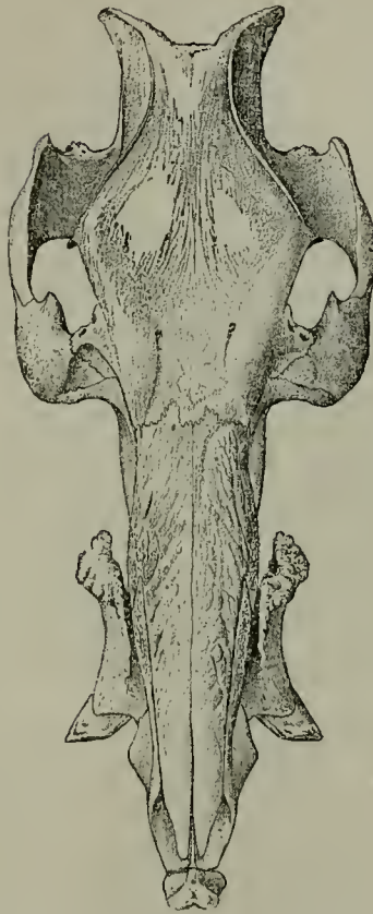
Skull of Potamochoerus larvatus , ♂, from Madagascar (seen from above).
