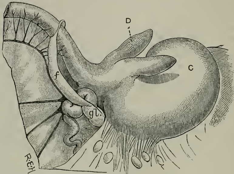
Caecum of Manatus inunguis .
