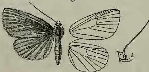
Beguma constellata , ♂. \frac{1}{2} .
