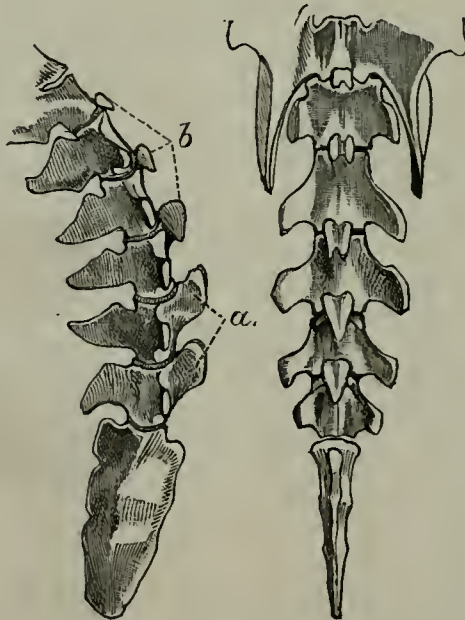
Colymbus septentrionalis . Lateral (left-hand figure) and ventral aspects of caudal vertebræ.
