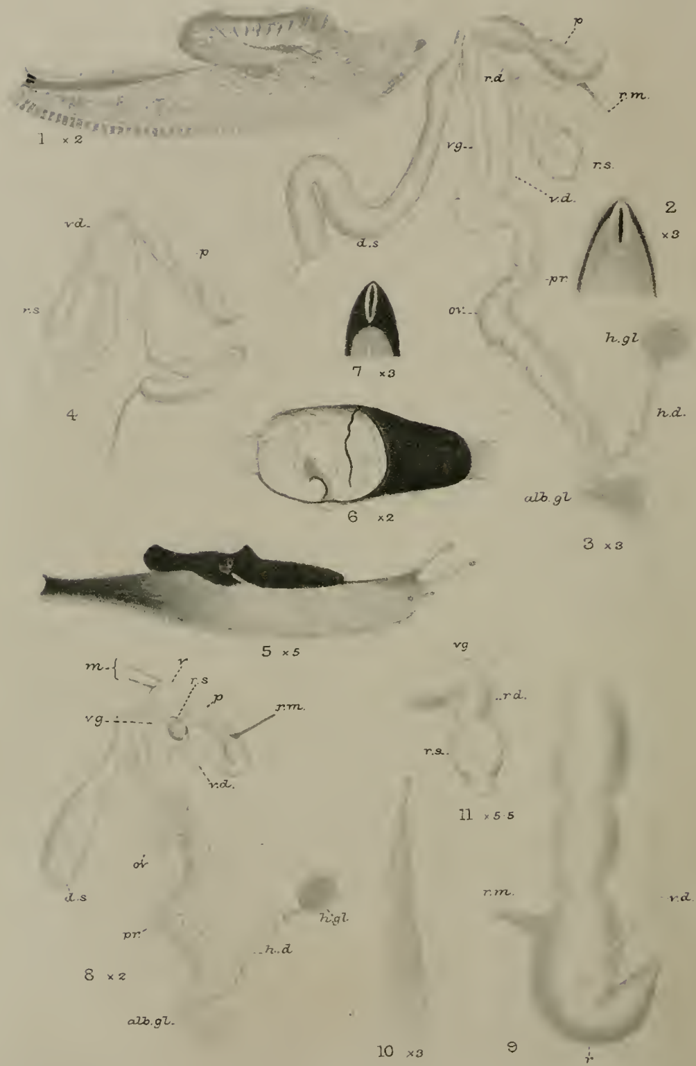
Slugs of the Genus Parmarion.
