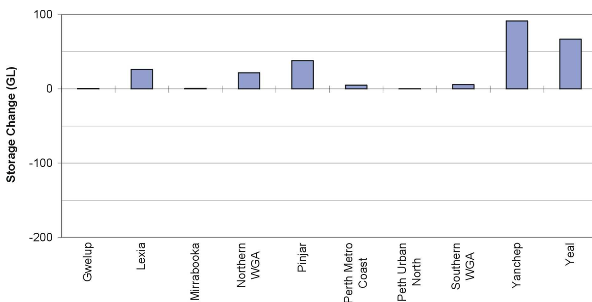
Figure 41. Storage changes for each of the Gnangara Mound Zones – Scenario 5: Pines removal.
