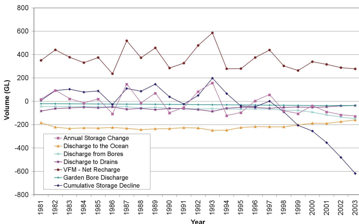
Figure 43. PRAMS annual water balances for the Gnangara Groundwater Mound.
