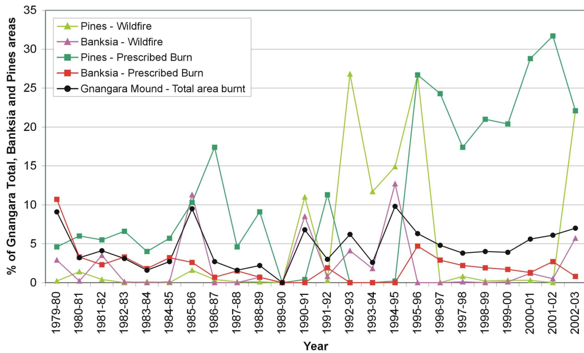
Figure 11. Percentage areas burned (prescribed and wildfires) for pines, Banksia and the Gngara Groundwater Mound.
