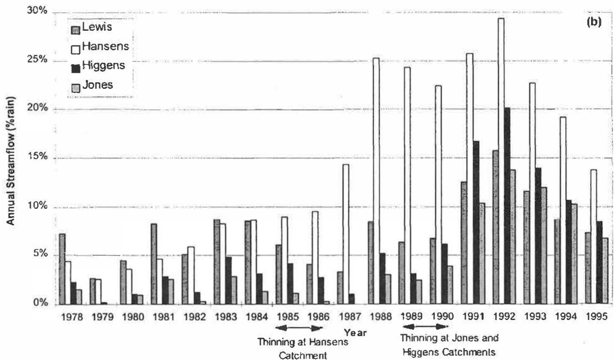
Figure 15: Annual streamflow (%rain) for Lewis, Hansens, Higgens and Jones
