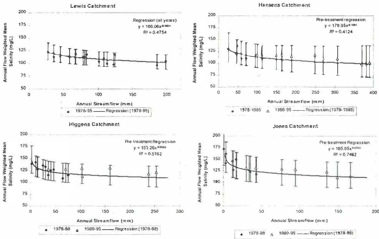
Figure 25: Stream salinity-streamflow relationships
