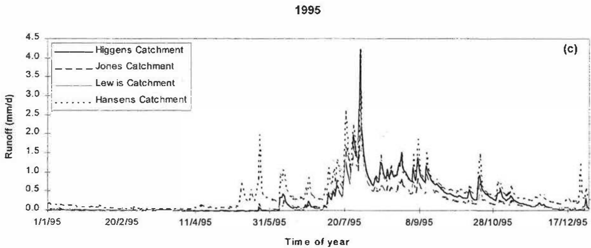
Figure 13: Daily streamflow for the years 1978, 1992 and 1995 for Lewis, Hansens, Higgens and Jones
