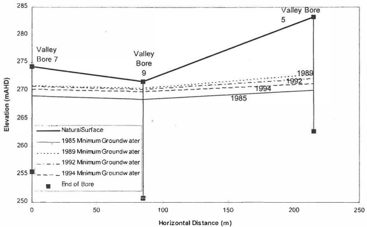
Figure 8: Groundwater level variation along the cross section at Hansens
