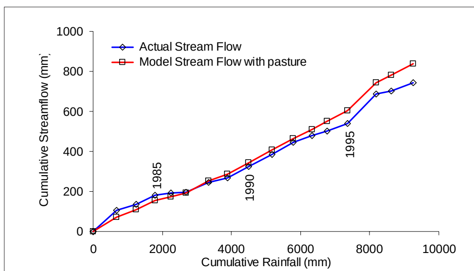
Figure 6.8 Maringee Farms Catchment streamflow
