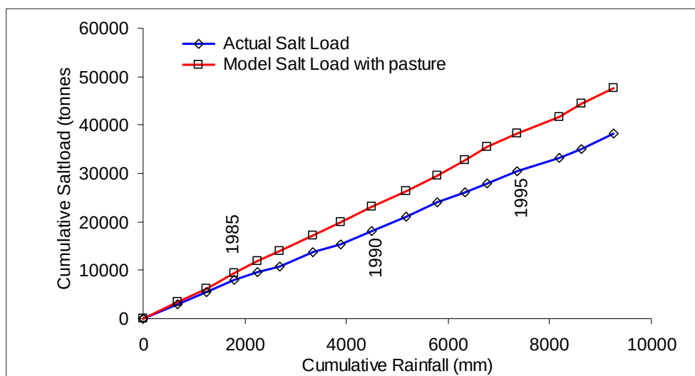
Figure 6.7 Maringee Farms Catchment salt-load
