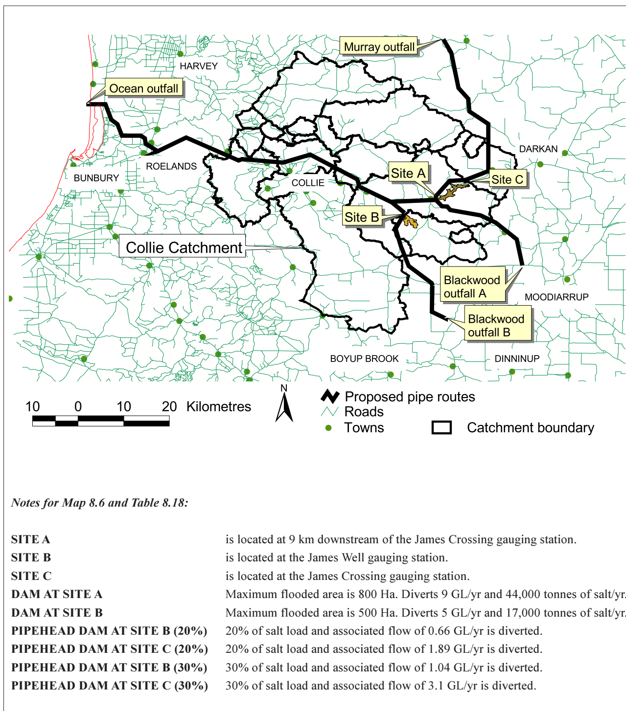
Map 8.6 Location of possible stream diversion sites and pipeline routes
