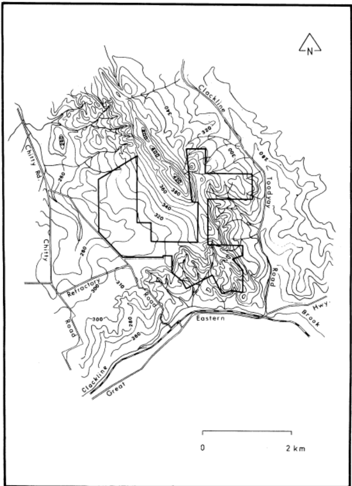
Figure 5. Clackline Nature Reserve showing the associated, contours (m). (Source: W.A. Department of Land and Surveys 1:50 000 series.)
