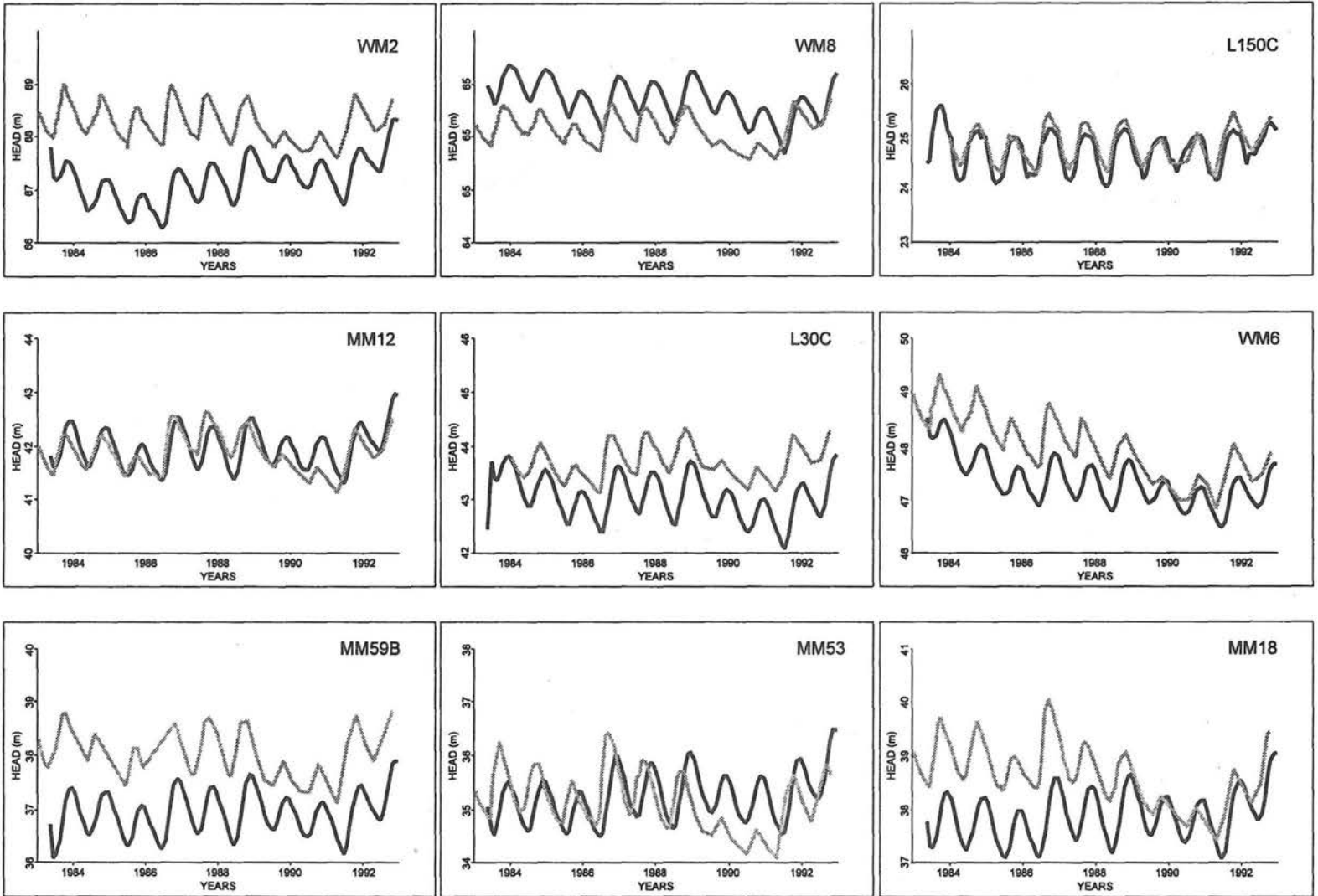
FIGURE 19 - EAST GNANGARA Model Calibrations at Criteria Wells.
