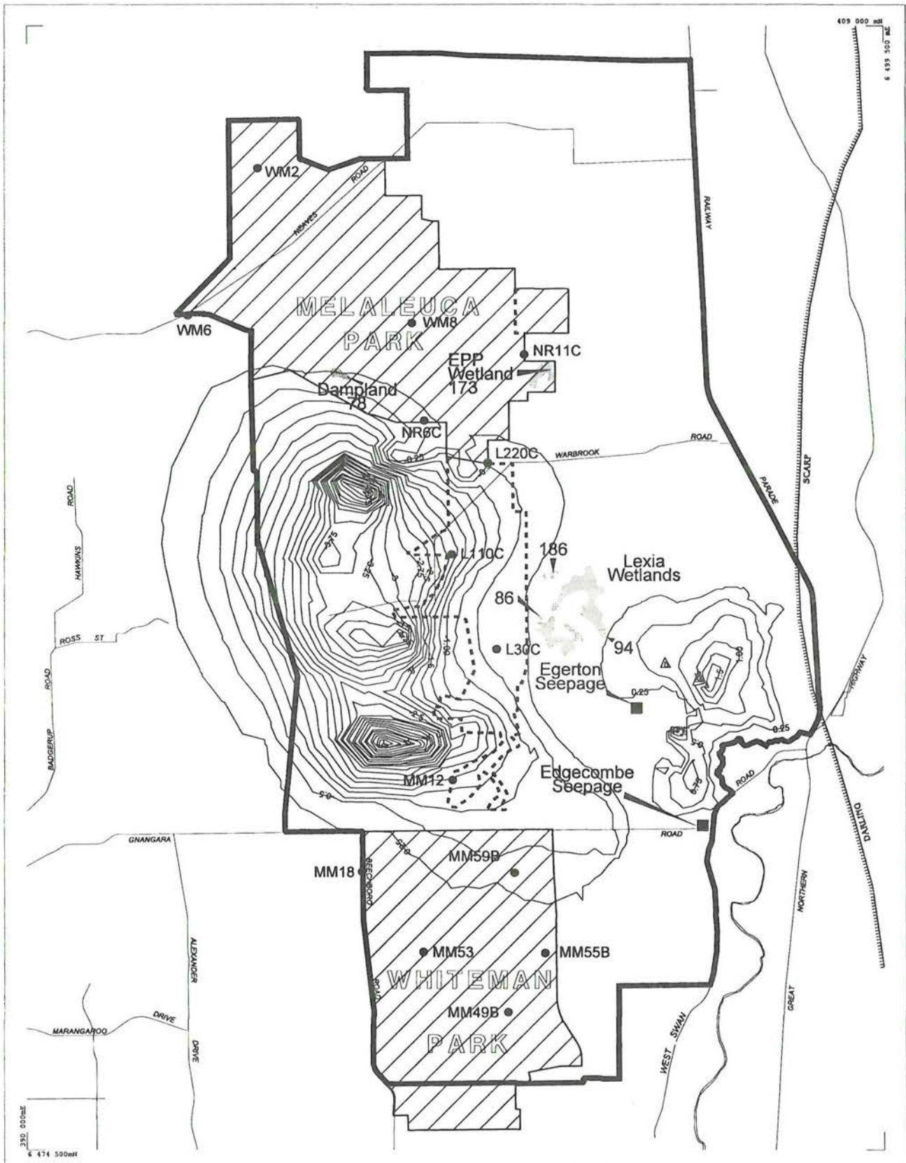
FIGURE 24 EAST GNANGARA MOUND. Impact of Proposed Lexia and East Mirrabooka Groundwater Schemes (Urbanisation included)
