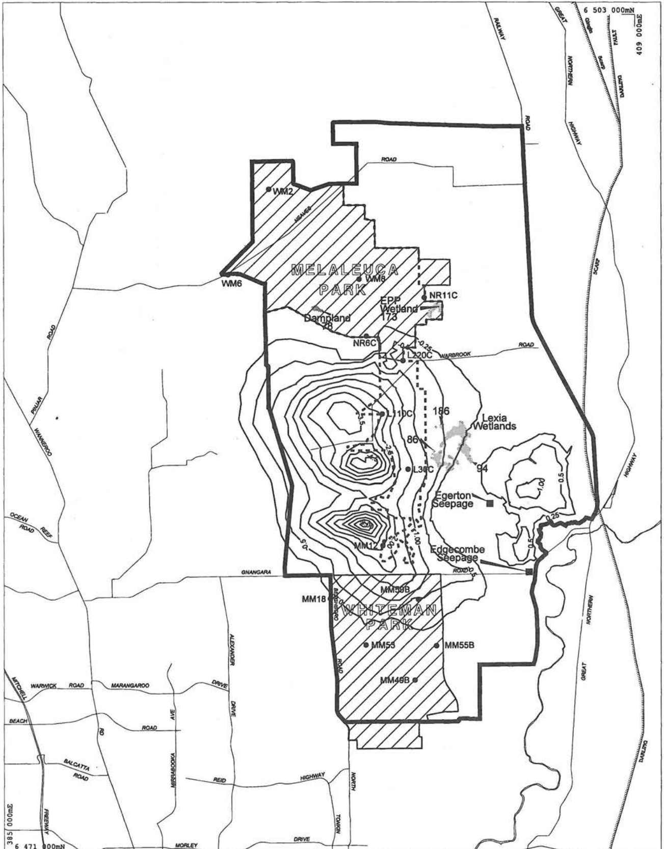
FIGURE 30 - RUN 7. EAST GNANGARA MOUND. Impact of Groundwater Abstraction on Water Levels.
