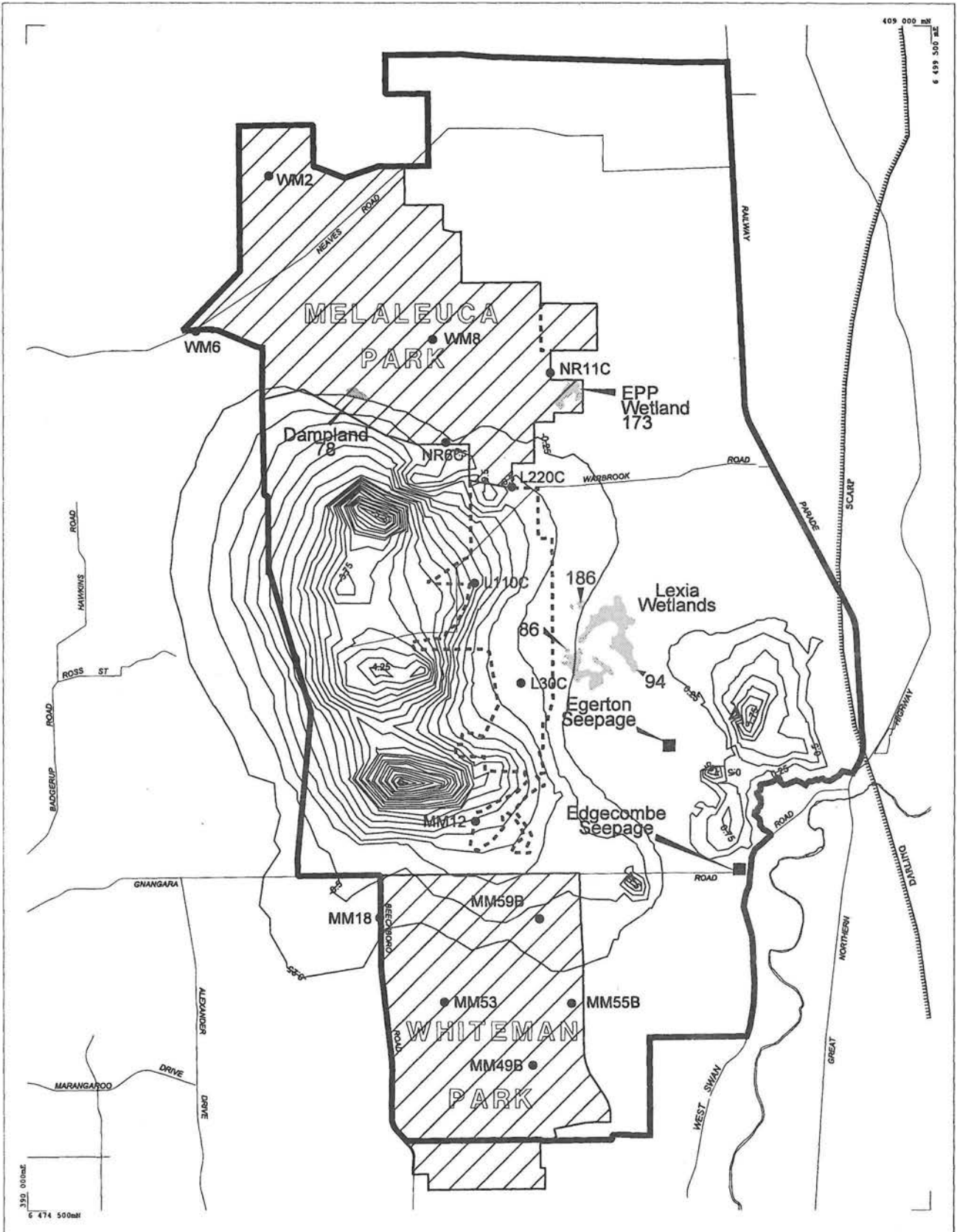
FIGURE E EAST GUNGAHARA MOUND. Impact of Preferred Abstraction and and Land-use Scenario
