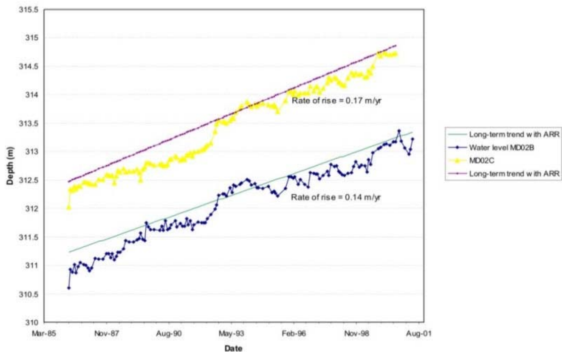
Figure 5. Water levels with accumulative monthly residual rainfall for MD02b and MD02c
