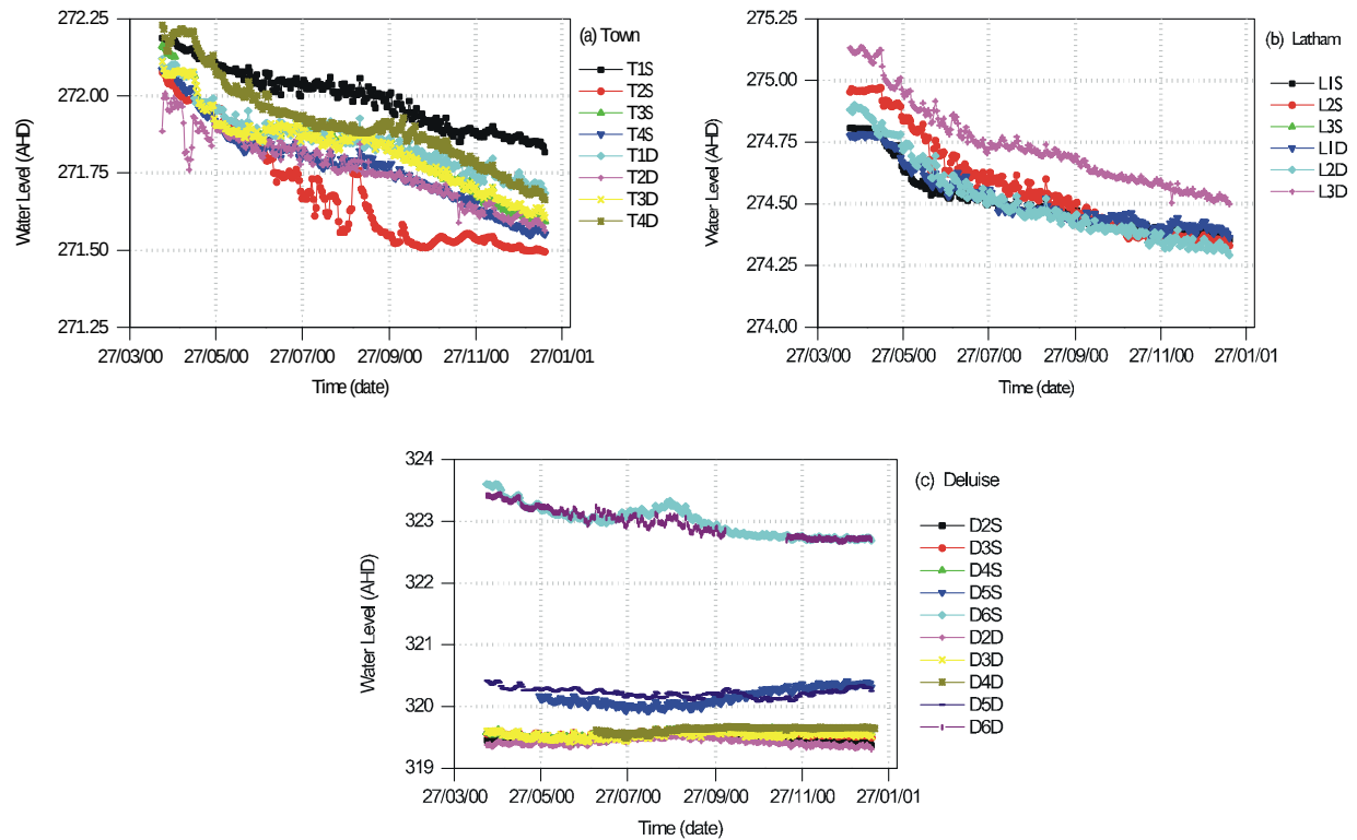
Figure 2: Temporal variation of water levels in shallow and deep piezometers at (a) town, (b) Latham and (c) Deluise sites (Wakeman sub-catchment, Narembreen).
