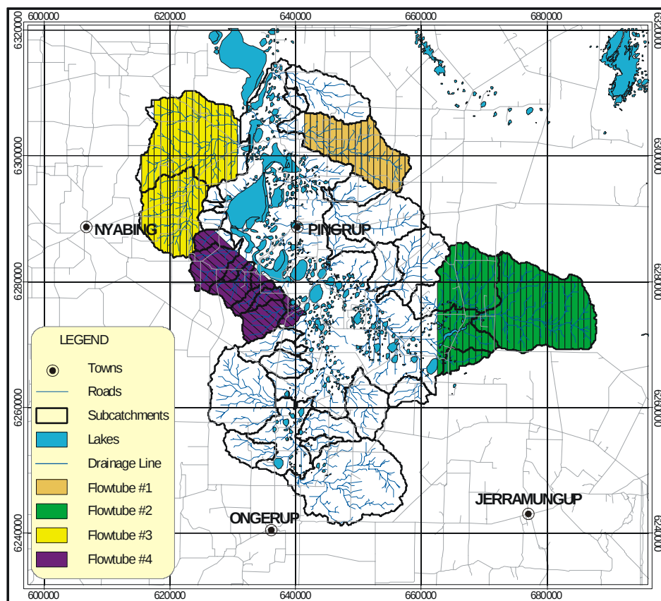
Figure 4: Modelled sub-catchments
