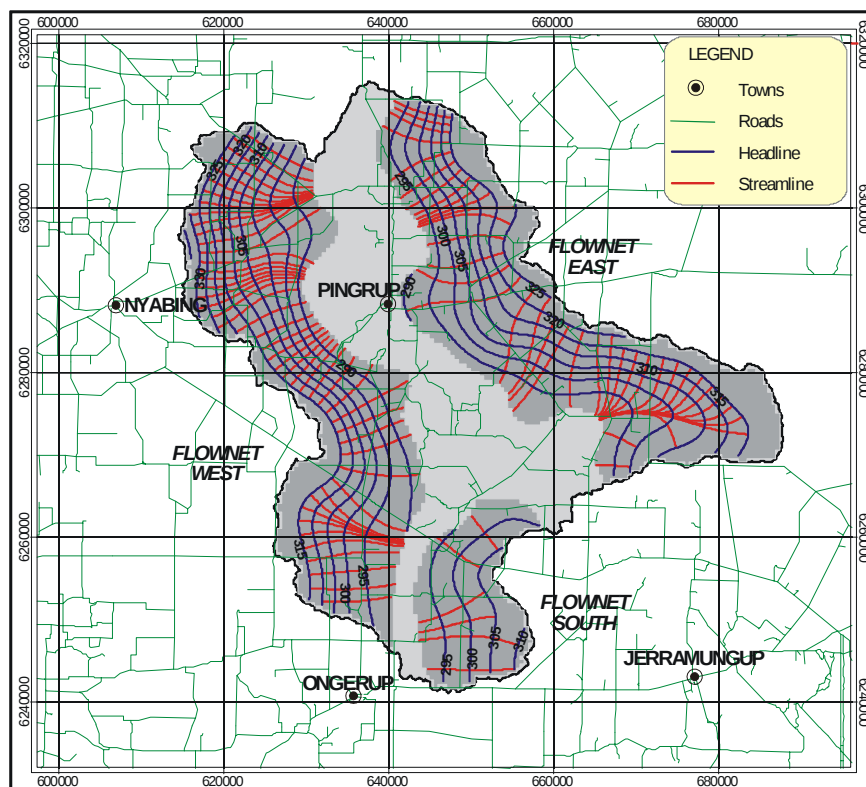
Figure 3: Groundwater Flownet
