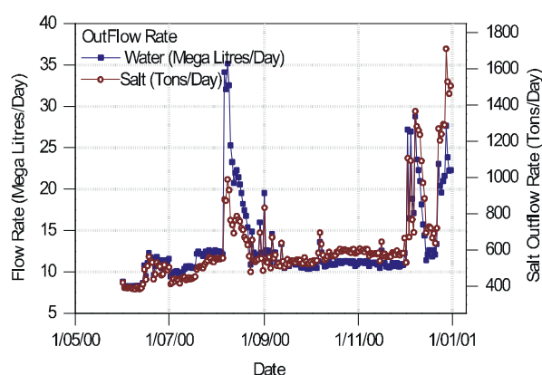
Figure 5: Temporal variation of flow and salt outflow from a main drain in the town of Narembreen (Wakeman sub-catchment)
