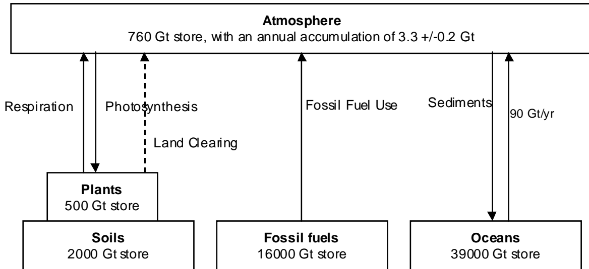
Figure 1. The global carbon cycle (Gt = giga tonnes or 1000 million tonnes). (Source: CRC for Greenhouse Gas Accounting.)
