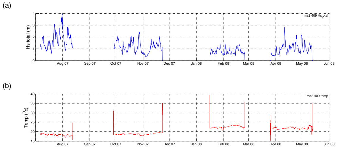
Figure 23 Time-series of (a) significant wave height, and (b) temperature from the SBE26 at site MS2.
