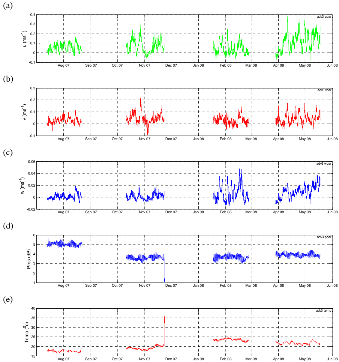
Figure 8 Burst averaged time series from ADV3. (a) eastward, (b) northward, and (c) vertical velocity components, (d) depth and (e) temperature.
