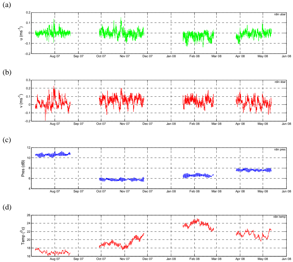
Figure 14 Time series from RDIN. (a) depth-averaged u (eastward) velocity, (b) depth-averaged v (northward) velocity, (c) depth and (d) temperature
