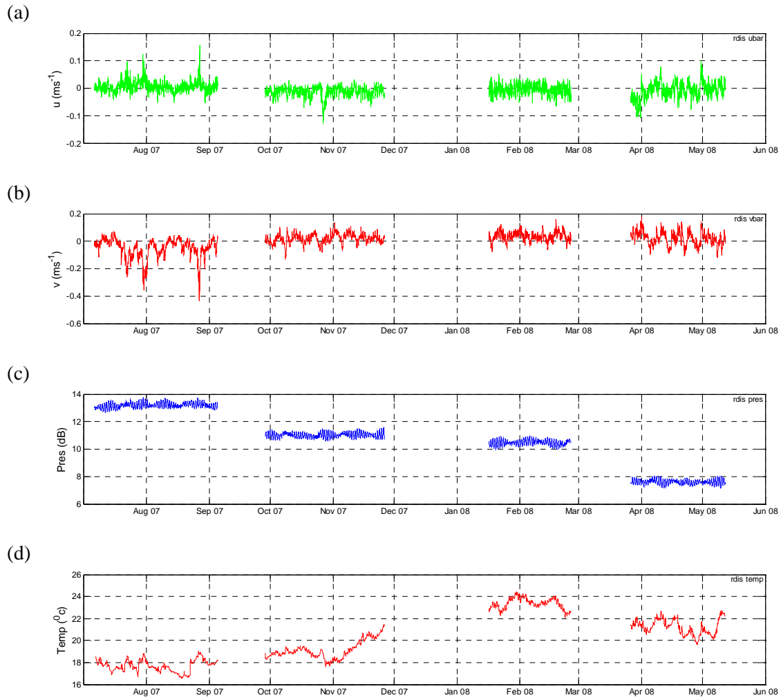
Figure 15 Time series from RDIS. (a) depth-averaged u (eastward) velocity, (b) depth-averaged v (northward) velocity, (c) depth and (d) temperature
