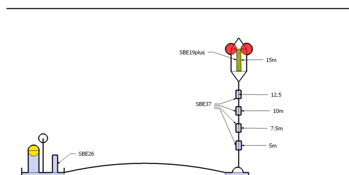
Figure 20 Schematic of mooring at MS2
