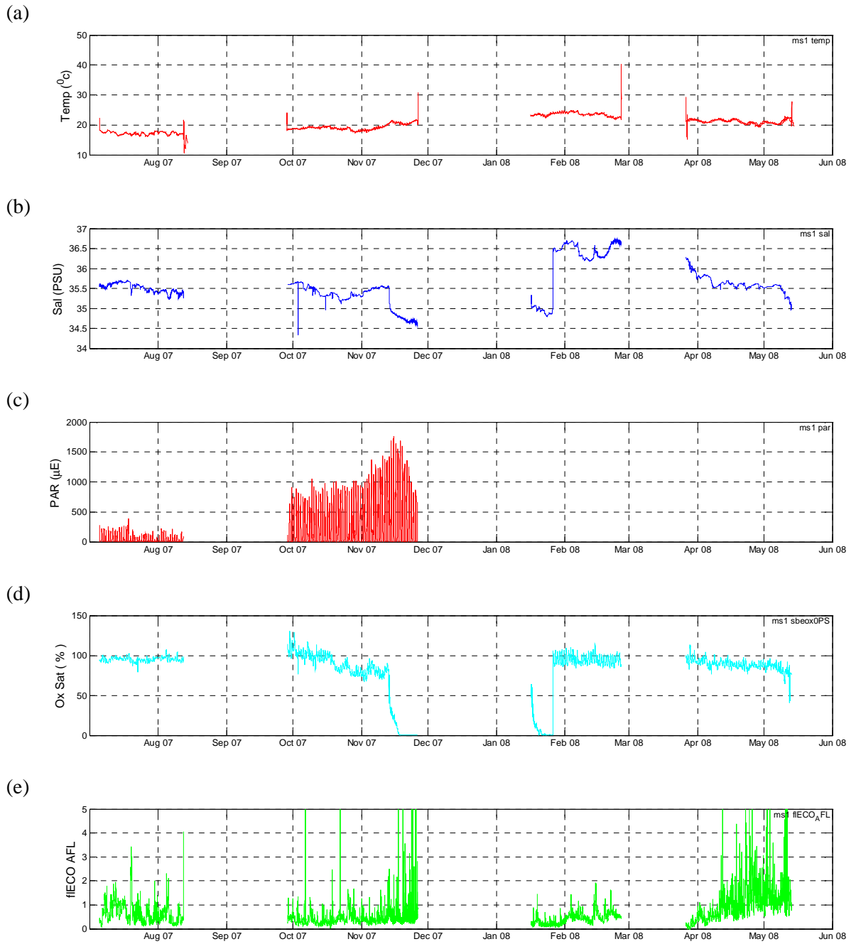
Figure 17 Time-series from SBE19plus at site MS1, (a) temperature, (b) salinity, (c) PAR, (d) oxygen, (e) fluorescence
