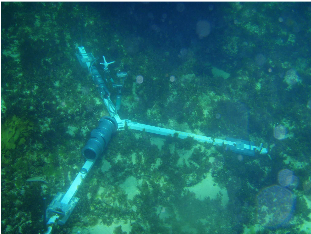
Figure 5 ADV mooring frame
