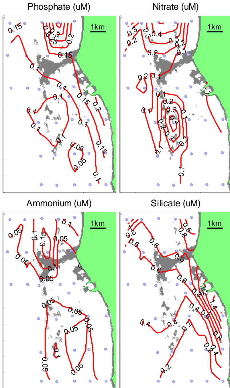
Figure 39 LI200801 surface nutrient distributions.
