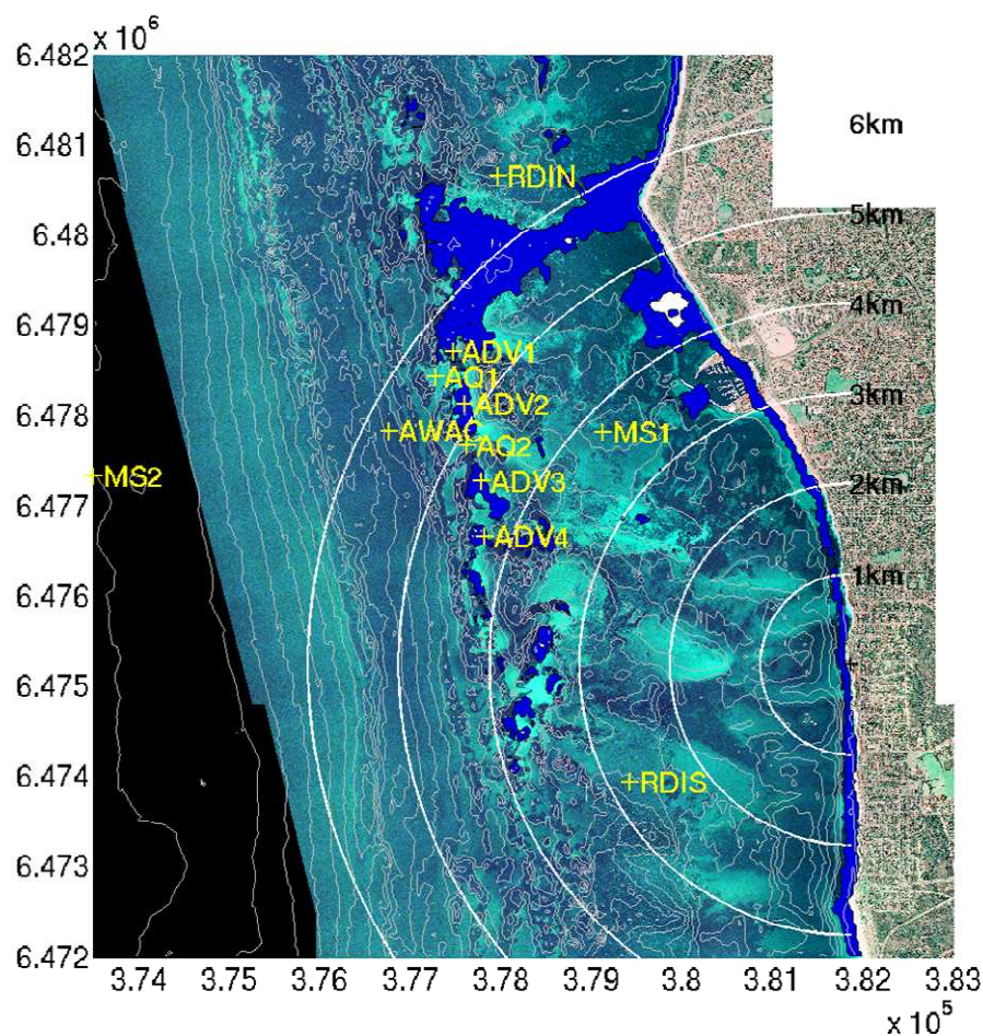
Figure 2 Marmion lagoon showing instrument sites. The filled blue areas denote depths less than 4m. (Aerial photograph courtesy of Oceanica )
