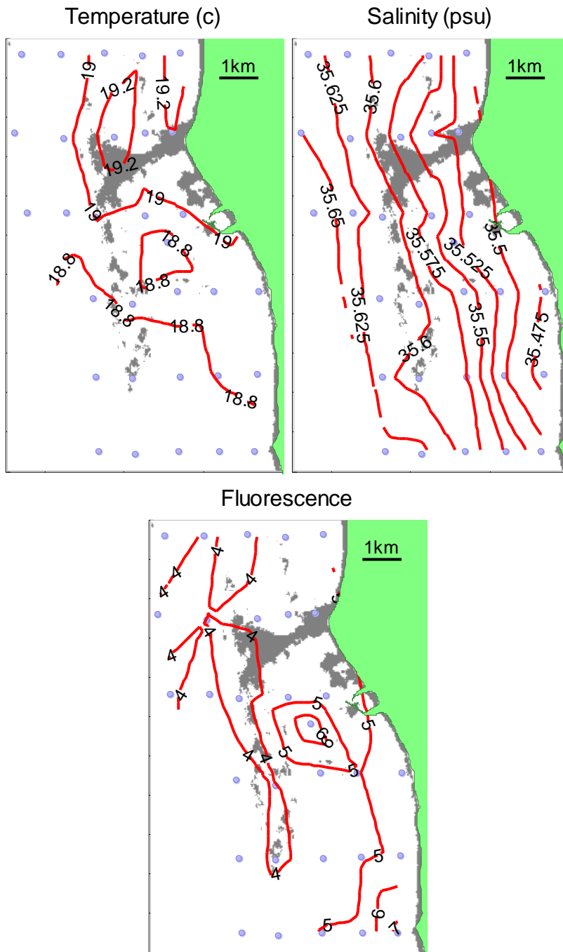
Figure 34 LI200718 surface (2m) temperature, salinity and fluorescence.
