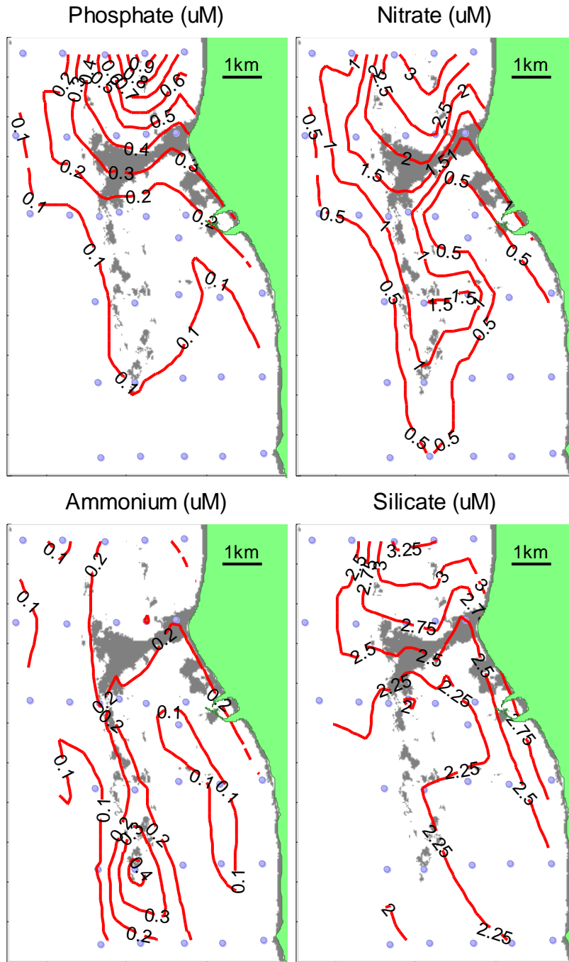
Figure 49 LI200852 surface nutrient distributions.
