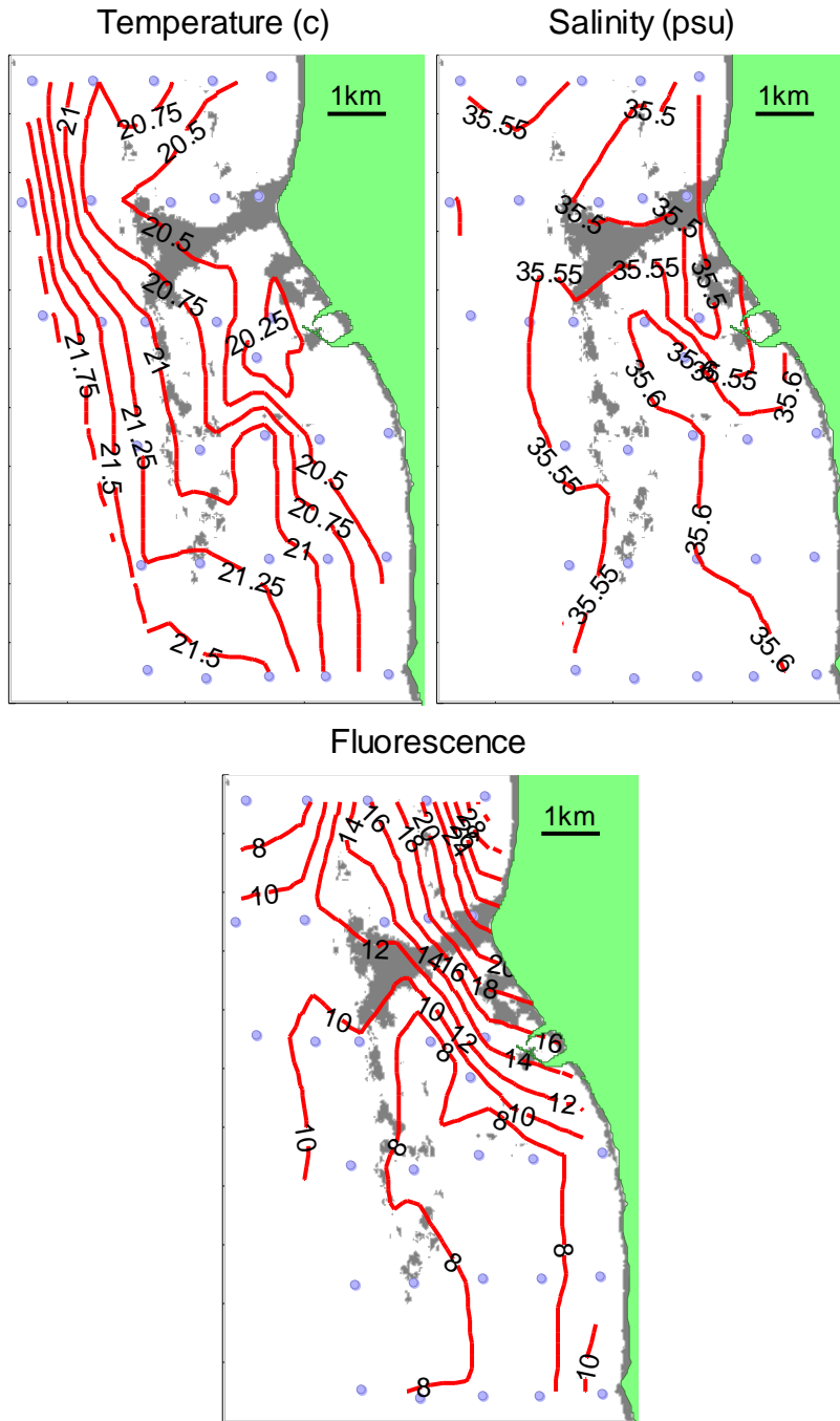
Figure 46 LI200845 surface (2m) temperature, salinity and fluorescence.
