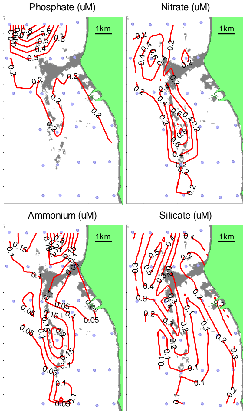
Figure 41 LI200811 surface nutrient distributions.
