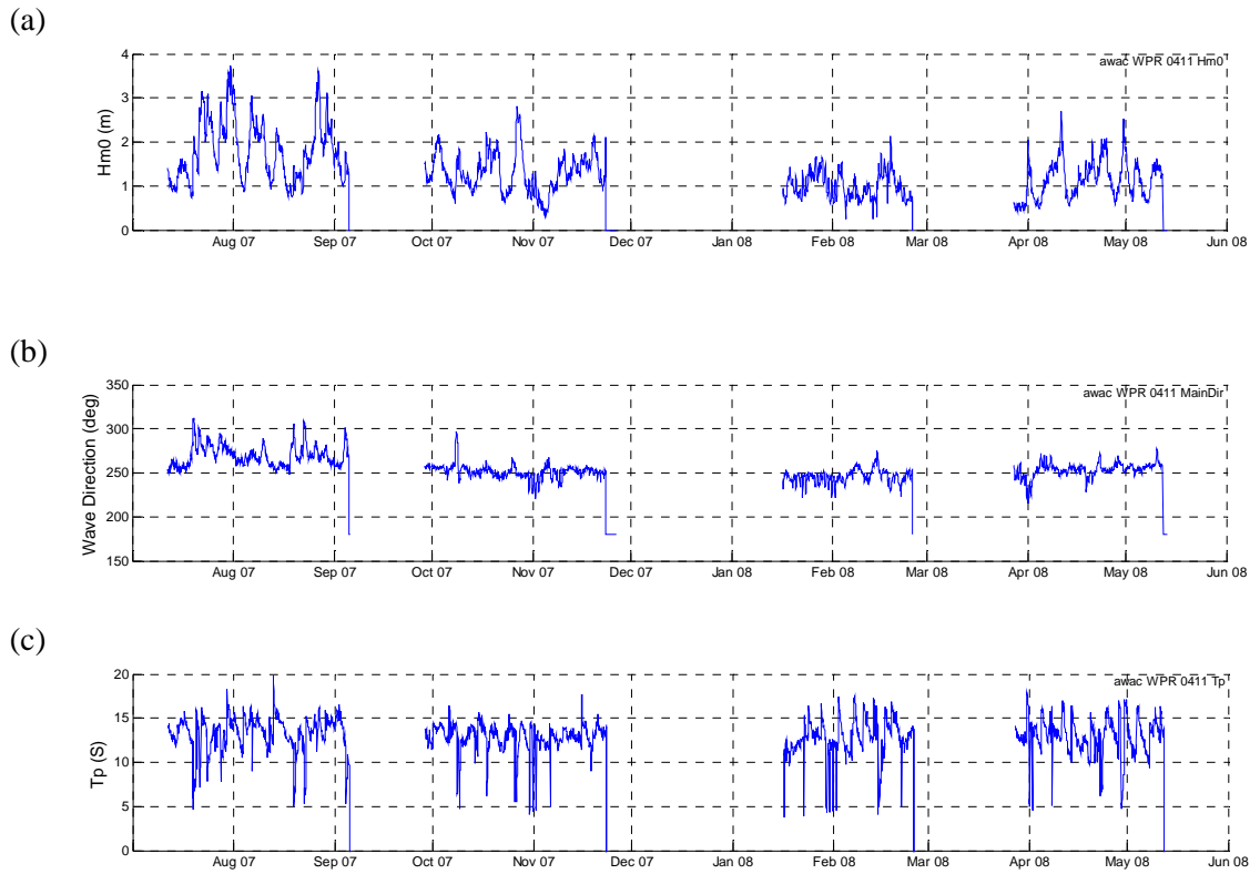
Figure 4 Time series at AWAC, (a) Significant wave height, (b) wave direction, and (c) wave period.
