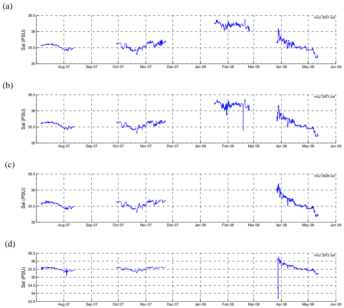
Figure 25 Time-series of salinity measured by the SBE37's at MS2, with (a) being the shallowest and (d) being the deepest. The sensor depths are plotted in Figure 26.
