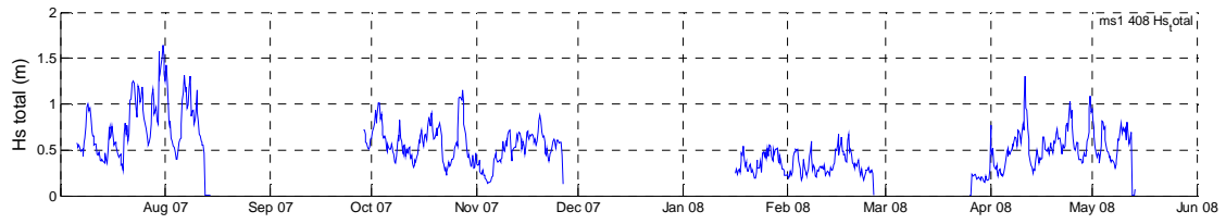
Figure 18 Time-series of significant wave height from SBE26 at site MS1.
