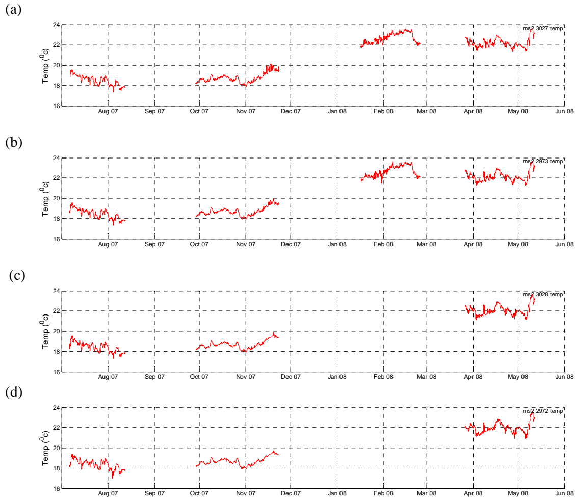
Figure 24 Time-series of temperatures measured by the SBE37's at MS2, with (a) being the shallowest and (d) being the deepest. The sensor depths are plotted in Figure 26.
