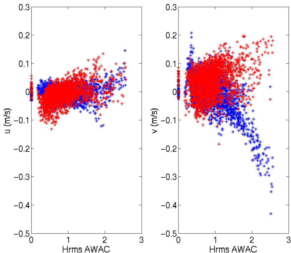
Figure 51 Mean eastward (left panel) and northward (right panel) currents at RDIN (red) and RDIS (blue).
