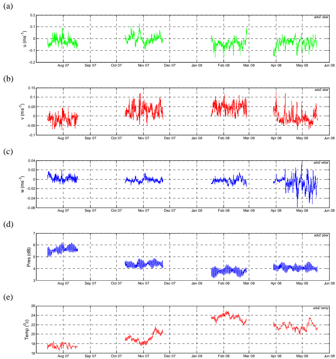
Figure 7 Burst averaged time series from ADV2. (a) eastward, (b) northward, and (c) vertical velocity components, (d) depth and (e) temperature.
