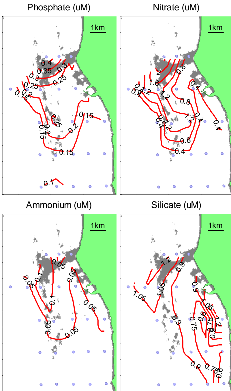
Figure 29 LH01 surface nutrient distributions.
