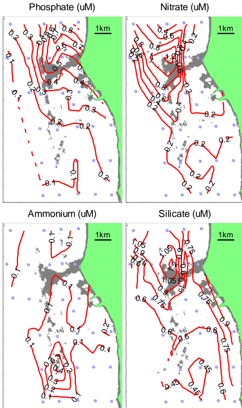
Figure 33 LI200712 surface nutrient distributions.
