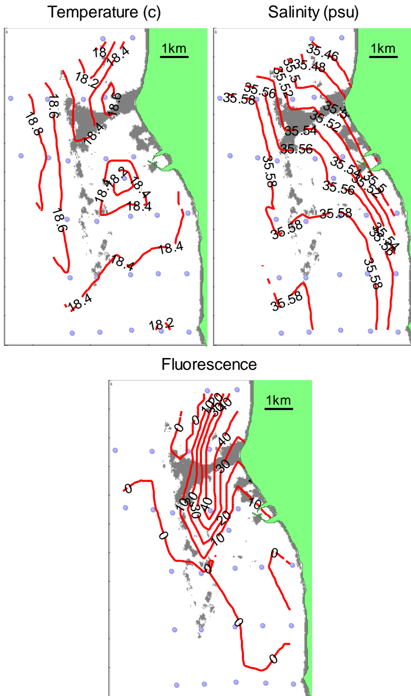
Figure 32 LI200712 surface (2m) temperature, salinity and fluorescence.
