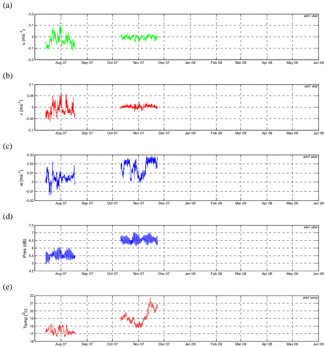
Figure 6 Burst averaged time series from ADV1. (a) eastward, (b) northward, and (c) vertical velocity components, (d) depth and (e) temperature.
