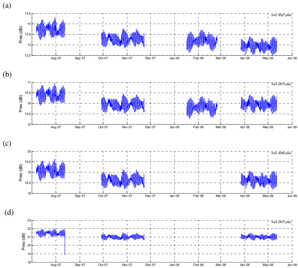
Figure 26 Time-series of depth measured by the SBE37's at MS2, with (a) being the shallowest and (d) being the deepest.
