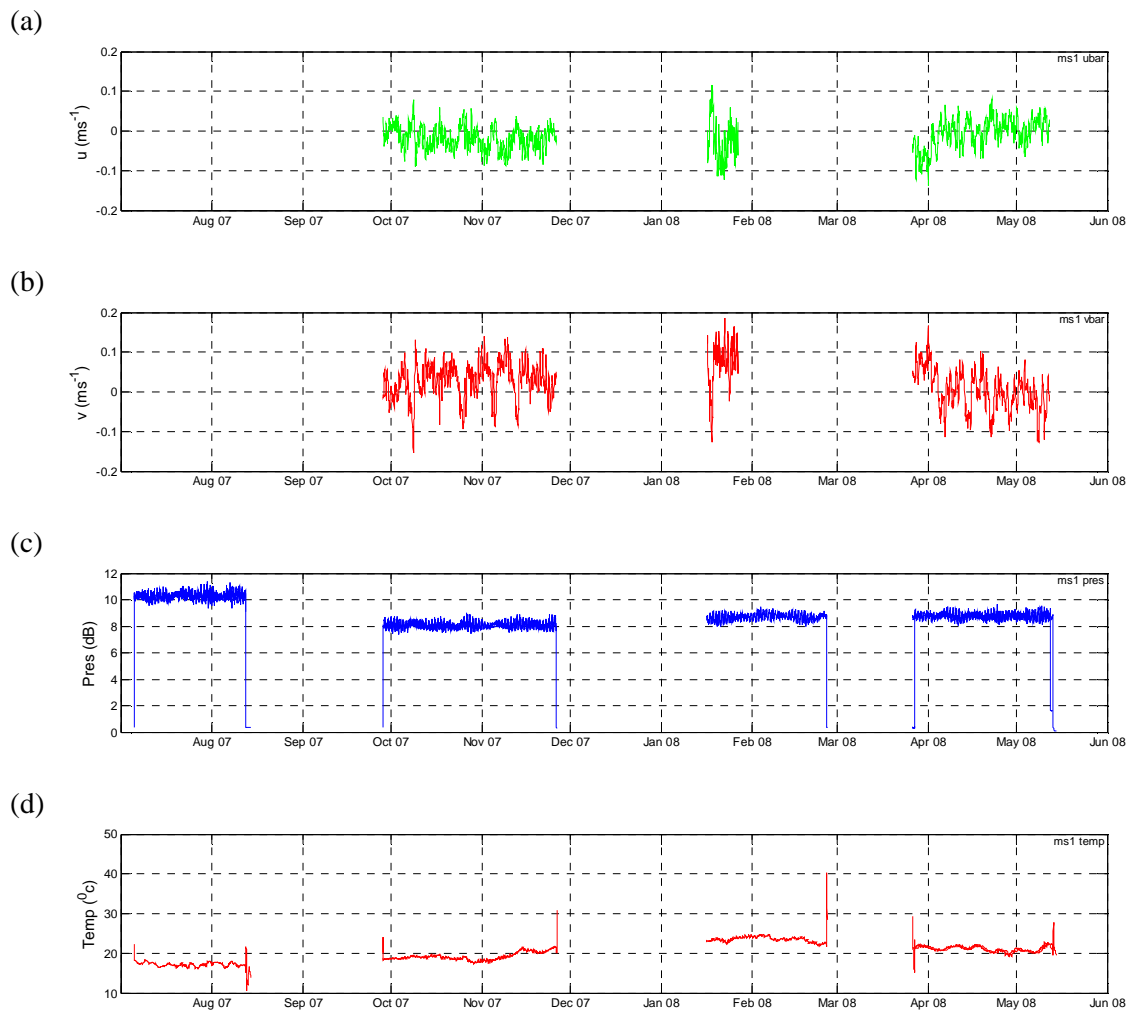
Figure 19 Time-series from rdi adcp at MS1. (a) depth-averaged u (eastward) velocity, (b) depth-averaged v (northward) velocity, (c) depth and (d) temperature
