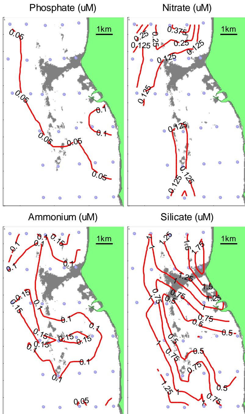
Figure 43 LI200830 surface nutrient distributions.
