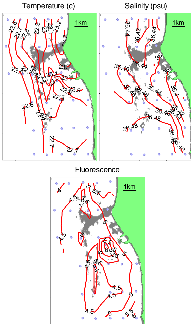
Figure 38 LI200801 surface (2m) temperature, salinity and fluorescence.
