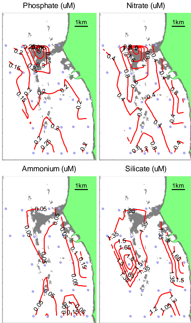
Figure 31 LI200710 surface nutrient distributions.
