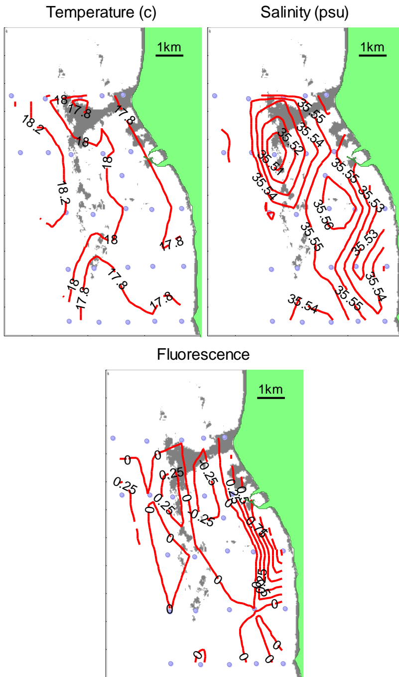
Figure 30 LI200710 surface (2m) temperature, salinity and fluorescence.
