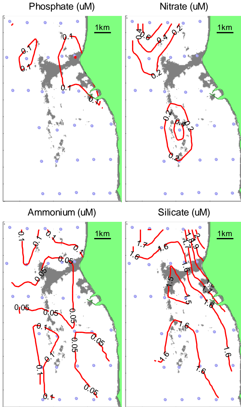
Figure 45 LI200836 surface nutrient distributions.
