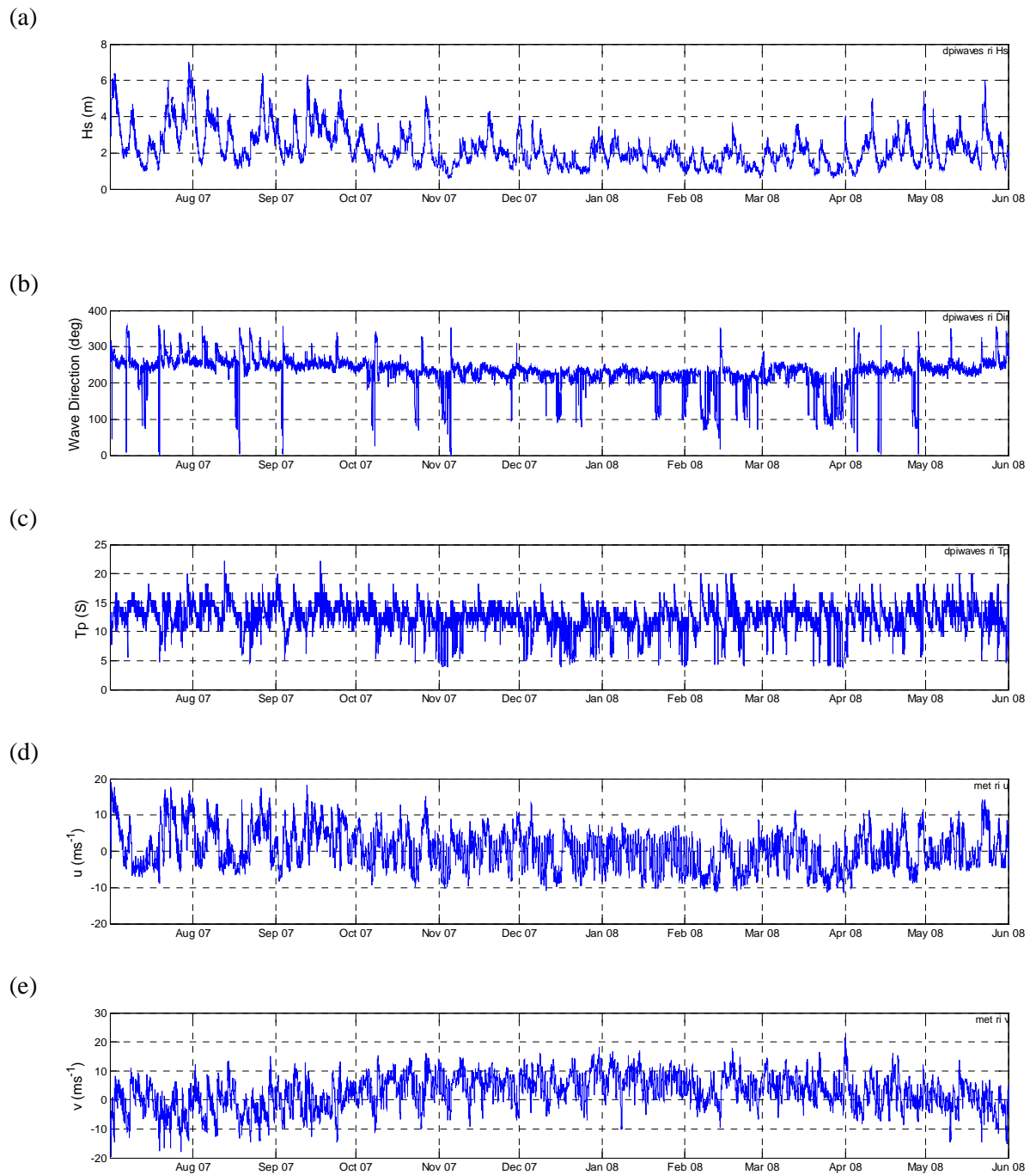
Figure 1 Time series from the Rottneest wave buoy ( 32^{\circ} 05'39''\text{S} 115^{\circ}24'28''\text{E} ); (a) significant wave height, (b) direction and (c) peak period. Panels (d) and (e) are the eastward and northward components respectively of wind measured at Rottneest.
