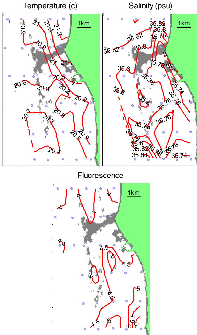
Figure 36 LI200724 surface (2m) temperature, salinity and fluorescence.
