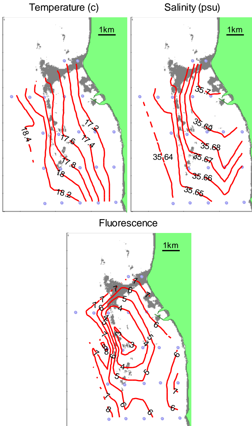
Figure 28 LH01 surface (2m) temperature, salinity and fluorescence.
