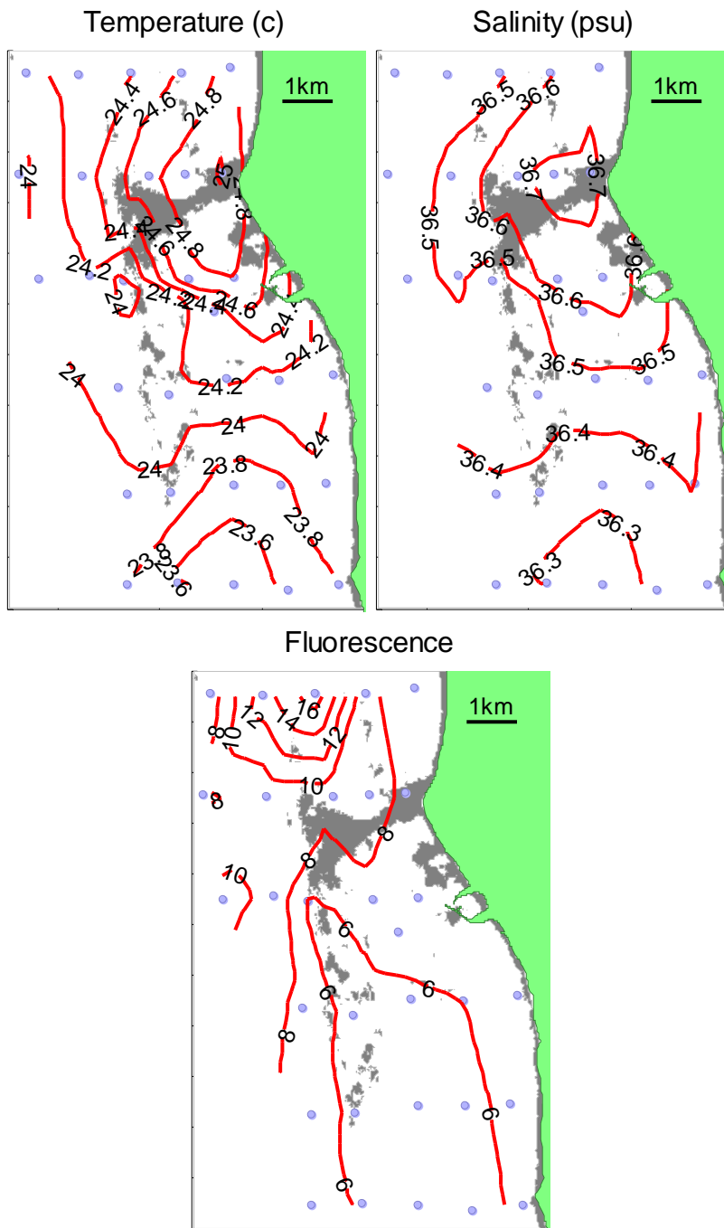
Figure 40 LI200811 surface (2m) temperature, salinity and fluorescence.
