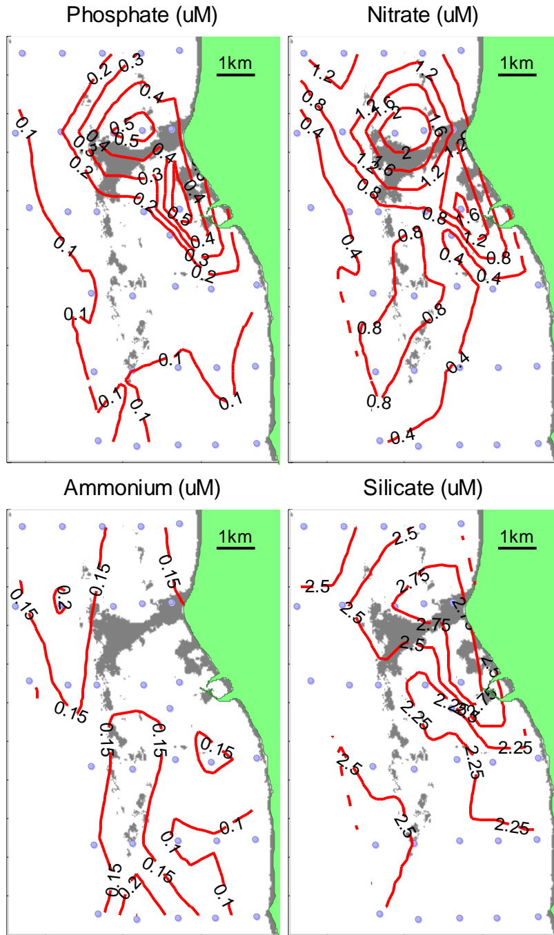
Figure 47 LI200845 surface nutrient distributions.
