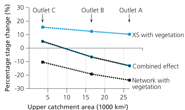
Figure 5.10. a) and b) Stage hydrographs at Wagga Wagga comparing the relative importance of local and upstream vegetation condition. c) Percentage stage change at Wagga Wagga (Outlet A) for a given event size. d) Percentage stage change down the catchment (from outlet C to A) with the addition of riparian vegetation.
