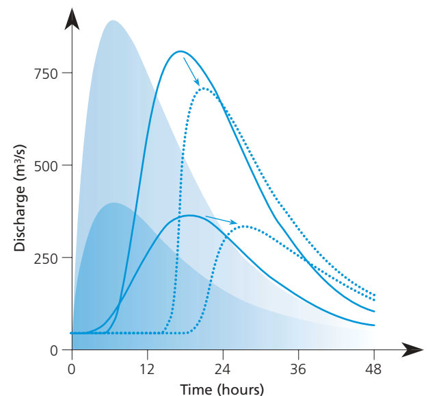
Flood waves @ 50 km — Channel with no vegetation ..... Channel with vegetation → Change in peak Input flood waves Light blue Large flood Dark blue Moderate flood
