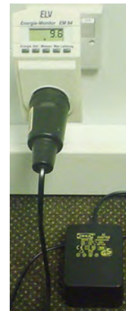
Figure 22.1. An awful AC lamp-adaptor from IKEA – the adaptor uses nearly 10 W even when the lamp is switched off!
