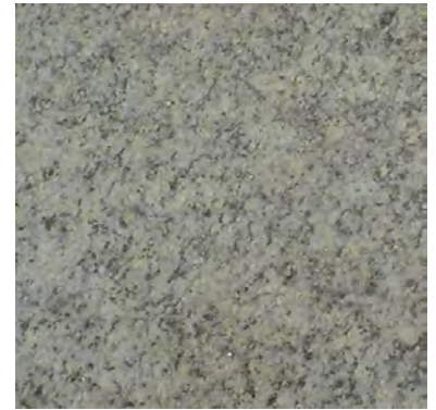
Figure 16.2. Some granite.
