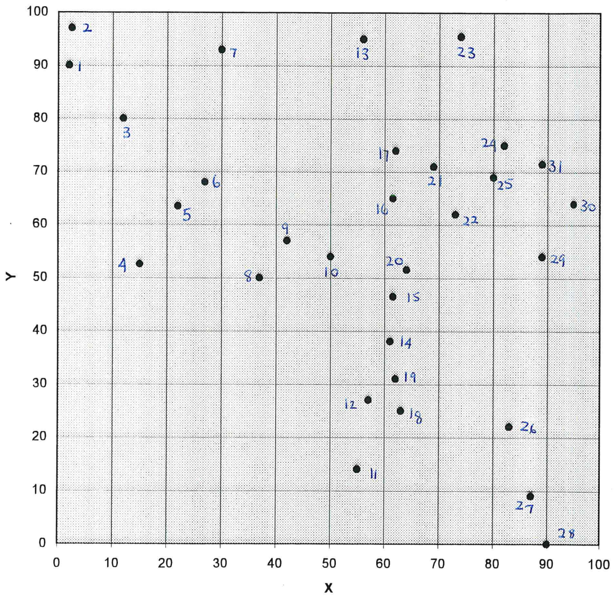
Figure YD6 Location of Melaleuca uncinata Site 5 Yellowdine
