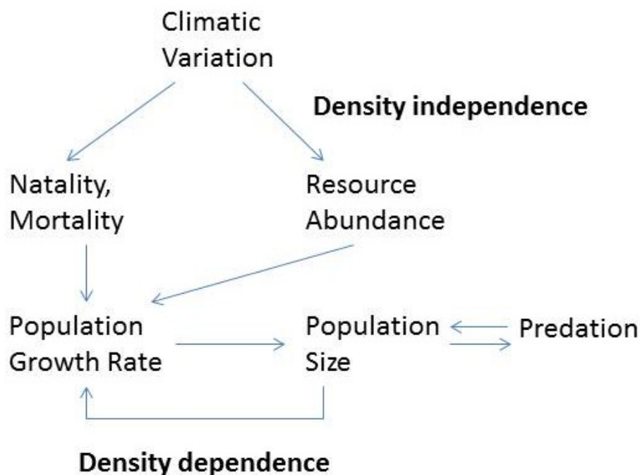
FIGURE 3-1 Population processes, including density-independent and density-dependent controls.
