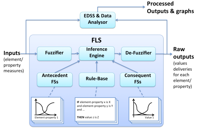
Fig. 1. The architecture of the developed FLS
