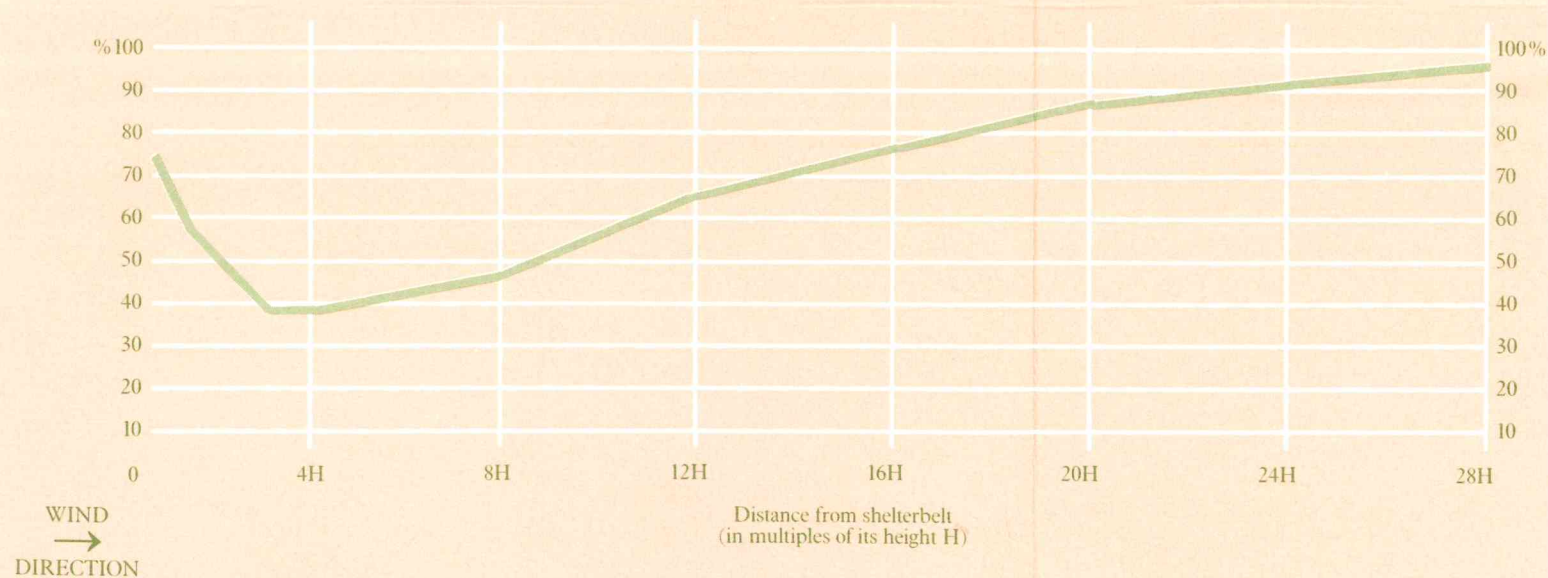
FIGURE 1 WINDSPEED BEHIND A SHELTERBELT (EXPRESSED AS A PERCENTAGE OF UNCONTROLLED WINDSPEED)
