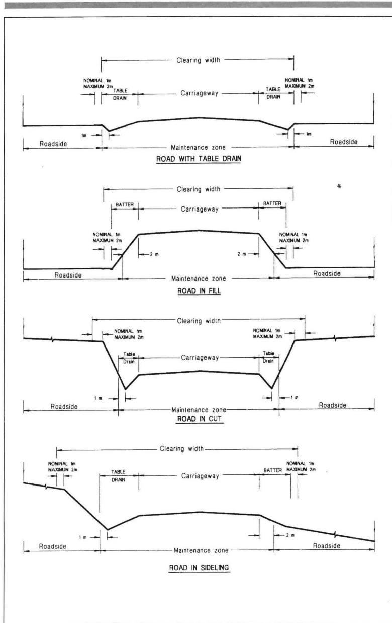
Typical road reserve cross sections
