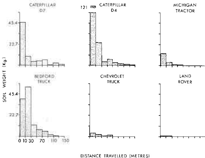
Figure 6 Soil Weight dropped from Mobile Machinery.
