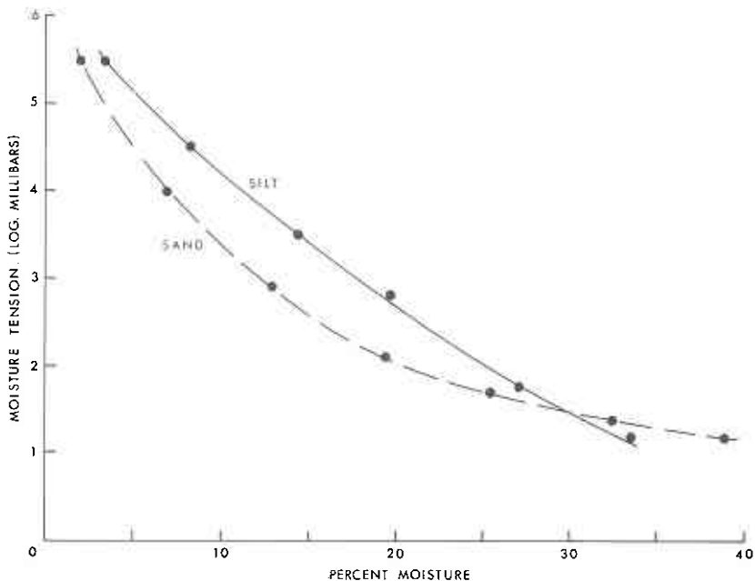
Figure 9 Characteristic moisture curves of silt from dieback gully and humisoid-sand from dieback swamp.
