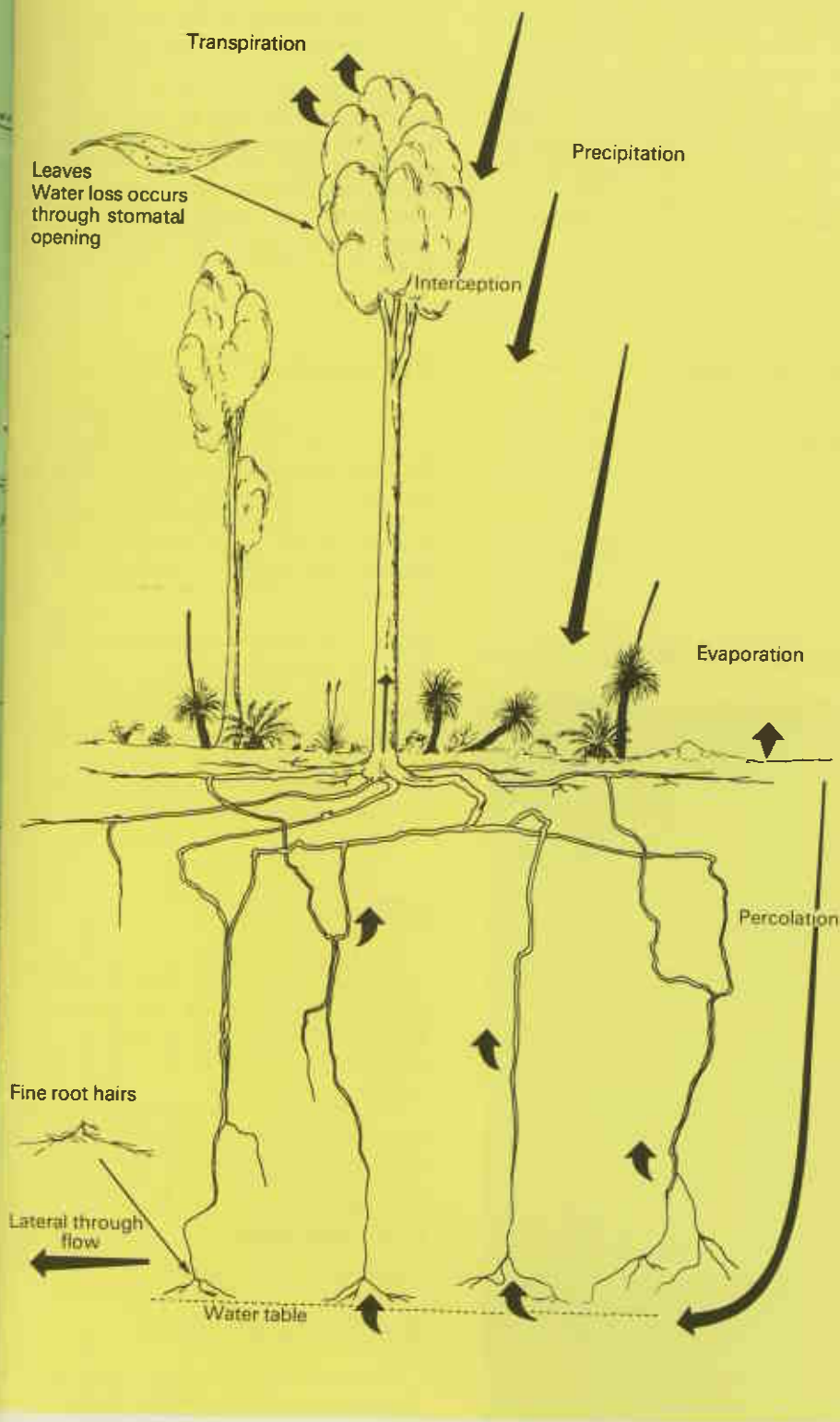
▲ Diagrammatic representation of the hydrological cycle.
