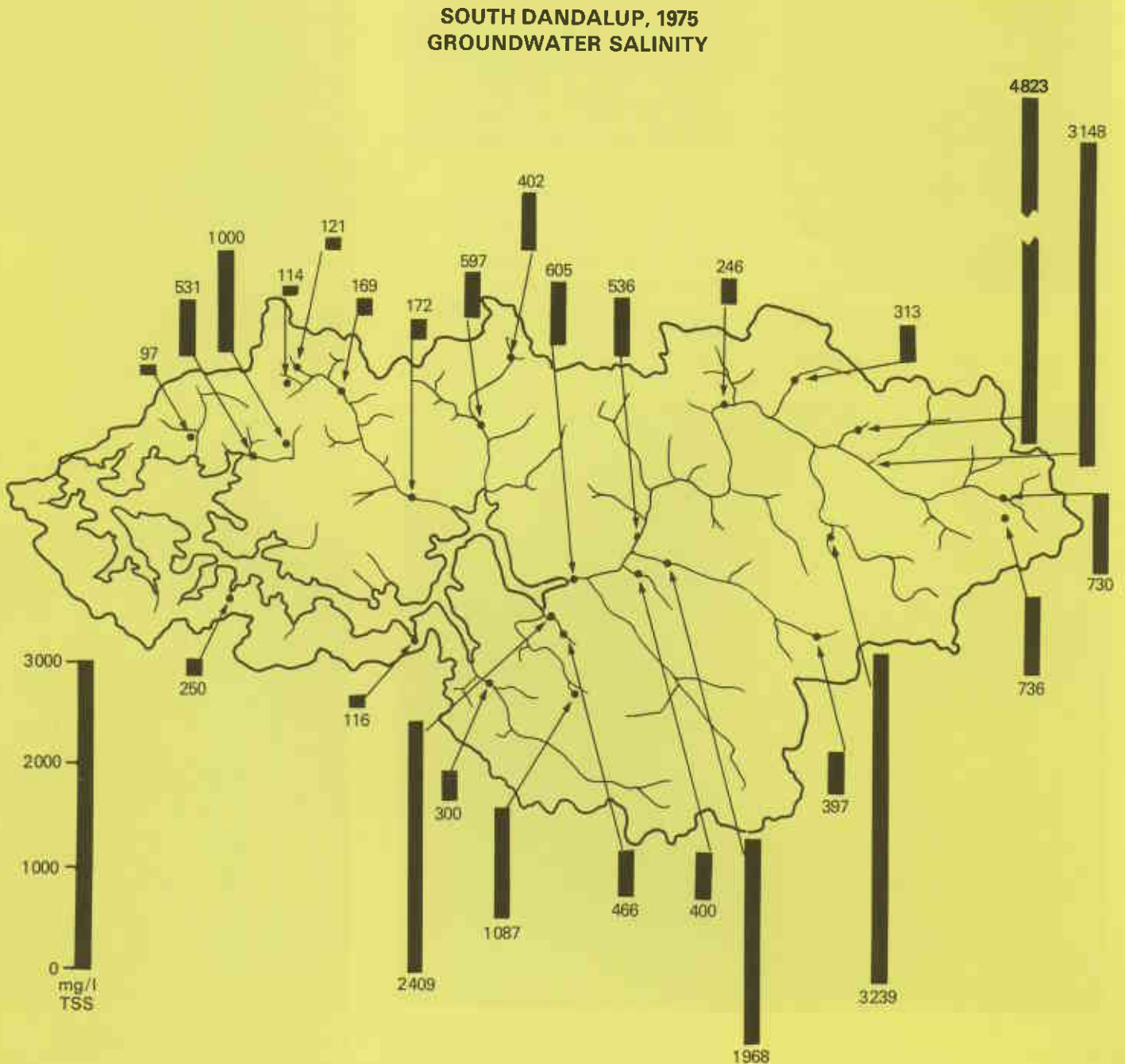
▼ South Dandalup catchment estimated groundwater salinity levels.
