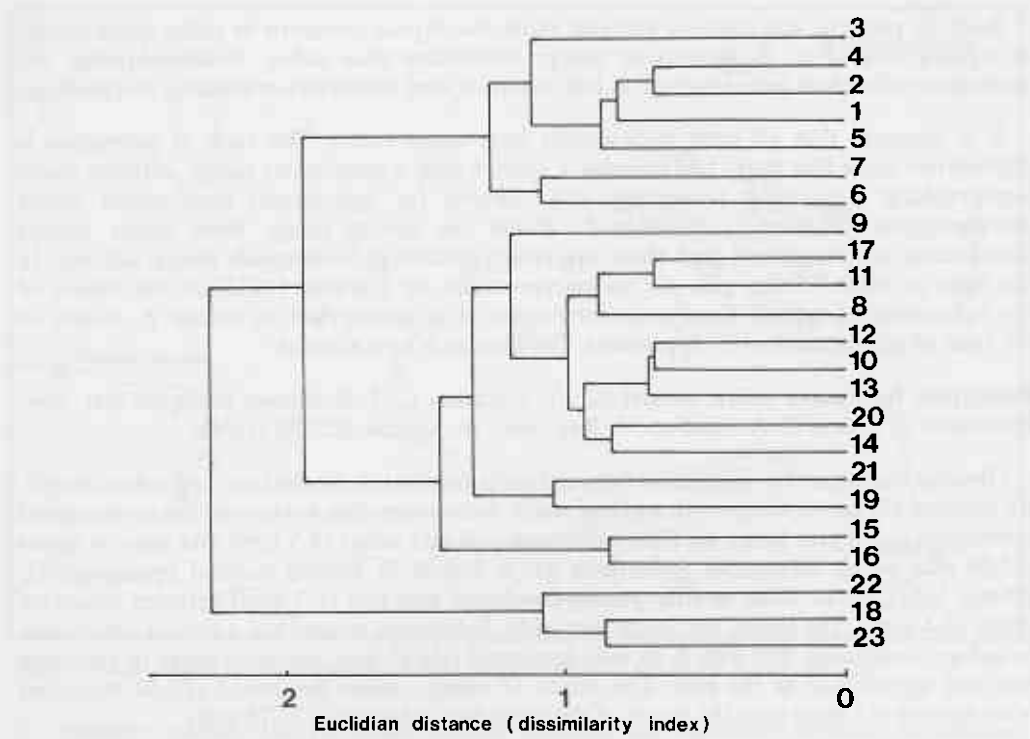
Figure 2. Phenogram of the numbered populations of Eucalyptus forrestiana s. lat.
