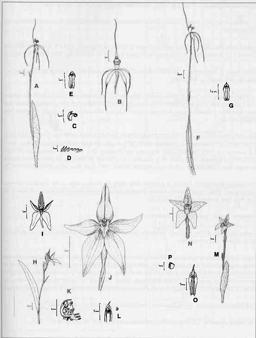
Figure 30. A-E. Caladenia uliginosa subsp. uliginosa from the Kojonup area, A.P. Brown 260. A - plant; B - flower from front; C - labellum and column from side; D - labellum fringe; E - column from front. F, G. C. uliginosa subsp. candicans from the Dale area, S.D. Hopper 5639. F - plant; G - column from front; H-L. C. flava subsp. flava from Wandering, A.P. Brown s.n. H - plant; I - flower from front; J - flower from front, enlarged view; K - labellum and column; L - column from front. M-P. C. flava subsp. maculata from the Kalbarri area, S.D. Hopper 6308. M - plant; N - flower from front; O - column from front; P - pollinia. Drawn by S.J. Patrick.
