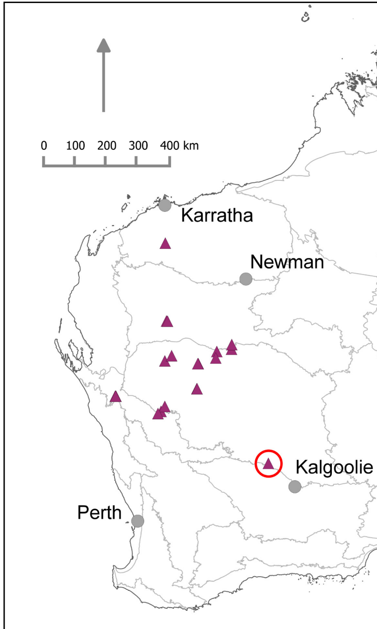
Figure 3. Distribution of Goodenia berringbinensis showing the disjunction between the main distribution and the more south-eastern population at the Ularring wetland (circled). The IBRA version 6.1 bioregions (Department of Sustainability, Environment, Water, Population and Communities 2004) are shown in grey.
