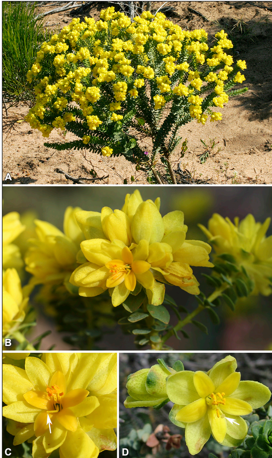
Figure 1. Geleznowia amabilis . A – habit; B – flowering heads with golden yellow bracts and sepals; C – a flower highlighting the long style with a narrow stigma (white arrow) and sepals that are much longer than the petals. Geleznowia verrucosa . D – single flower showing the lemon yellow petals and capitate stigma (white arrow). Images by K.A. Shepherd (A–C) from K.A. Shepherd & J.A. Wege KS 1305 and R. Davis (D) from R. Davis RD 11223.
