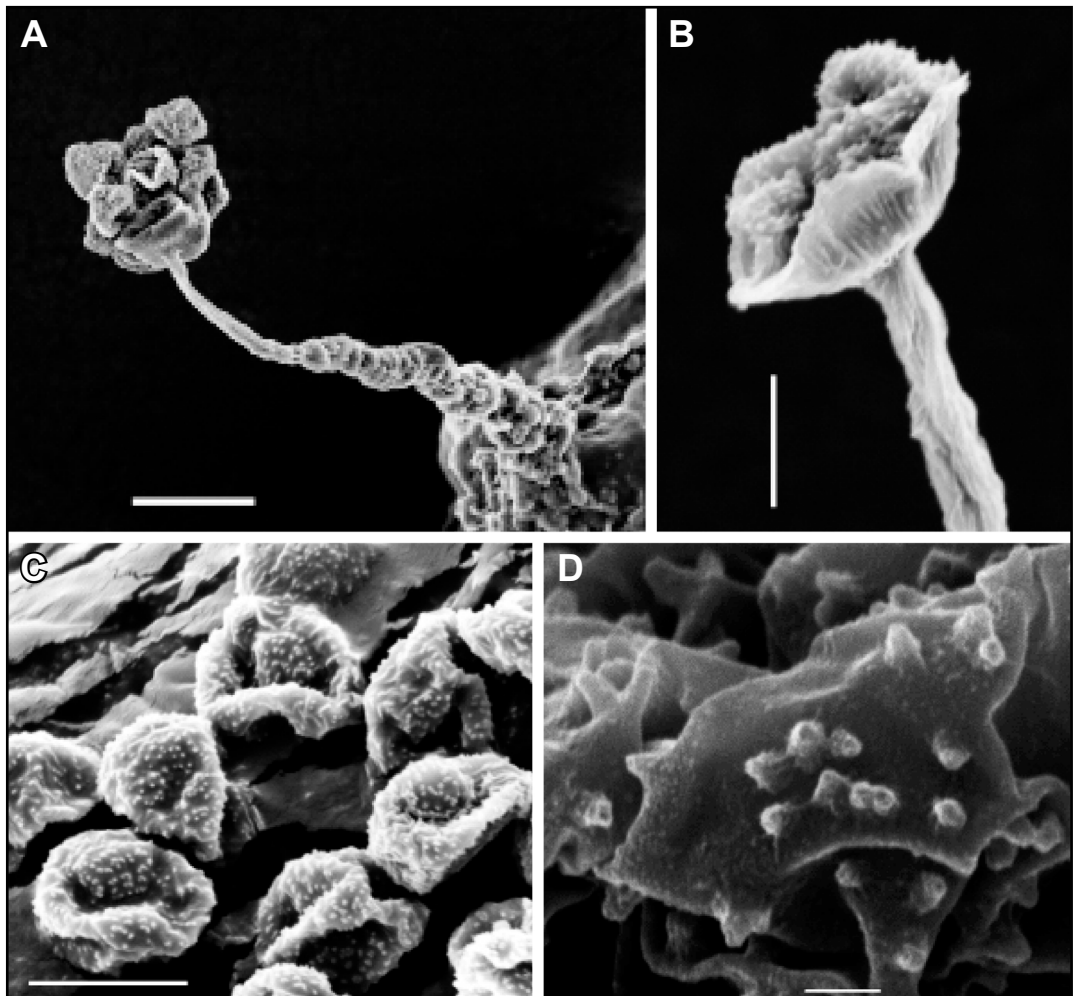
Figure 2. Echinostelium australiense as viewed with scanning electron microscopy. A – sporocarp showing the tapering stalk, rough below and a large peridial collar; B – large minutely striate petaloid collar showing the minutely widely stellate or roughened, somewhat thickened and recurved edge; C – collapsed spores showing sparsely warted ornamentation between the rather discreet, approximately circular darker patching with the warts arranged in clusters, lines or joined; D – spore ornamentation formed by rounded or flat topped warts and when clustered with minute ridges between the warts. Images from K.J. Knight MC 284 (B); MC 285 (A, C); MC 286 (D). Photographs by Steve Dillon (A-C) and Yuri Novozhilov (D). Scale bars: 20 \mu\text{m} (A); 5 \mu\text{m} (B); 10 \mu\text{m} (C); 0.5 \mu\text{m} (D).
