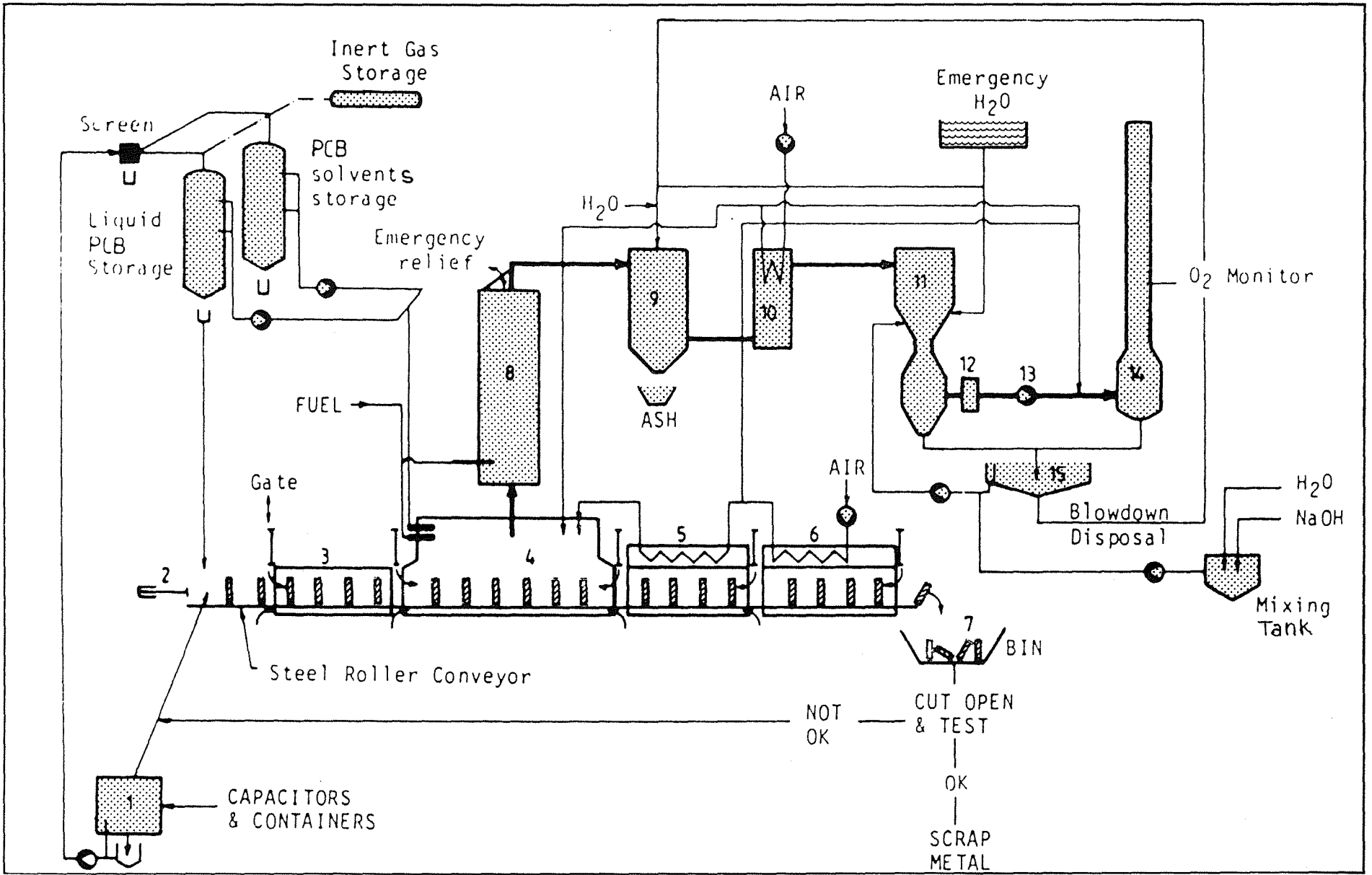
Figure 2. Simplified Process Diagram of the Incinerator. (Source: PER)
