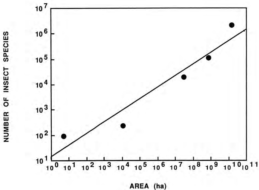
Figure 6. Relationships between number of insect species and area for various localities. Least-squares best-fit equation is \log Y = 1.15 + 0.46 \log X , with r^2 = 0.92 .
