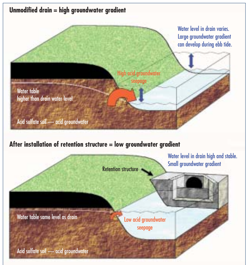
Figure 3: These diagrams demonstrate the principle of reducing groundwater gradients by keeping drain water levels high and stable using a retention structure. This helps contain acid groundwater in the landscape and reduce acid export to rivers. Diagrams Scott Johnston
